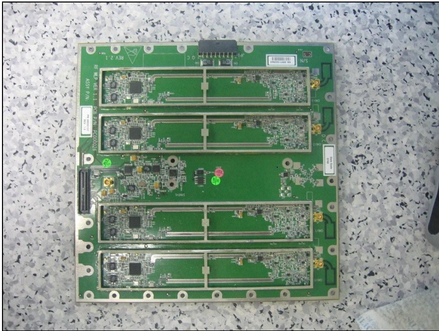
Photograph 10. RF board CS No covers
