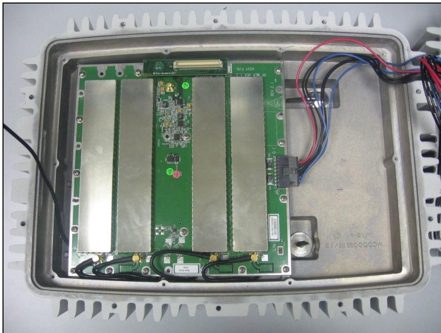
Photograph 12. RF Layer
