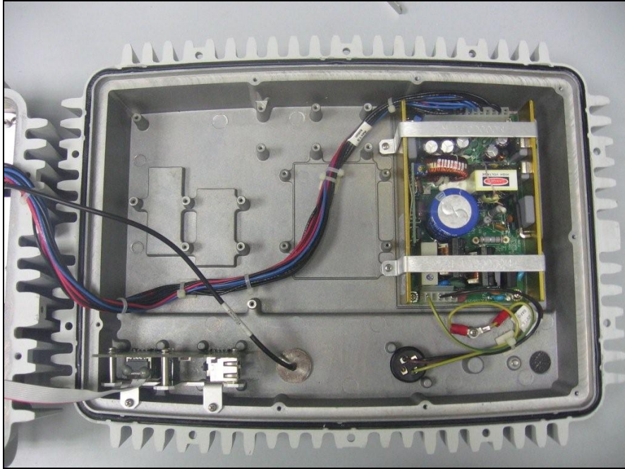
Photograph 9. Power Side
