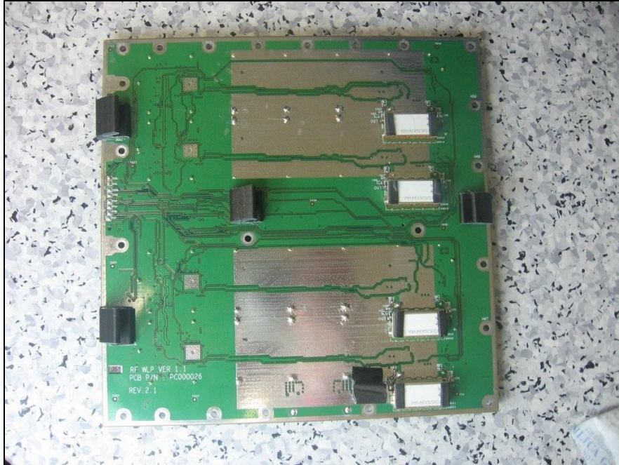
Photograph 11. RF Board PS
