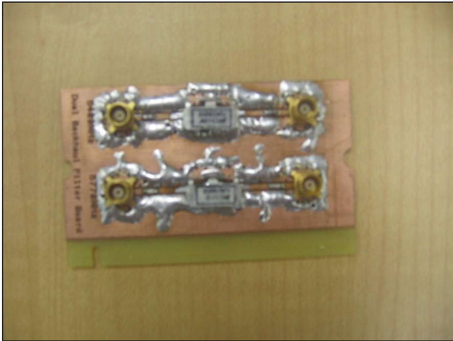
Photograph 6. Filters CS
