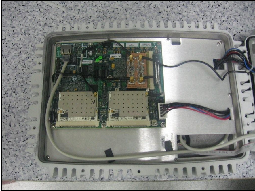
Photograph 3. BB Layer
