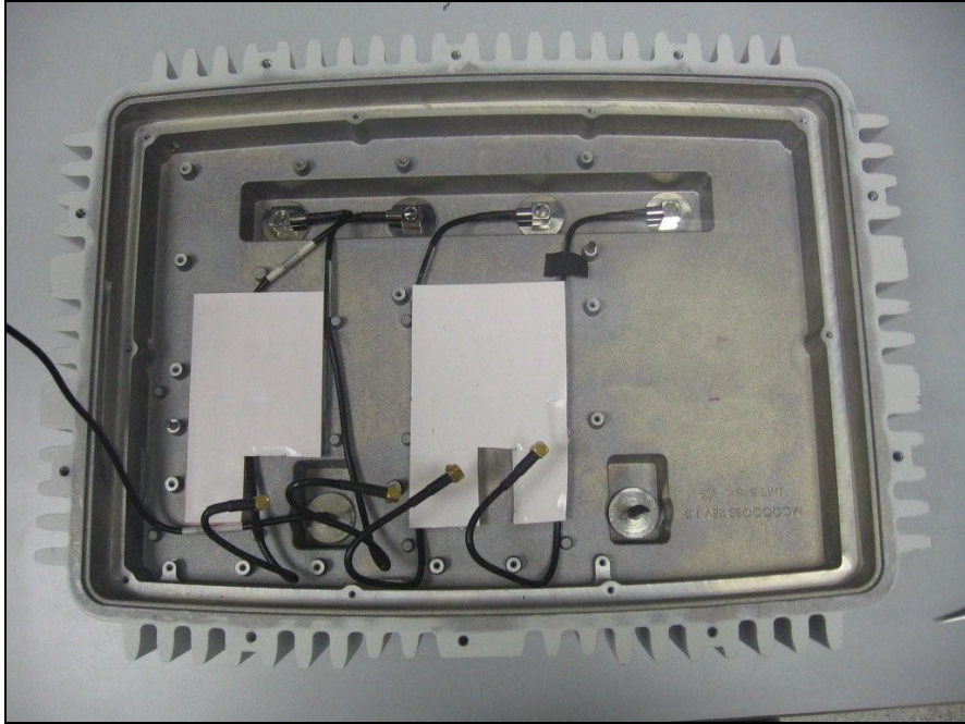
Photograph 5. Bottom Layer
