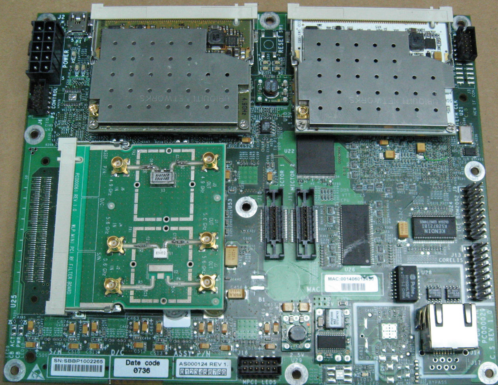
Base Band Board with filter card and Modules
