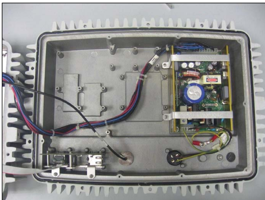
Photograph 8. Power Side
