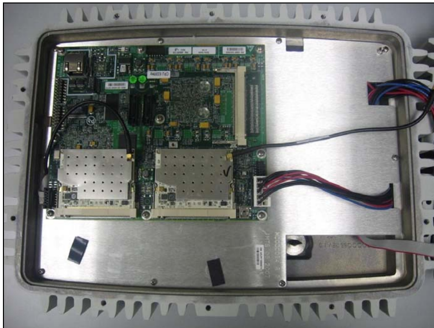
Photograph 4. BB Layer
