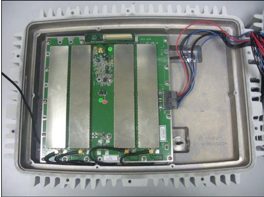
Photograph 11. RF Layer
