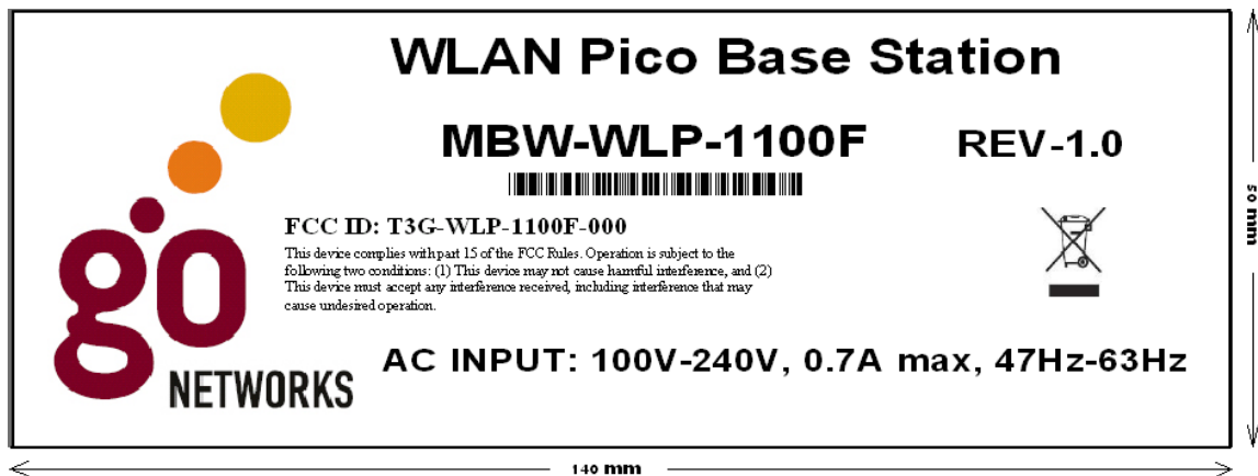
Figure 1. FCC Label
