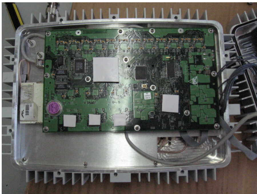
Figure 1 Top Cover With BB Card Internal View
