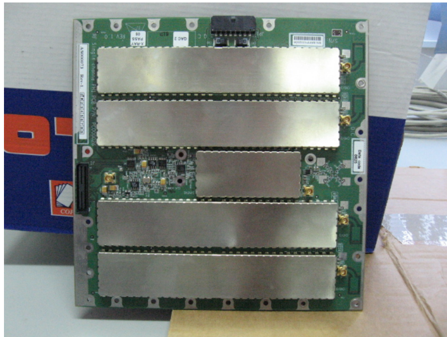
Figure 13 RF Card Component Side With Shield
