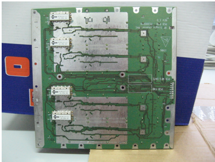
Figure 15 RF Card Print Side
