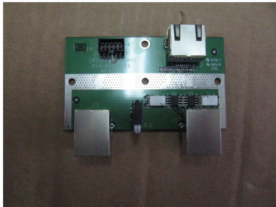
Figure 10 IF Card Top Side
