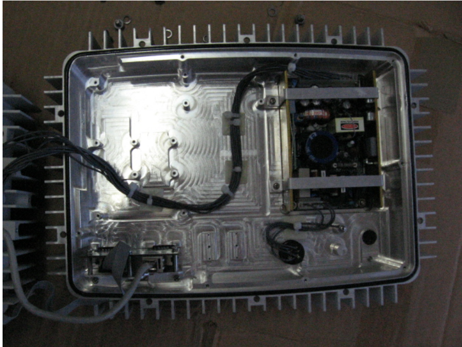
Figure 5 Bottom Cover With IF Card and Power Supply Internal View
