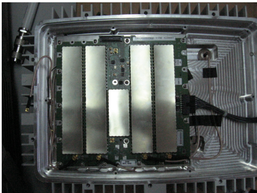
Figure 2 Top Cover With RF Card Internal View
