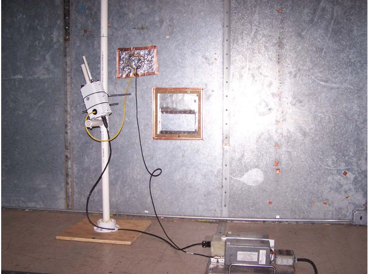
Photograph 3. Conducted Emissions Test Setup
