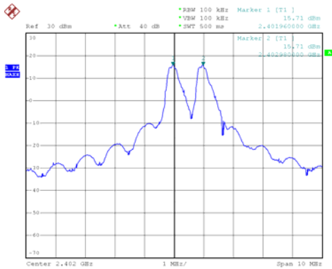
Channel 01 2402MHz
