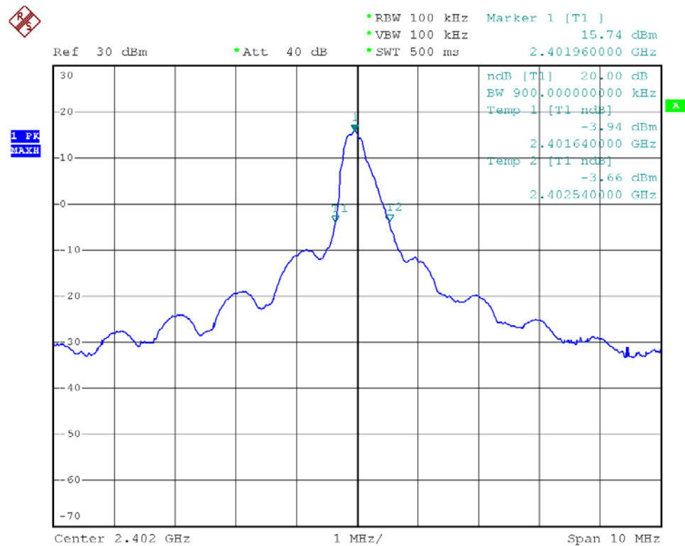
Figure Channel 00:
