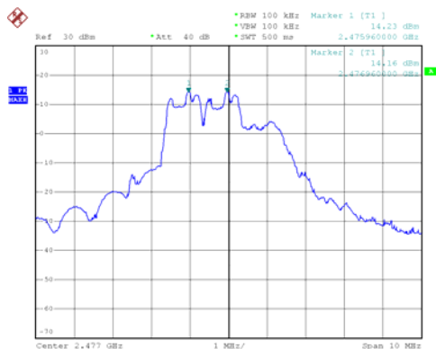
Channel 75 2477 MHz
