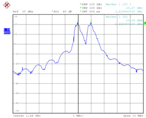
Channel 38 2440MHz
