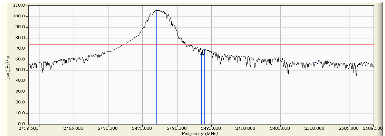
Figure Channel 75:
