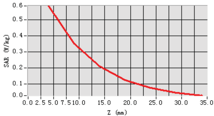
SAR, Z Axis Scan (X = 9, Y = 38)
