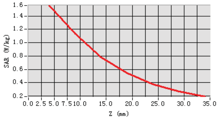
SAR, Z Axis Scan (X = -28, Y = -13)
