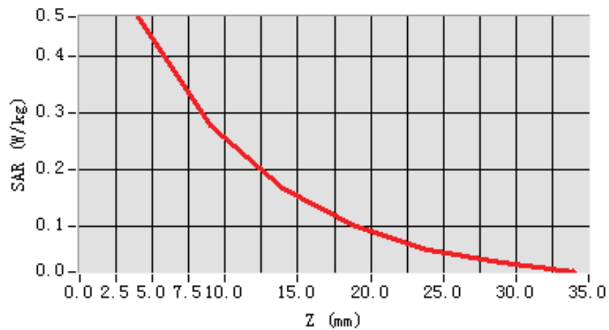
SAR, Z Axis Scan (X = 10, Y = 36)
