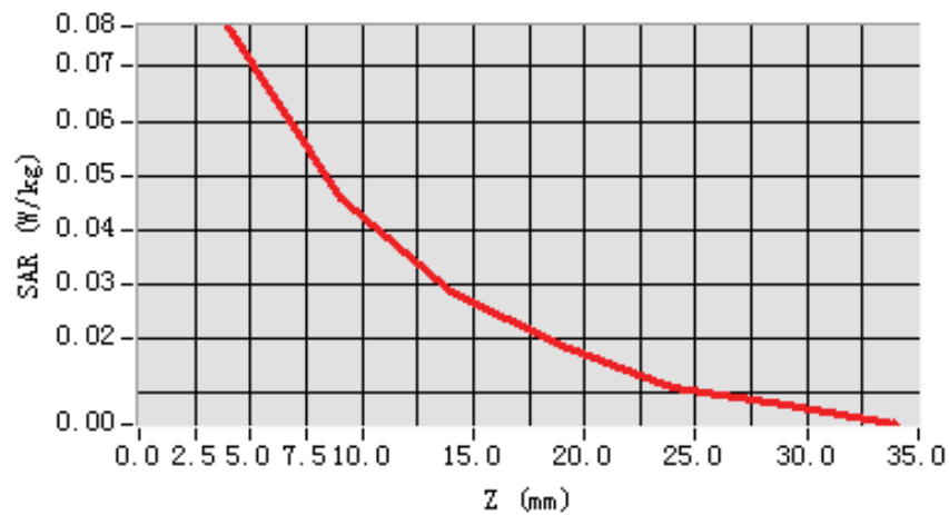
SAR, Z Axis Scan (X = -80, Y = -48)
