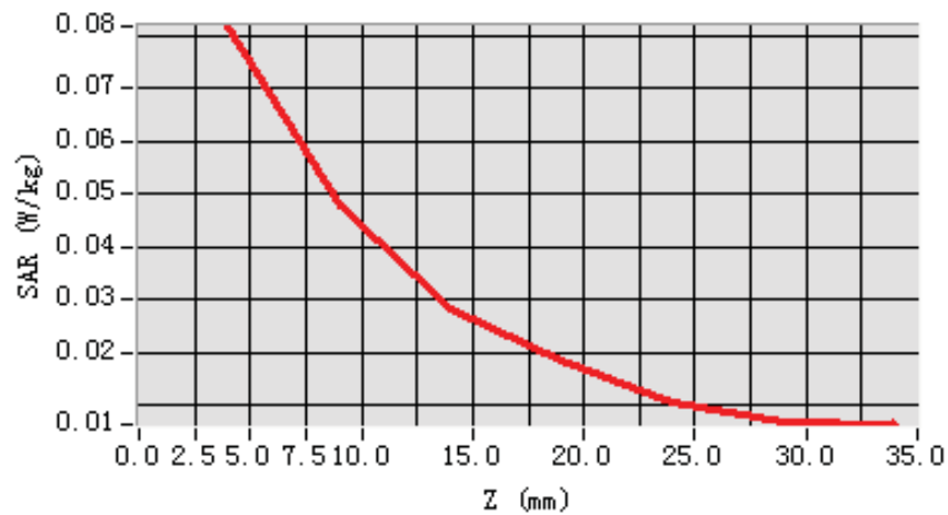
SAR, Z Axis Scan (X = -74, Y = -53)
