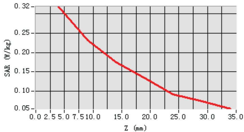
SAR, Z Axis Scan (X = -38, Y = -18)
