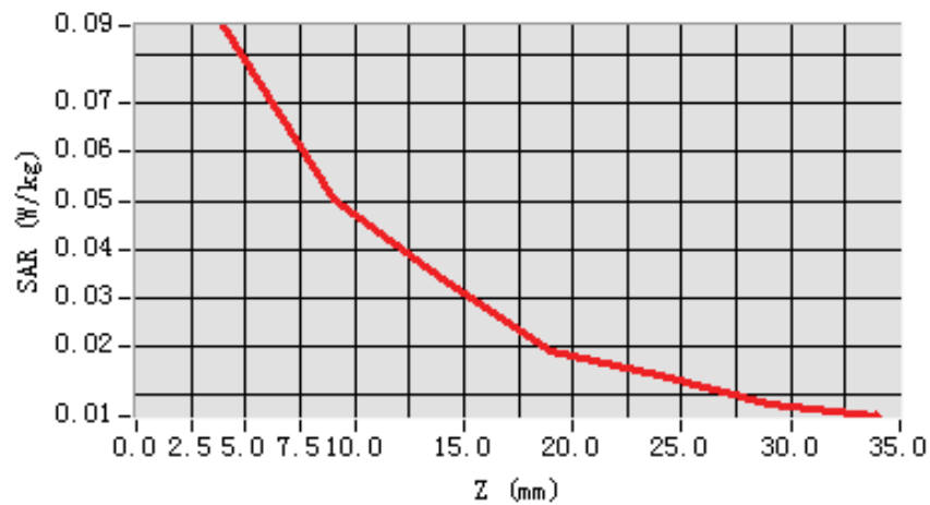
SAR, Z Axis Scan (X = -73, Y = -48)
