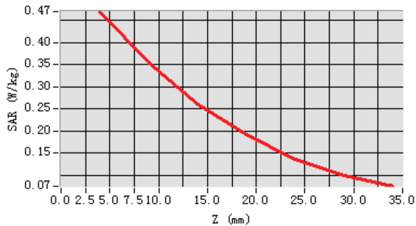
SAR, Z Axis Scan (X = -42, Y = -27)
