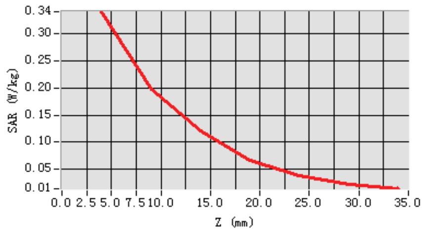
SAR, Z Axis Scan (X = -80, Y = -58)
