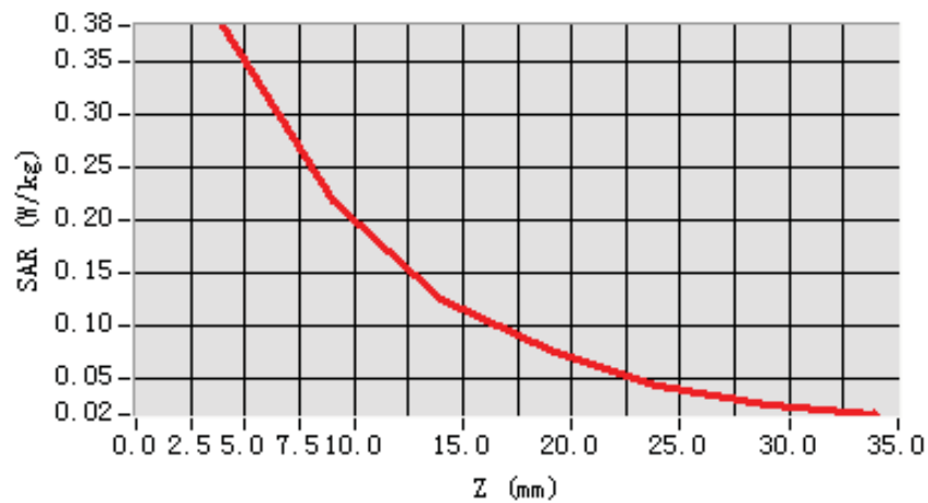
SAR, Z Axis Scan (X = -76, Y = -61)
