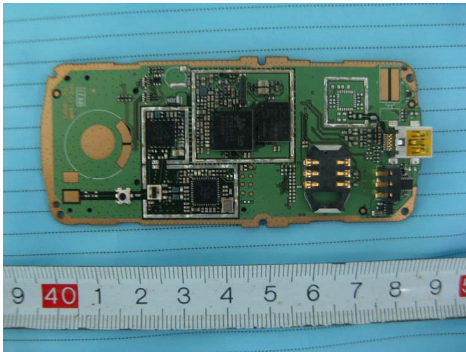
EUT – Main Board Bottom Unshielded View (Without FM Function for GPRS1218, GPRS1219)
