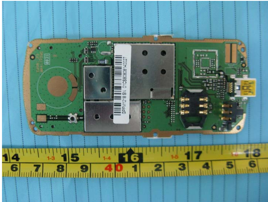
EUT – Main Board Bottom Shielded View (Without FM Function for GPRS1218, GPRS1219)
