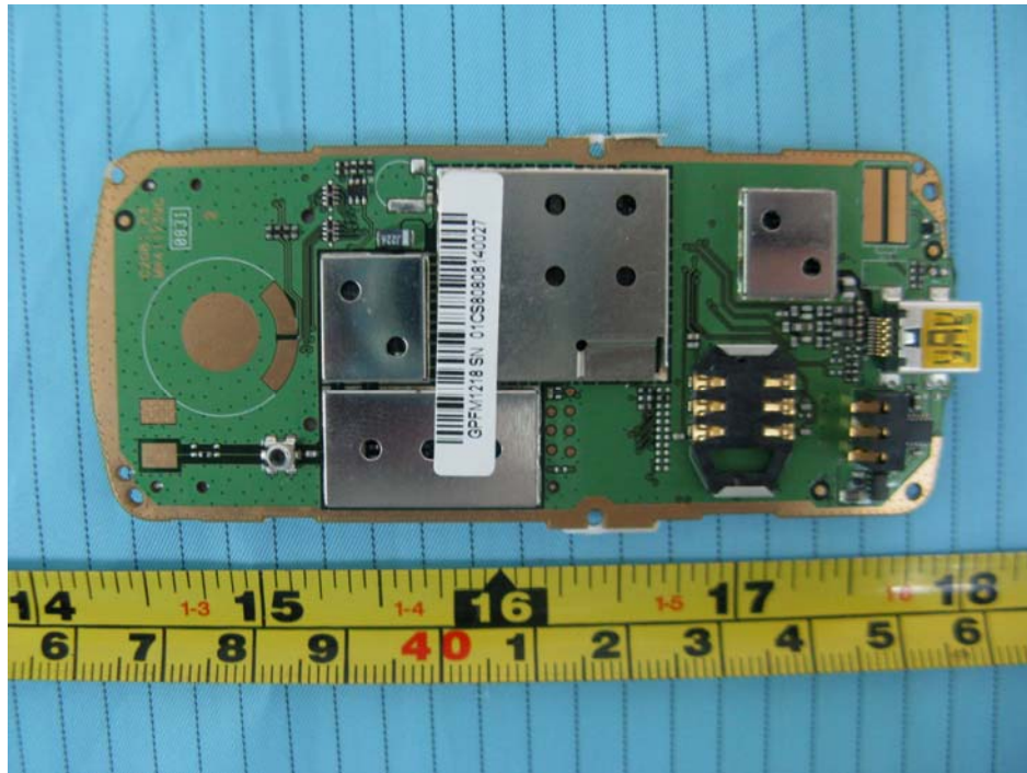
EUT – Main Board Bottom Shielded View
