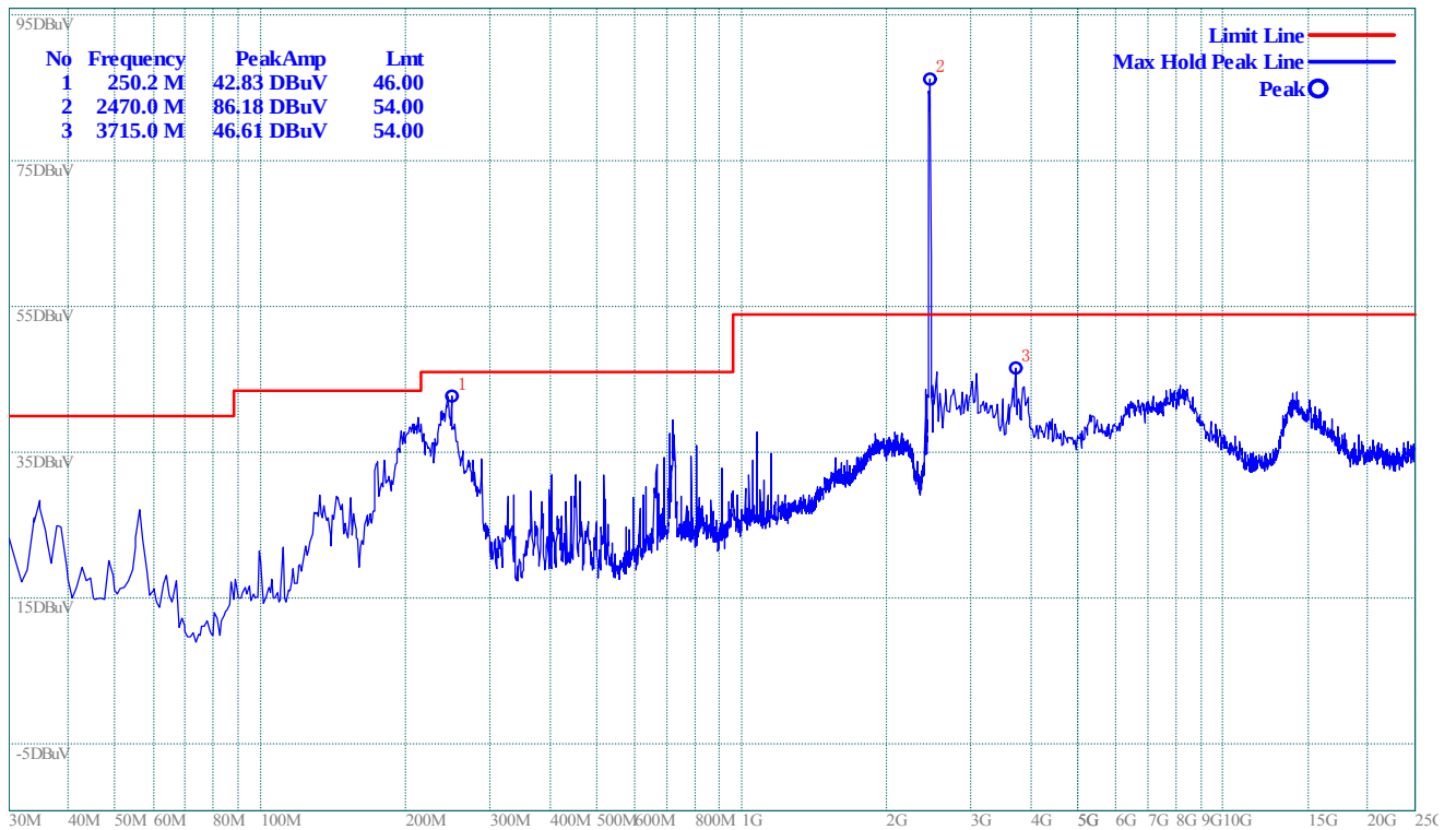
(Plot C.2: Antenna Horizontal, 30MHz to 25GHz)
