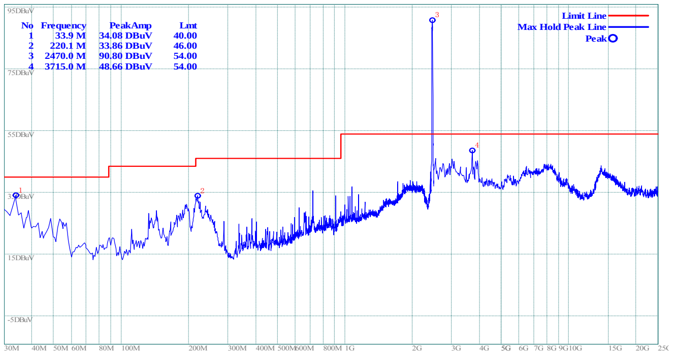
(Plot C.3: Antenna Vertical, 30MHz to 25GHz)
