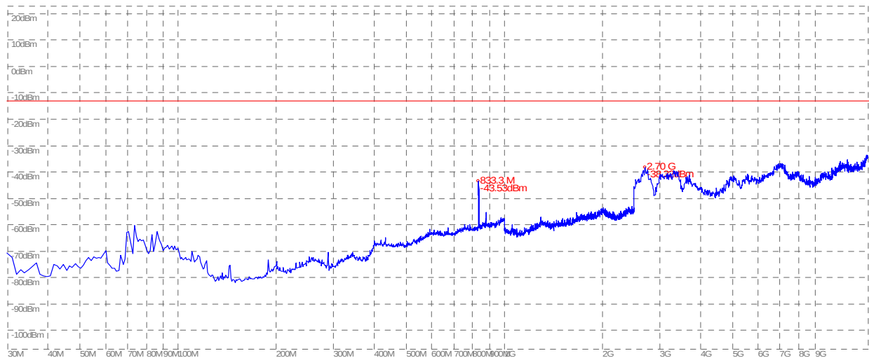
(Plot C.4: WCDMA 850MHz Channel = 4400, Test Antenna Vertical)
