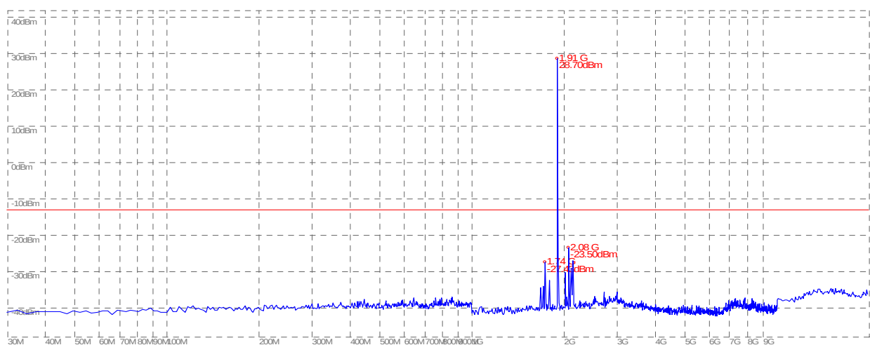
(Plot B3: GSM 1900MHz Channel = 810, 30MHz to 20GHz)
