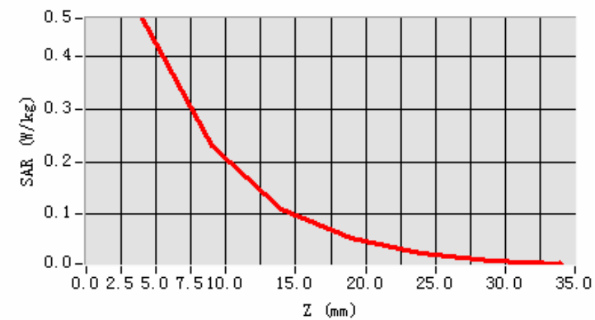
SAR, Z Axis Scan (X = 6, Y = -42)
