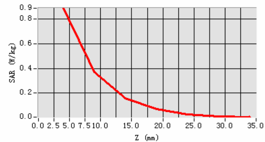
SAR, Z Axis Scan (X = -66, Y = -52)
