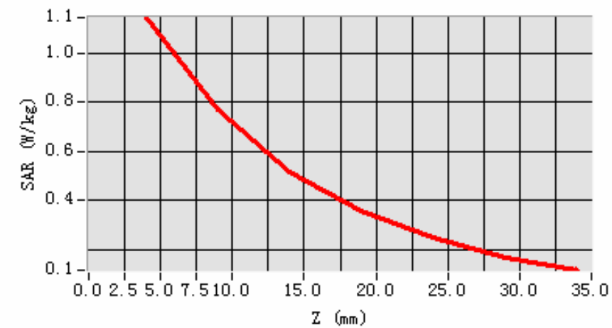
SAR, Z Axis Scan (X = 9, Y = -19)
