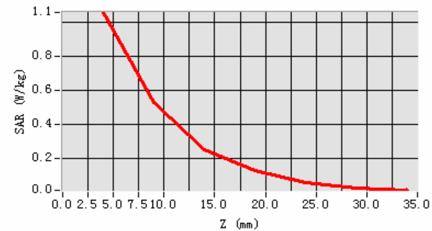
SAR, Z Axis Scan (X = 12, Y = -42)
