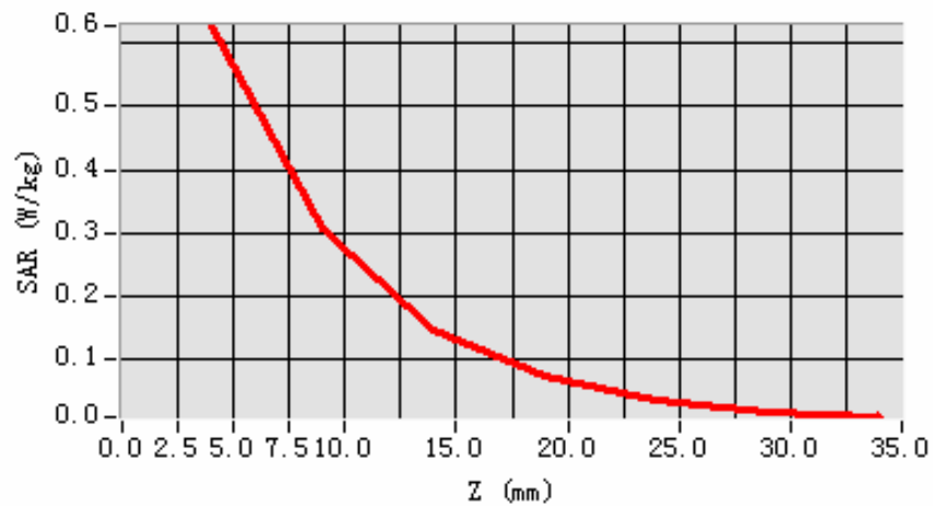
SAR, Z Axis Scan (X = 0, Y = 34)
