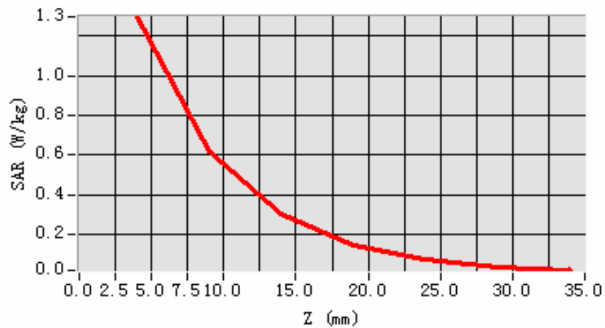
SAR, Z Axis Scan (X = -17, Y = 26)
