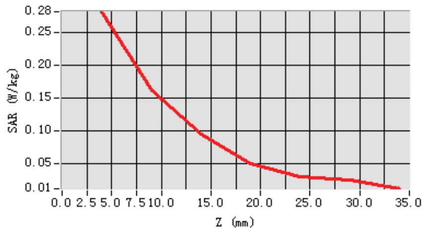
SAR, Z Axis Scan (X = 9, Y = 45)
