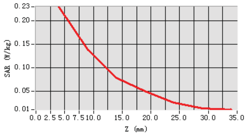
SAR, Z Axis Scan (X = -80, Y = -45)
