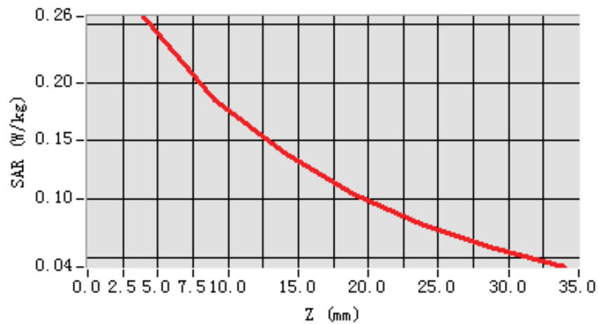
SAR, Z Axis Scan (X = -41, Y = -23)
