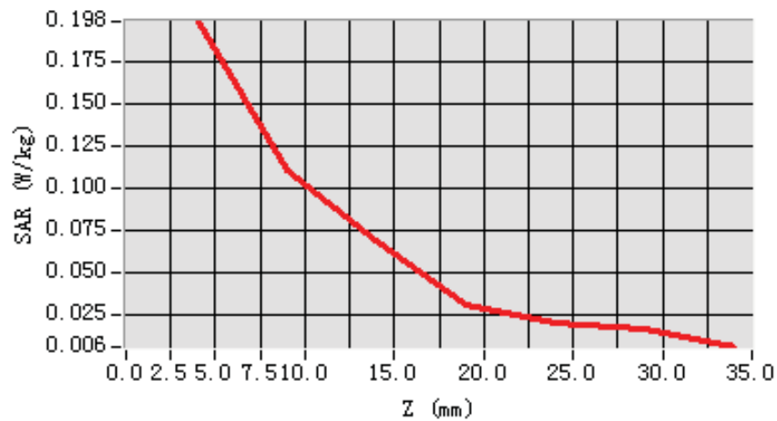
SAR, Z Axis Scan (X = -80, Y = -43)
