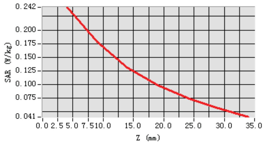
SAR, Z Axis Scan (X = -41, Y = -26)
