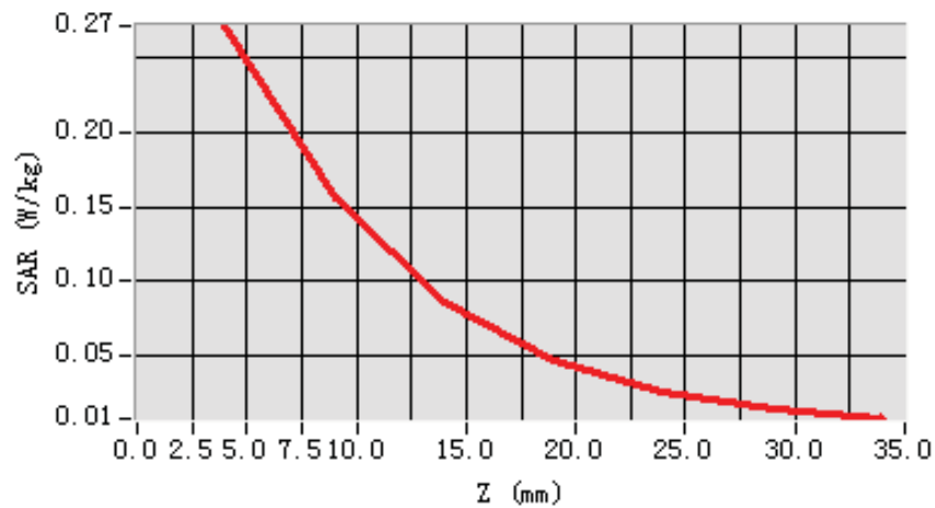
SAR, Z Axis Scan (X = -79, Y = -49)
