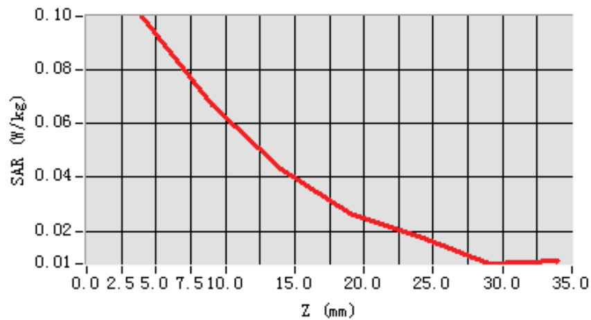
SAR, Z Axis Scan (X = -25, Y = 0)
