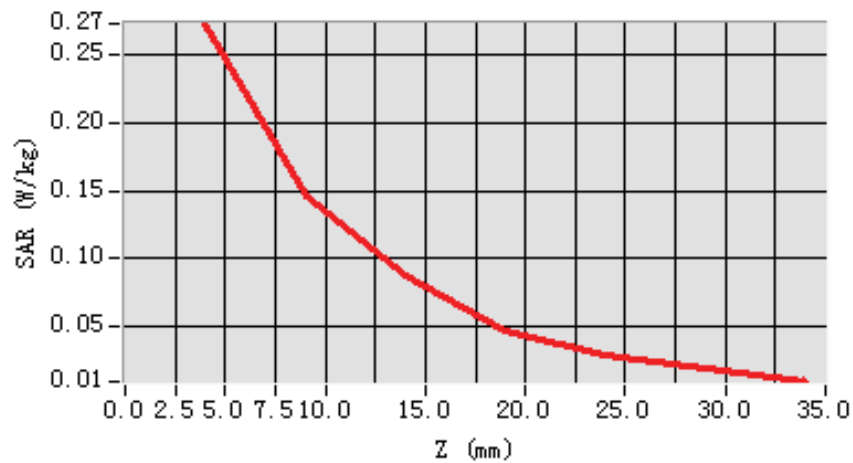
SAR, Z Axis Scan (X = -80, Y = -46)
