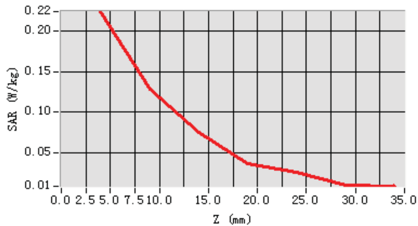
SAR, Z Axis Scan (X = -78, Y = -49)
