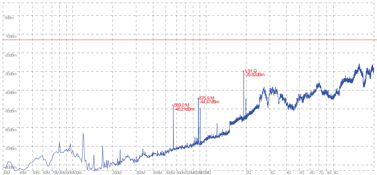
(Plot L.2: GPRS 1900MHz Channel = 810, Test Antenna Vertical)
