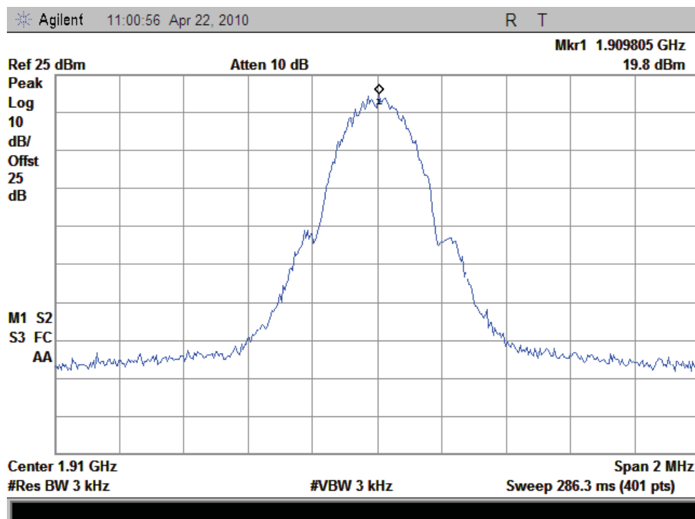
(Plot H: GPRS 1900MHz Channel = 810)
