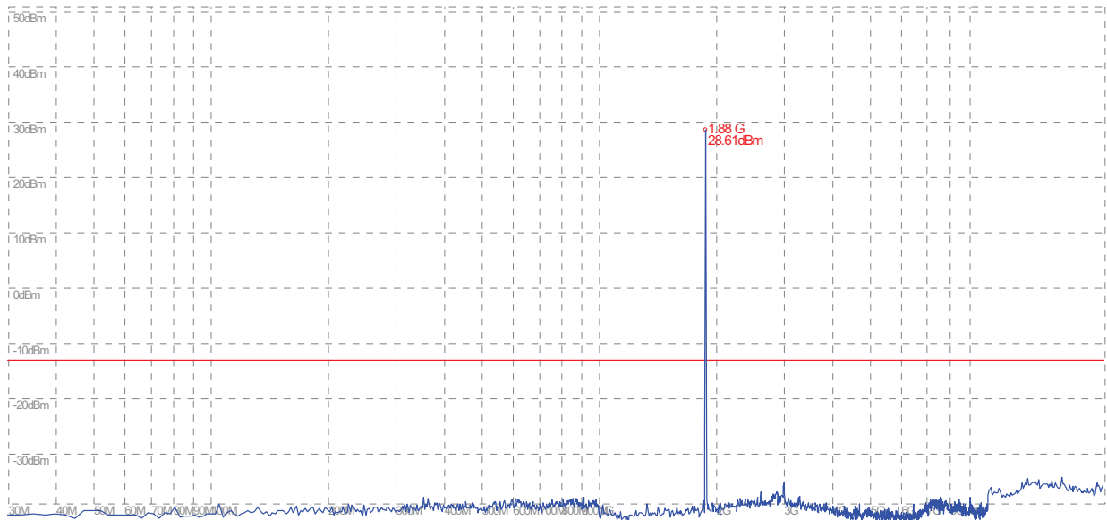
(Plot K: GPRS 1900MHz Channel = 661, 30MHz to 20GHz)
