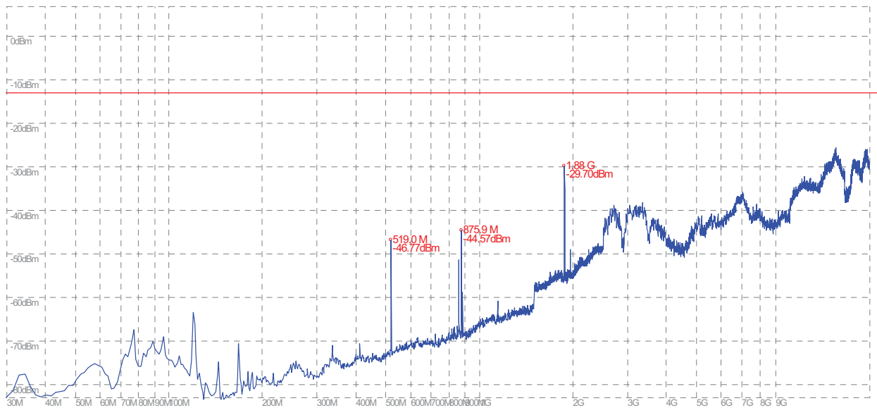
(Plot K.2: GPRS 1900MHz Channel = 661, Test Antenna Vertical)
