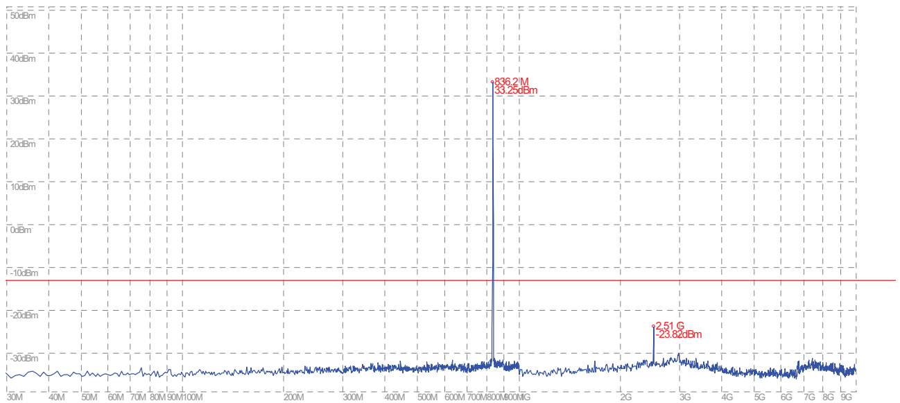
(Plot H: GPRS 850MHz Channel = 190, 30MHz to 10GHz)
