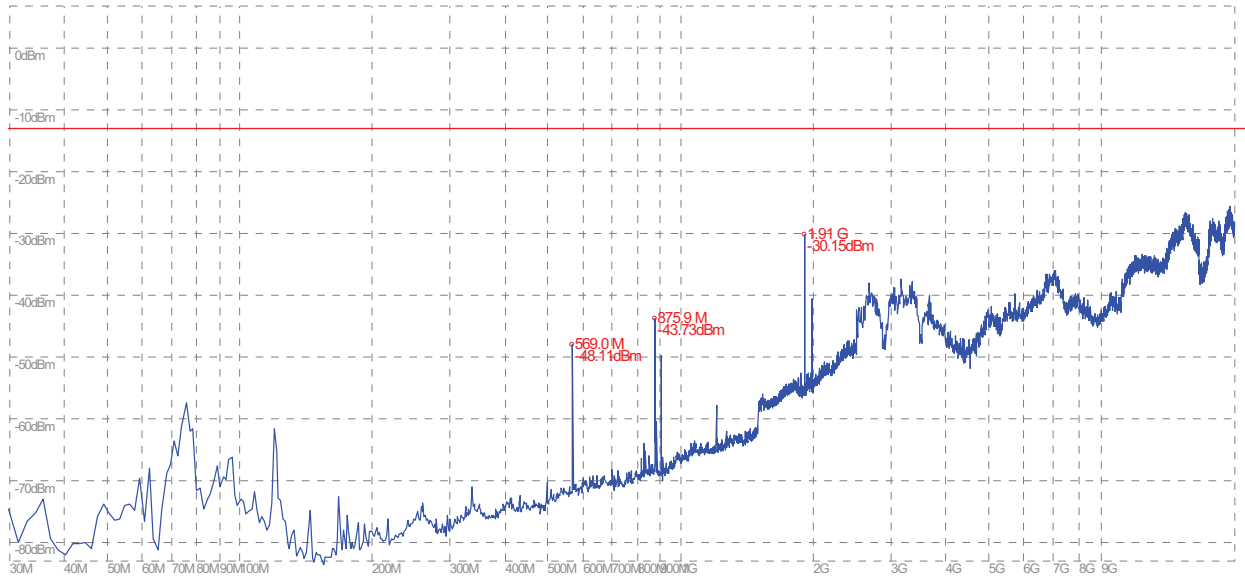
(Plot L.1: GPRS 1900MHz Channel = 810, Test Antenna Horizontal)
