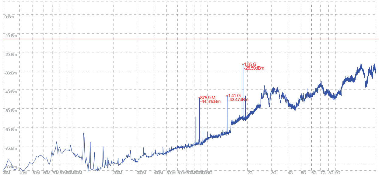
(Plot J.1: GPRS 1900MHz Channel = 512, Test Antenna Horizontal)
