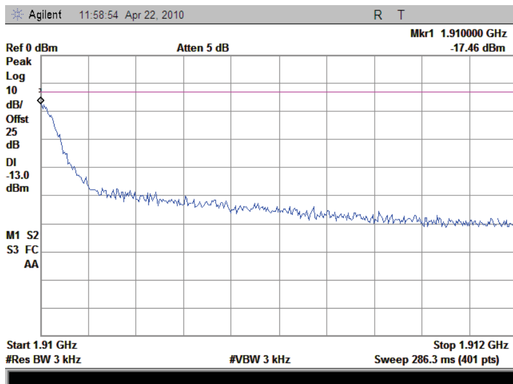
(Plot D: GPRS Channel = 810)
