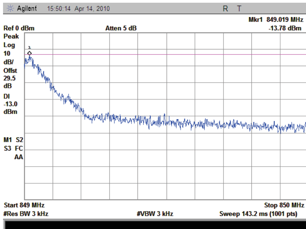
(Plot B: GSM Channel = 251)
