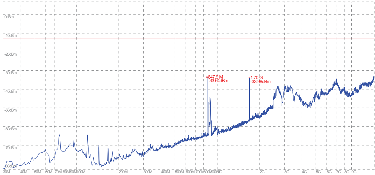
(Plot I.1: GPRS 850MHz Channel = 251, Test Antenna Horizontal)
