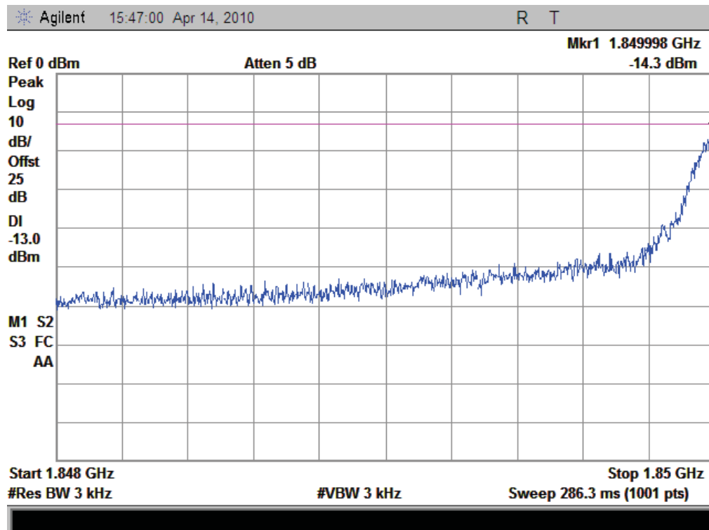
(Plot C: GSM Channel = 512)
