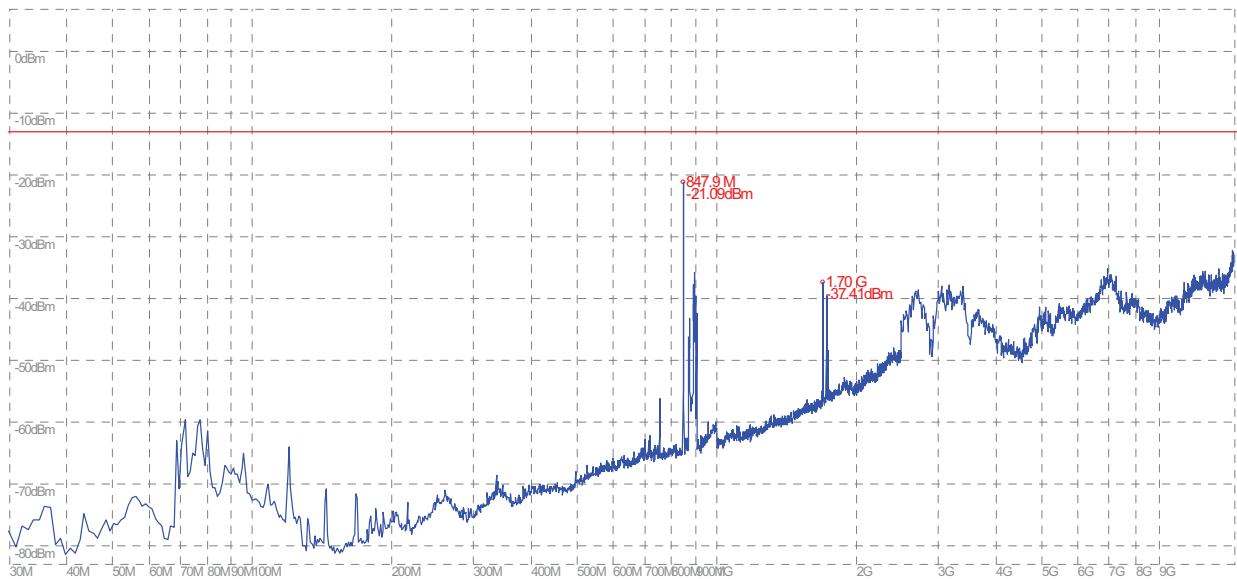
(Plot I.2: GPRS 850MHz Channel = 251, Test Antenna Vertical)
