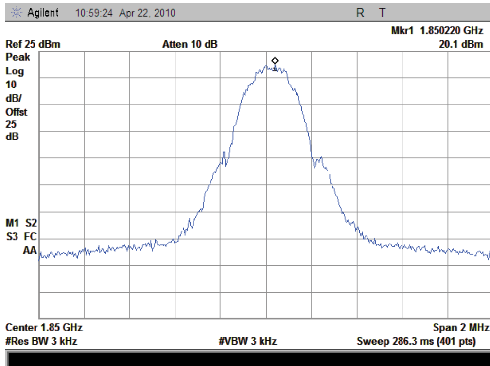
(Plot G: GPRS 1900MHz Channel = 512)
