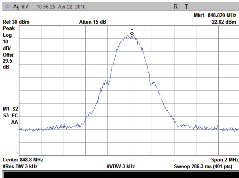
(Plot F: GPRS 850MHz Channel = 251)
