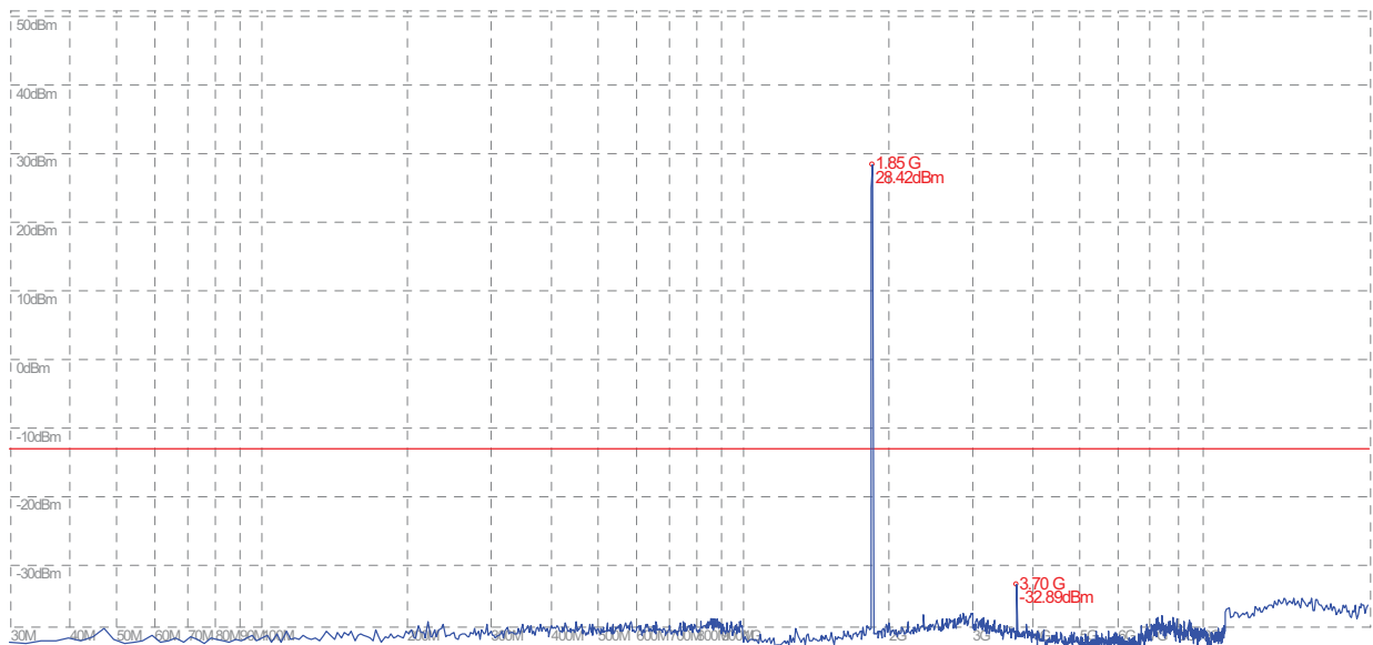
(Plot J: GPRS 1900MHz Channel = 512, 30MHz to 20GHz)
