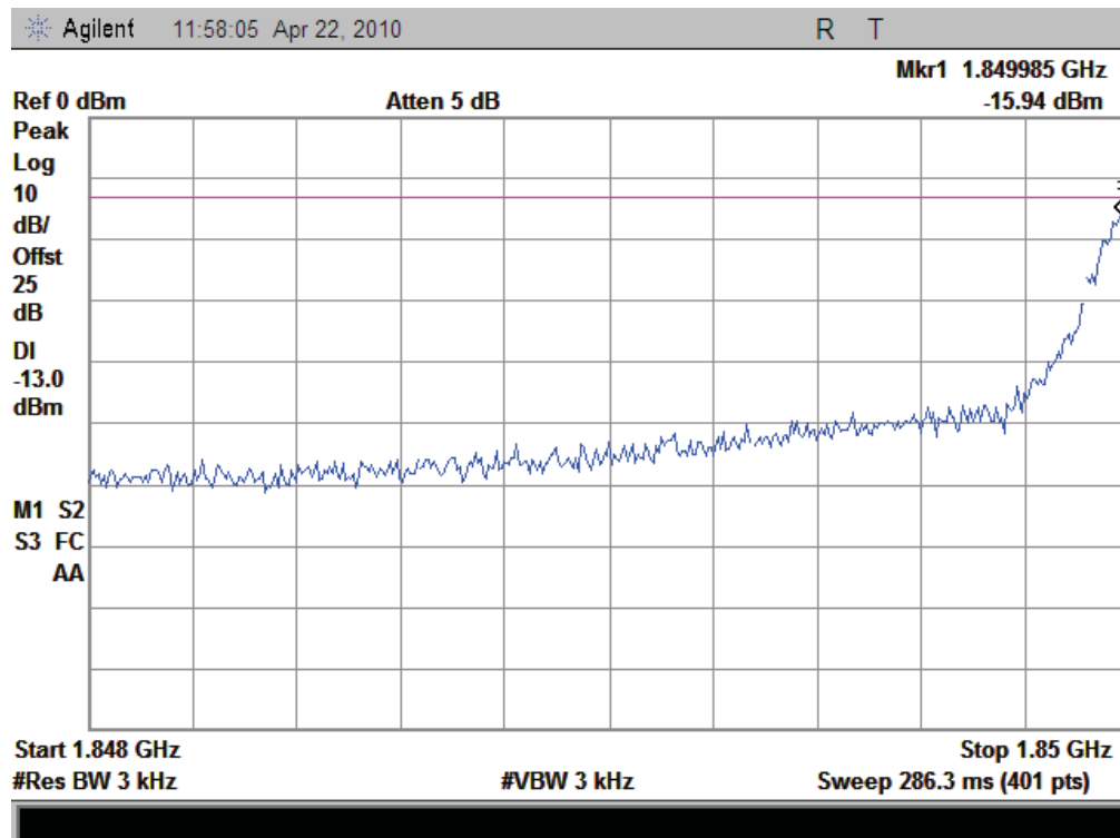
(Plot C: GPRS Channel = 512)
