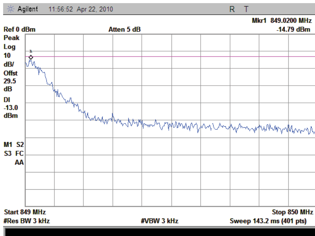
(Plot B: GPRS Channel = 251)
