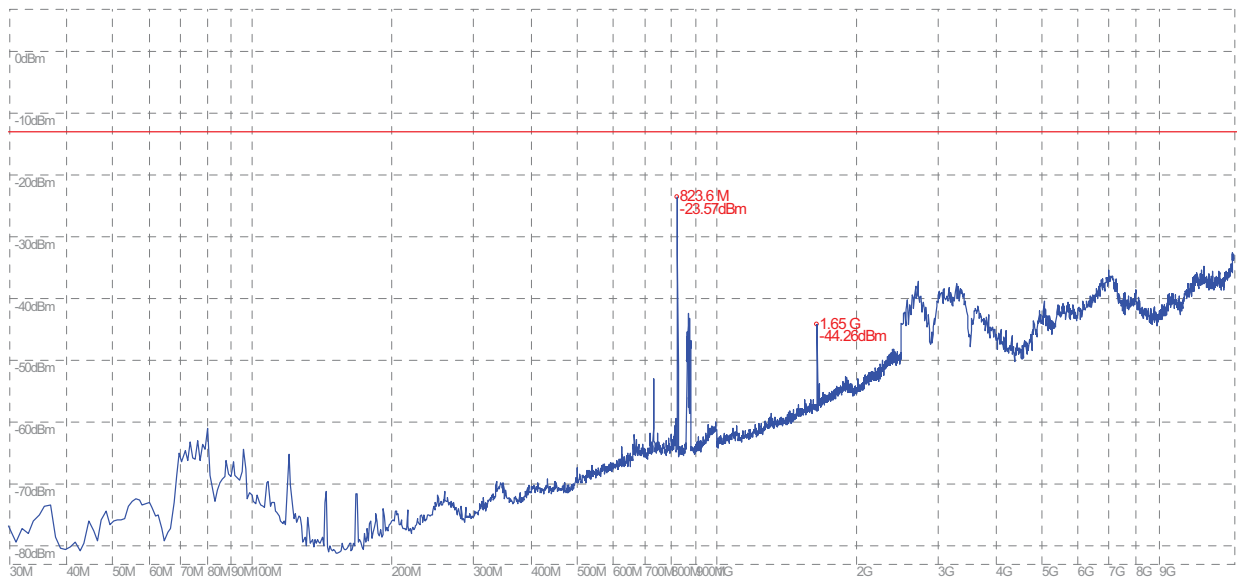
(Plot G.2: GPRS 850MHz Channel = 128, Test Antenna Vertical)
