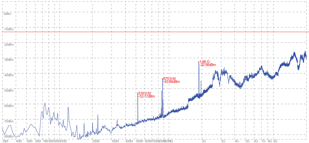
(Plot K.1: GPRS 1900MHz Channel = 661, Test Antenna Horizontal)
