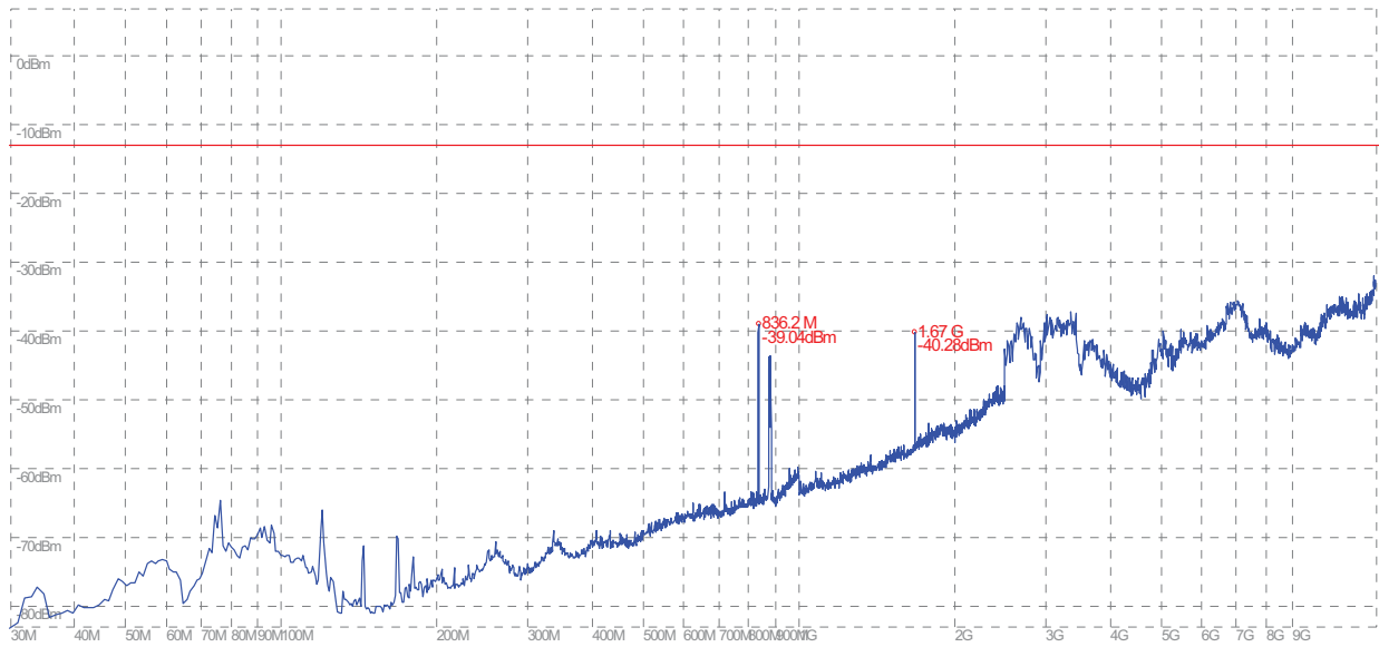
(Plot H.1: GPRS 850MHz Channel = 190, Test Antenna Horizontal)
