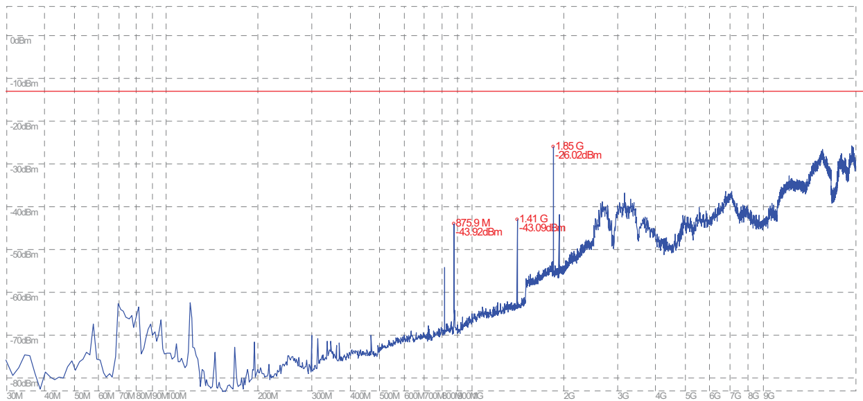
(Plot J.2: GPRS 1900MHz Channel = 512, Test Antenna Vertical)
