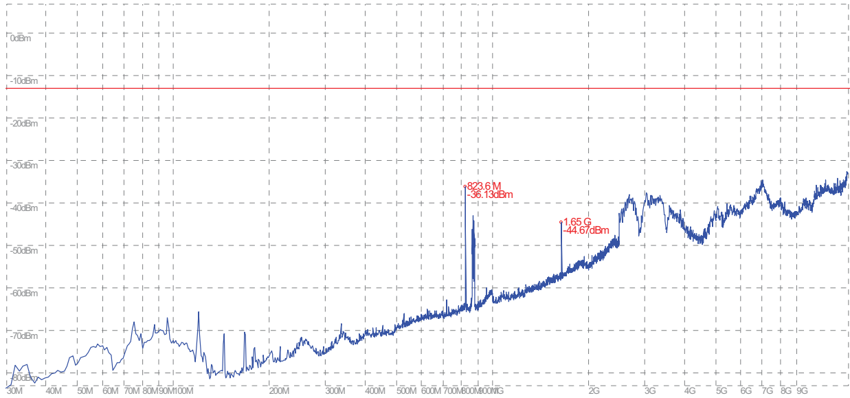
(Plot G.1: GPRS 850MHz Channel = 128, Test Antenna Horizontal)
