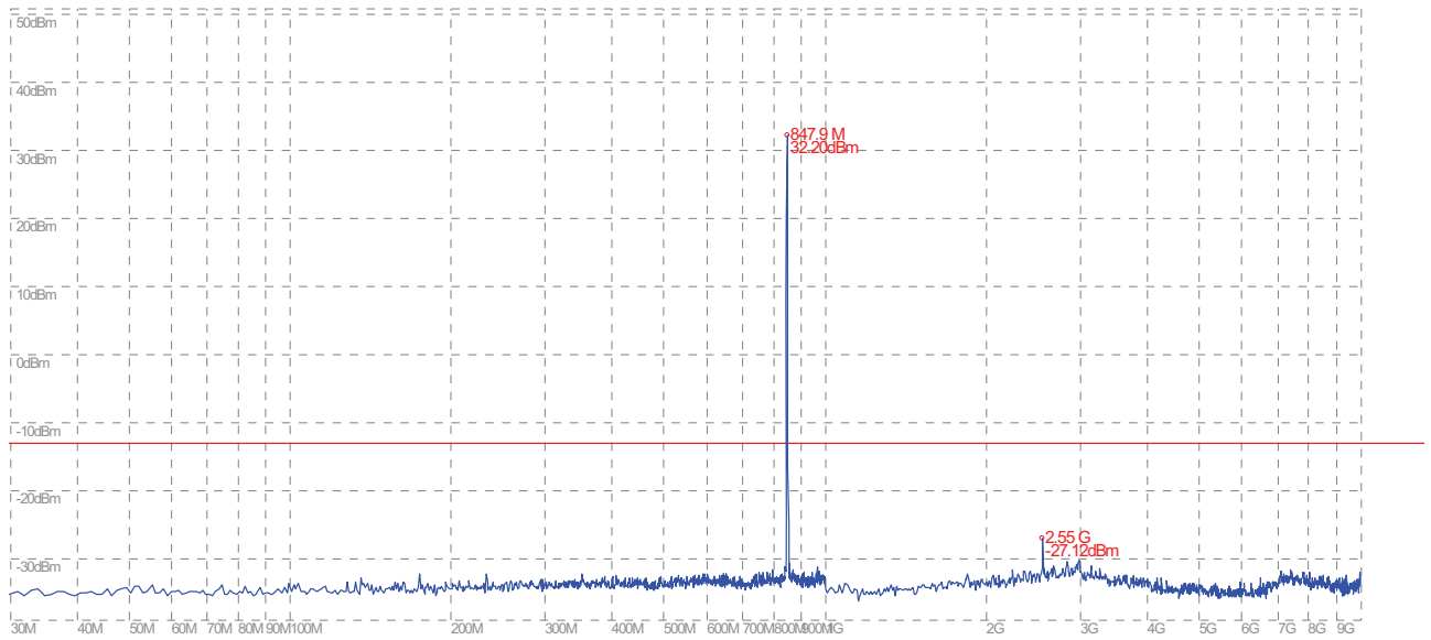
(Plot I: GPRS 850MHz Channel = 251, 30MHz to 10GHz)
