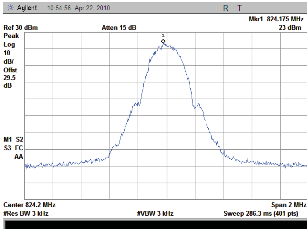
(Plot E: GPRS 850MHz Channel = 128)
