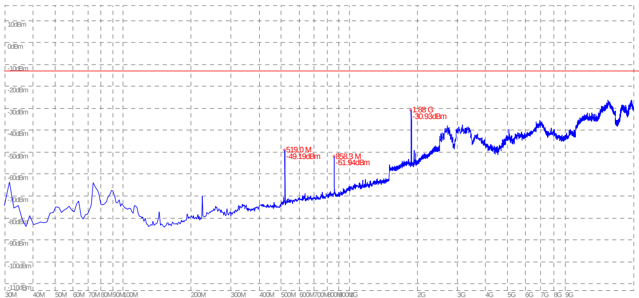
(Plot B.2: GSM 1900MHz Channel = 661, Test Antenna Vertical)
