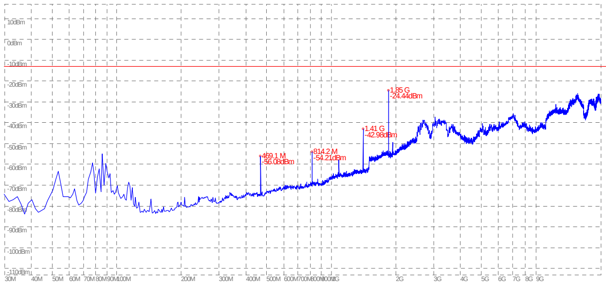
(Plot A.2: GSM 1900MHz Channel = 512, Test Antenna Vertical)
