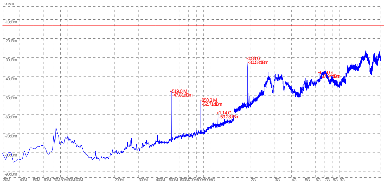
(Plot B.1: GSM 1900MHz Channel = 661, Test Antenna Horizontal)
