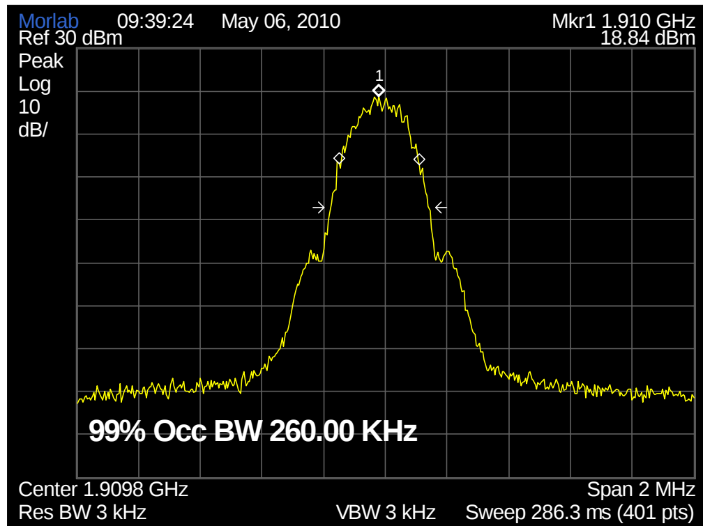
(Plot C: GSM 1900MHz Channel = 810)
