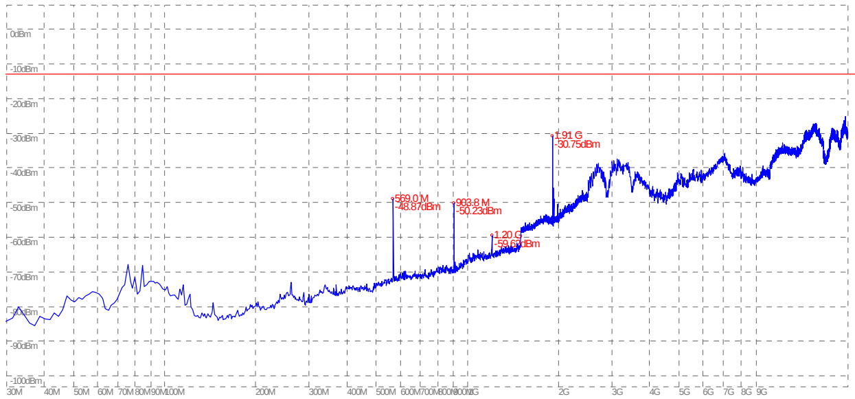
(Plot C.1: GSM 1900MHz Channel = 810, Test Antenna Horizontal)
