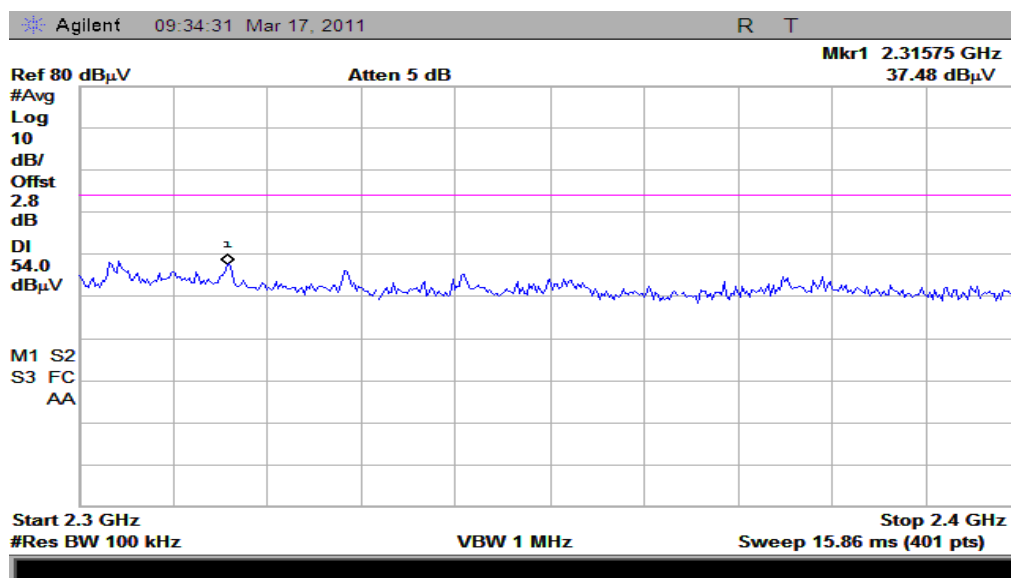
(Plot A2: Channel = 0 AVERAGE)
