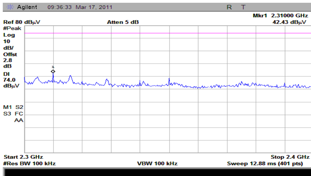
(Plot A1: Channel = 0 PEAK)
