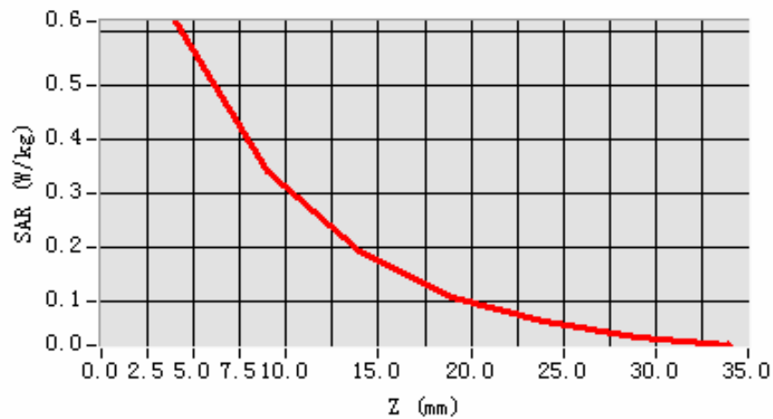
SAR, Z Axis Scan (X = 0, Y = 35)
