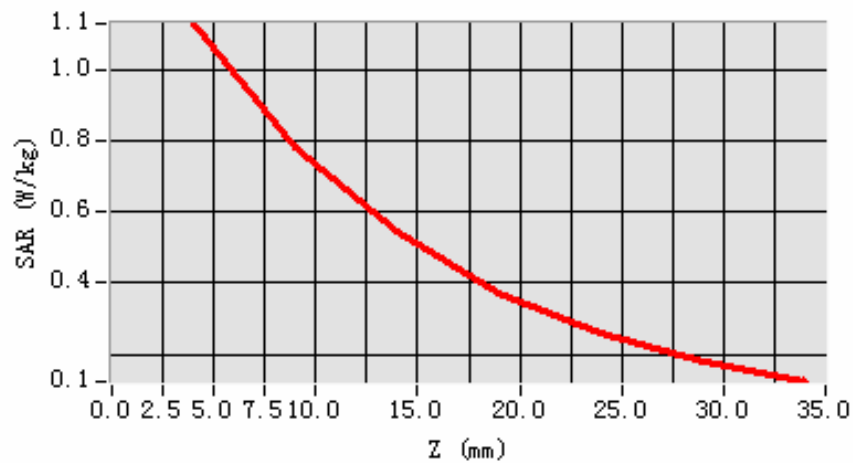
SAR, Z Axis Scan (X = -28, Y = -11)
