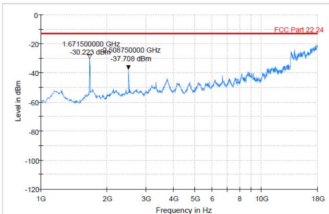
Field Strength of Spurious Radiated 1GHz-18GHz Vertical
