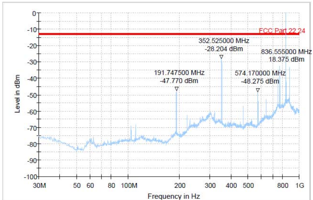
Field Strength of Spurious Radiated 30MHz-1GHz Vertical
