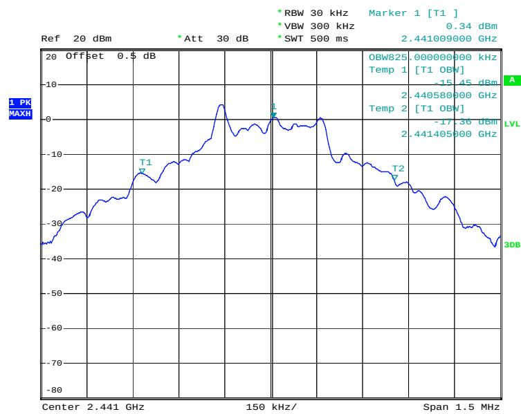
99% Occupied Bandwidth Plot on Channel 39
