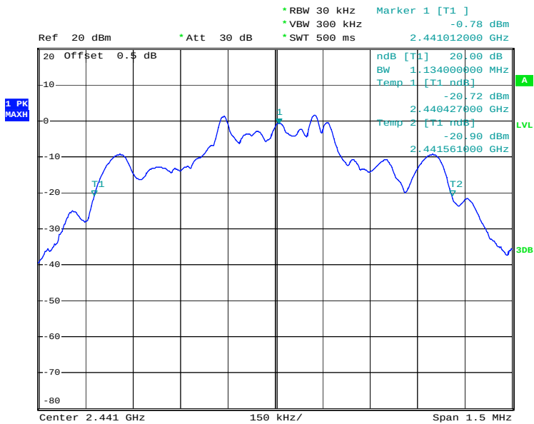
20 dB Bandwidth Plot on Channel 39
