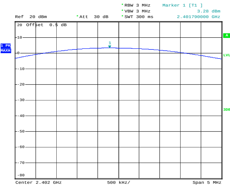
Peak Output Power Plot on Channel 00
