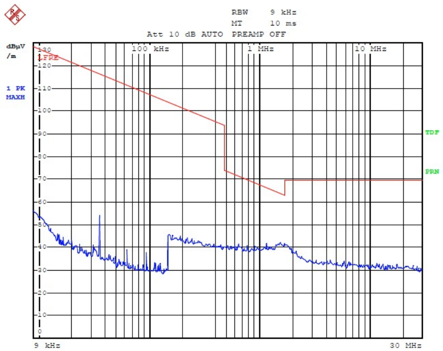
Radiated Emission Plot between 9 kHz ~ 30MHz (Horizontal)
