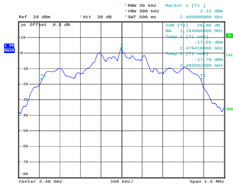
20 dB Bandwidth Plot on Channel 78
