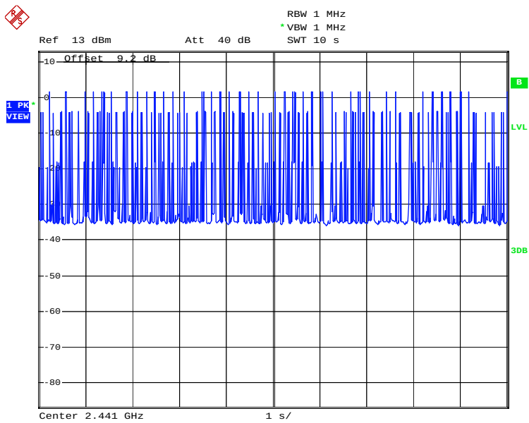
2DH3 Dwell Time (Count Pulses) Plot on Channel 39
