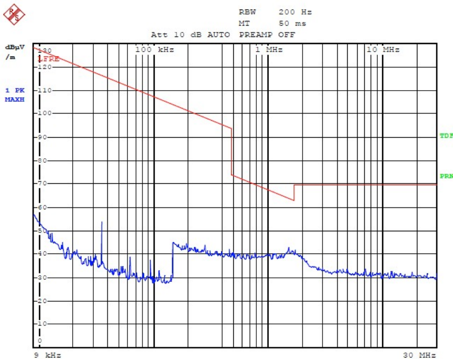
Radiated Emission Plot between 9 kHz ~ 30MHz (Vertical)
