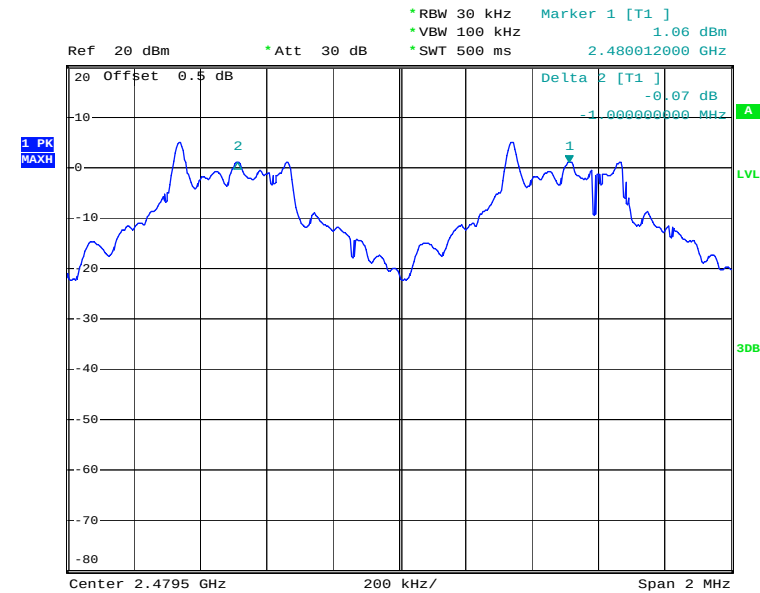
Channel Separation Plot on Channel 77 - 78
