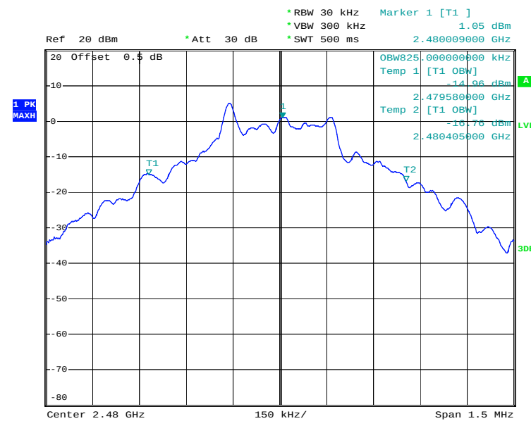
99% Occupied Bandwidth Plot on Channel 78
