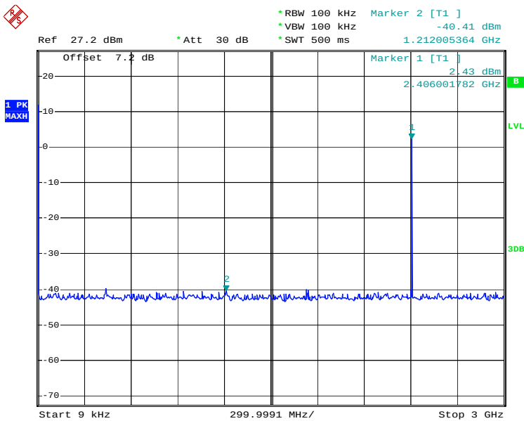
Conducted Spurious Emission Plot between 9 kHz ~ 3 GHz
