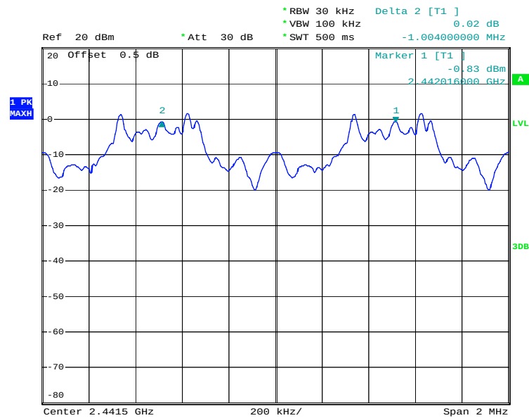
Channel Separation Plot on Channel 39 - 40
