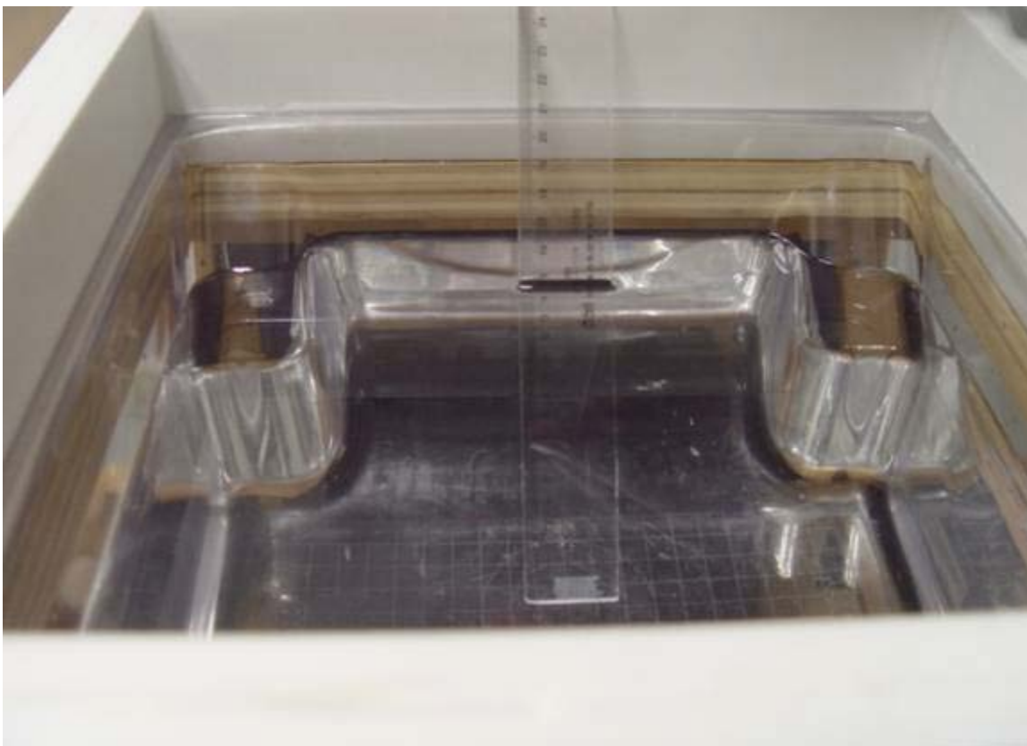
Photo of Liquid Height for Body SAR
