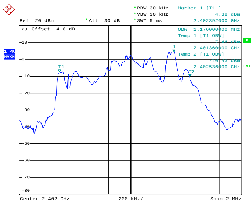
99% Bandwidth Plot on Channel 00
