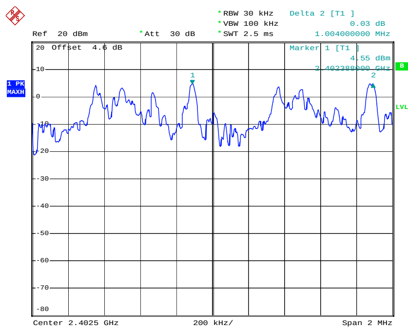
Channel Separation Plot on Channel 00 - 01
