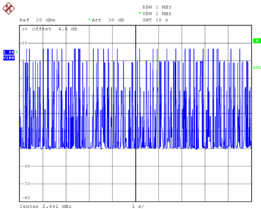
DH5 Dwell Time (Count Pulses) Plot on Channel 39
