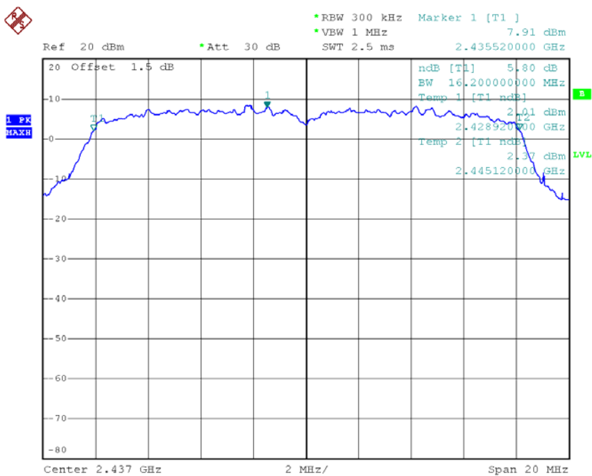
Mode 5 : 6 dB Bandwidth Plot on 802.11g Channel 06
