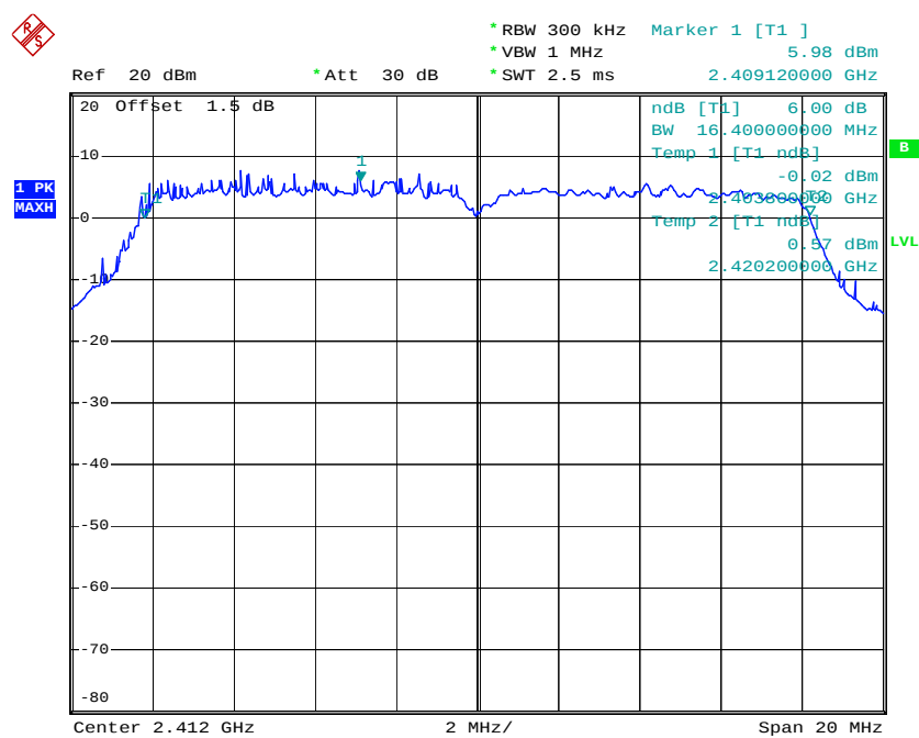
Mode 4 : 6 dB Bandwidth Plot on 802.11g Channel 01
