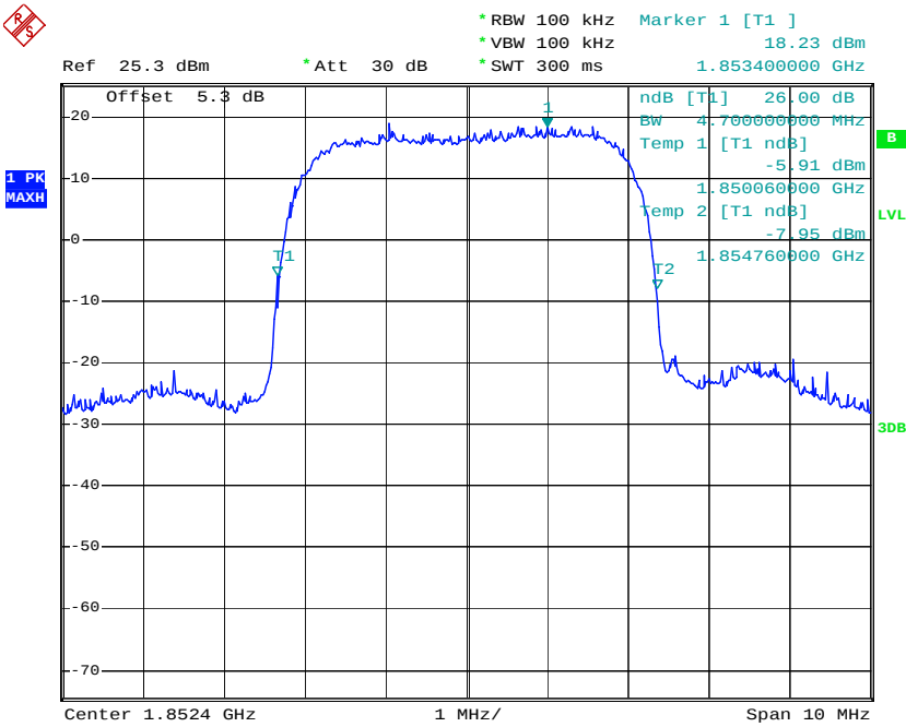
26dB Bandwidth Plot on Channel 9262
