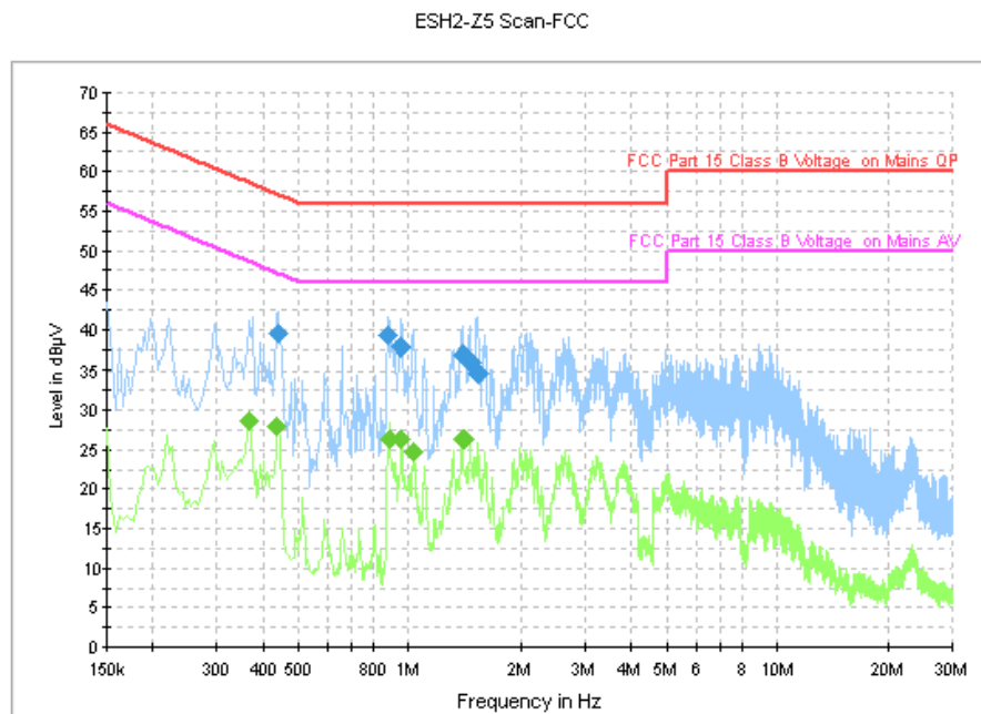
Fig. 81 AC Powerline Conducted Emission-802.11b
