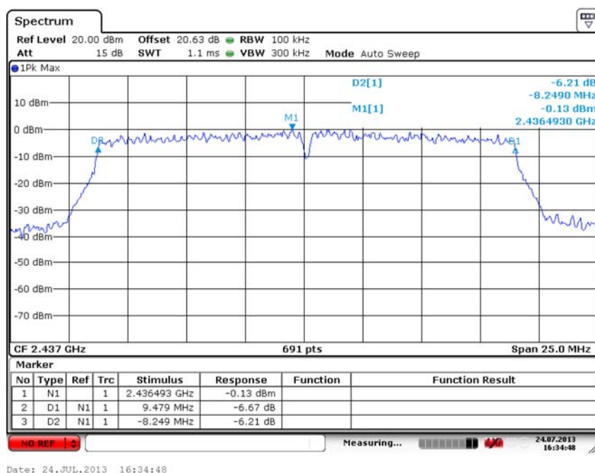
Fig. 17 Occupied 6dB Bandwidth (802.11 n-20MHz, Ch 6)
