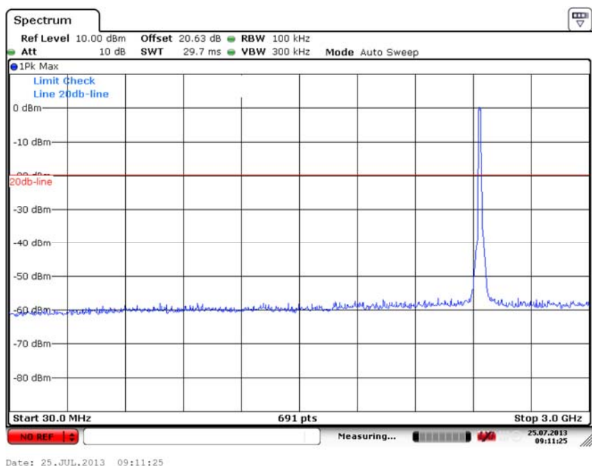
Fig. 38 Conducted Spurious Emission (802.11g, Ch6, 30 MHz-3 GHz)
