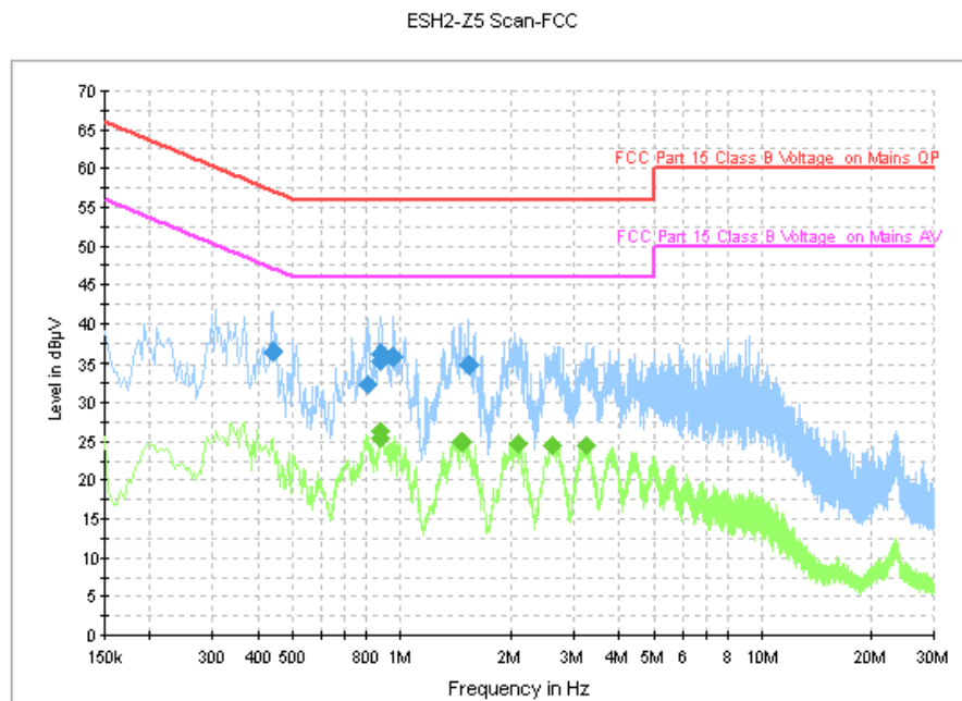
Fig. 83 AC Powerline Conducted Emission-802.11n-20M
