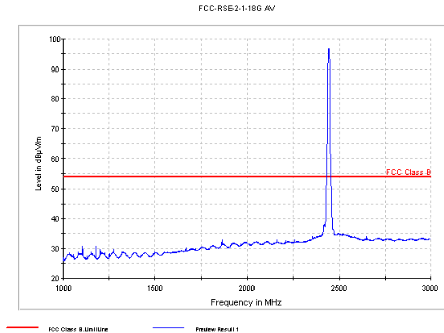
Fig. 57 Radiated Spurious Emission (802.11b, Ch6, 1 GHz-3 GHz)
