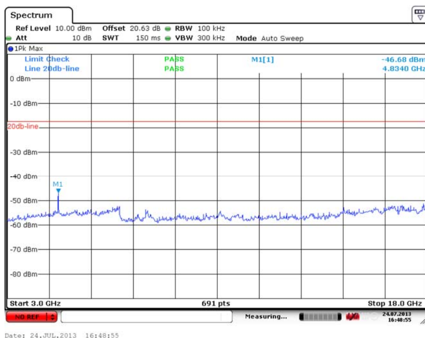
Fig. 27 Conducted Spurious Emission (802.11b, Ch1, 3 GHz-18 GHz)
