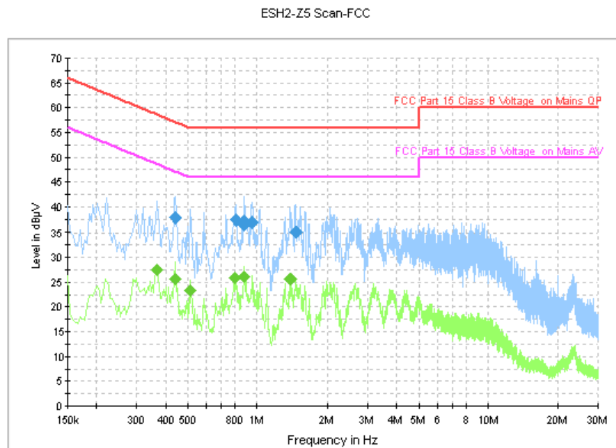
Fig. 82 AC Powerline Conducted Emission-802.11g
