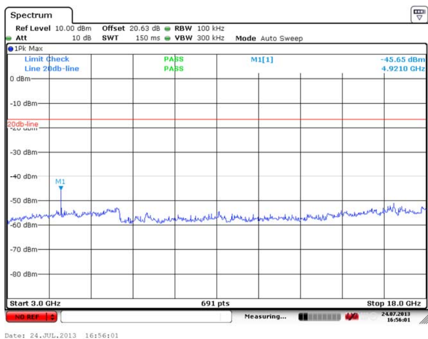
Fig. 33 Conducted Spurious Emission (802.11b, Ch11, 3 GHz-18 GHz)
