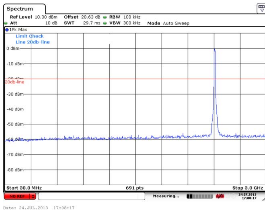
Fig. 44 Conducted Spurious Emission (802.11n-20M, Ch1, 30 MHz-3 GHz)
