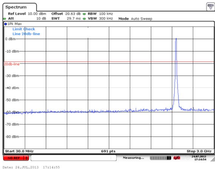
Fig. 50 Conducted Spurious Emission (802.11n-20M, Ch11, 30 MHz-3 GHz)
