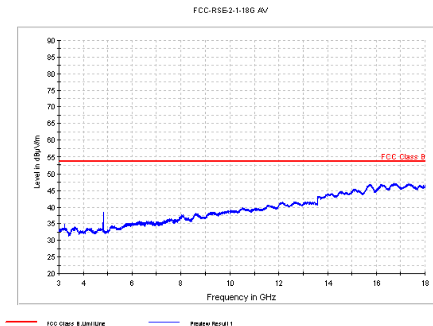
Fig. 73 Radiated Spurious Emission (802.11n-20M, Ch1, 3 GHz-18 GHz)
