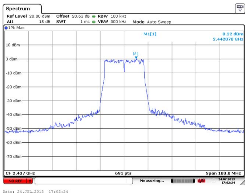
Fig. 37 Conducted Spurious Emission (802.11g, Ch6, Center Frequency)
