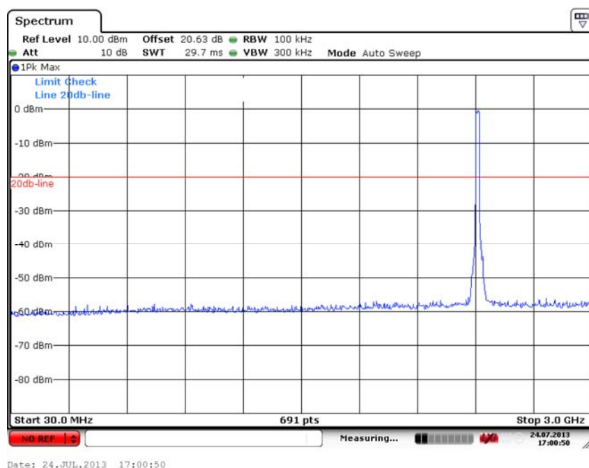
Fig. 35 Conducted Spurious Emission (802.11g, Ch1, 30 MHz-3 GHz)
