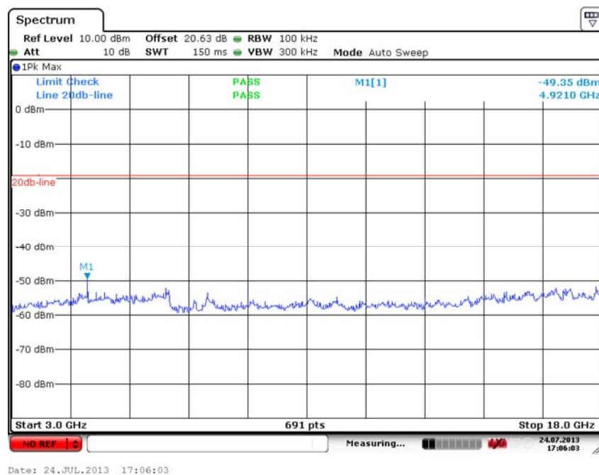
Fig. 42 Conducted Spurious Emission (802.11g, Ch11, 3 GHz-18 GHz)
