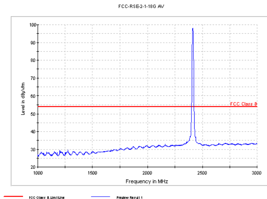
Fig. 54 Radiated Spurious Emission (802.11b, Ch1, 1 GHz-3 GHz)
