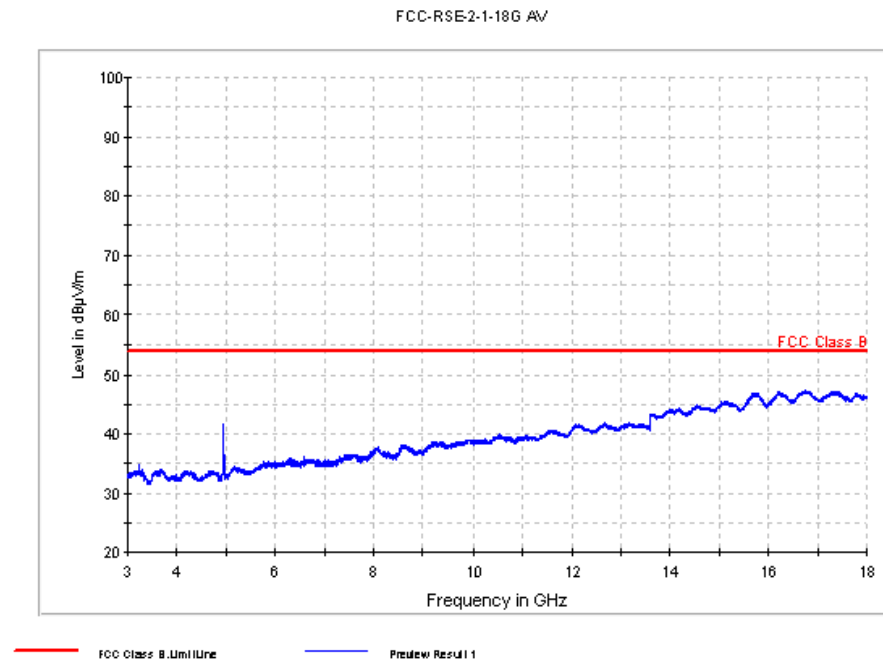
Fig. 79 Radiated Spurious Emission (802.11n-20M, Ch11, 3 GHz-18 GHz)
