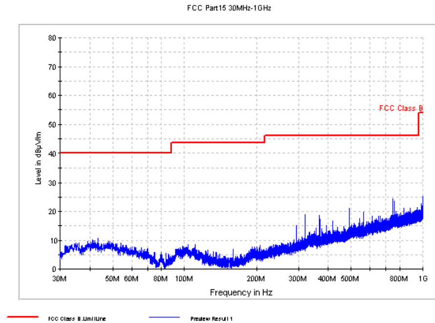
Fig. 71 Radiated Spurious Emission (802.11n-20M, Ch1, 30 MHz-1 GHz)
