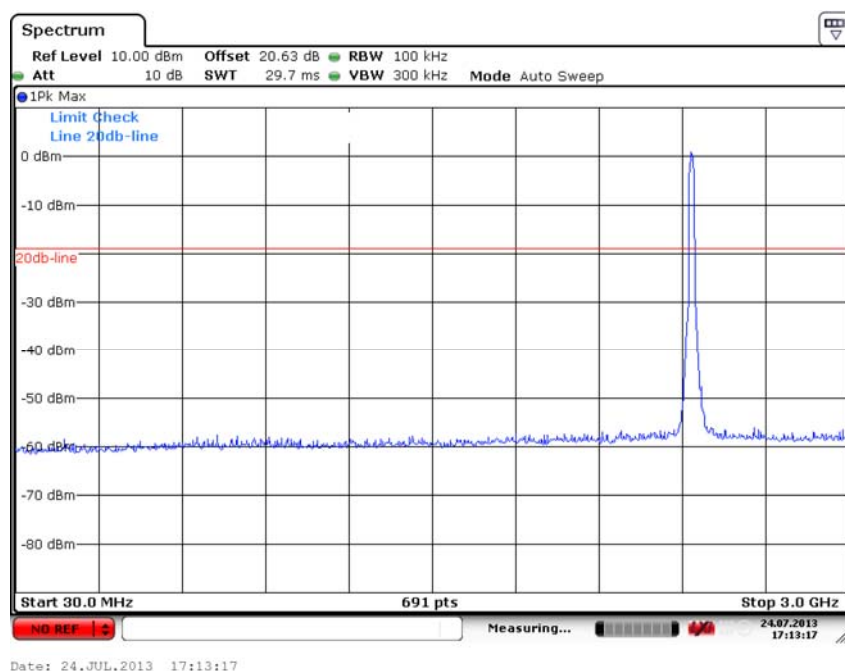
Fig. 47 Conducted Spurious Emission (802.11n-20M, Ch6, 30 MHz-3 GHz)
