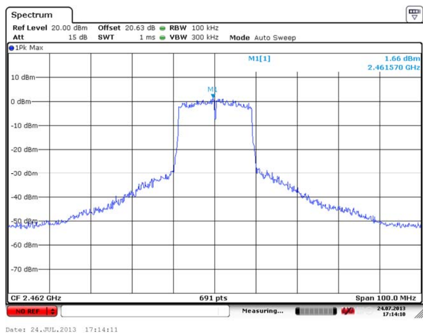
Fig. 49 Conducted Spurious Emission (802.11n-20M, Ch11, Center Frequency)
