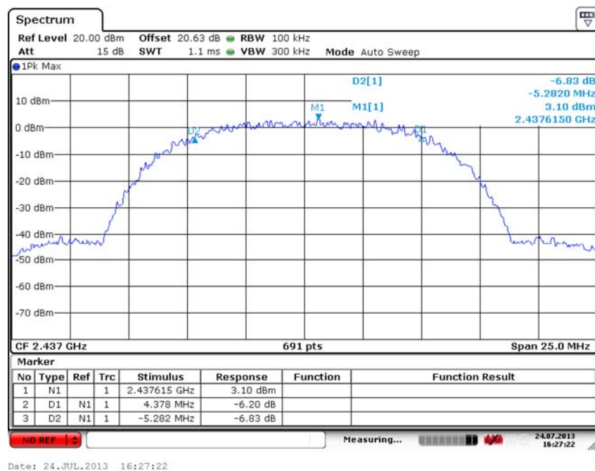
Fig. 11 Occupied 6dB Bandwidth (802.11b, Ch 6)
