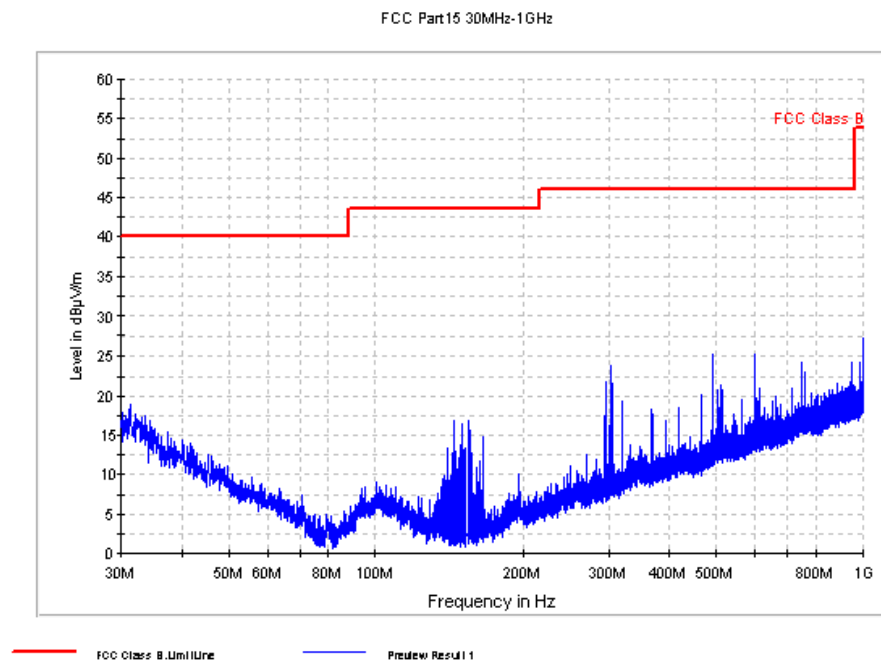
Fig. 56 Radiated Spurious Emission (802.11b, Ch6, 30 MHz-1 GHz)
