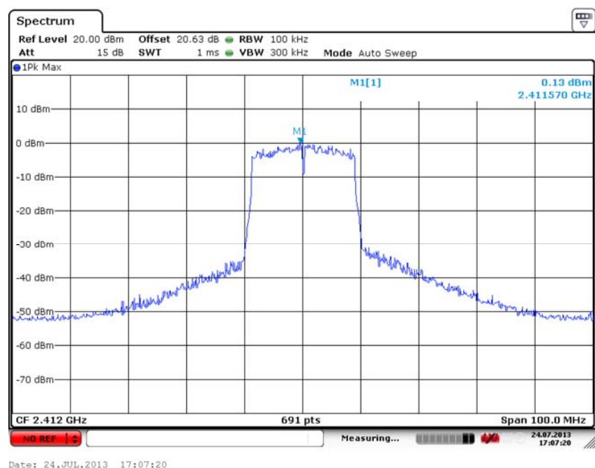
Fig. 43 Conducted Spurious Emission (802.11n-20M, Ch1, Center Frequency)
