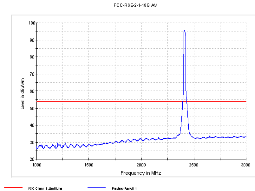
Fig. 75 Radiated Spurious Emission (802.11n-20M, Ch6, 1 GHz-3 GHz)
