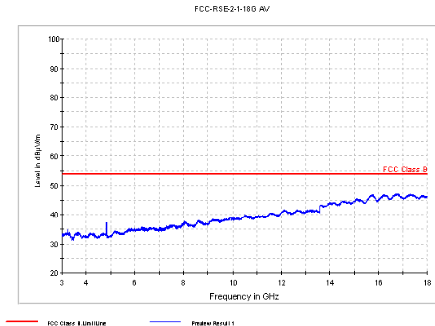
Fig. 64 Radiated Spurious Emission (802.11g, Ch1, 3 GHz-18 GHz)
