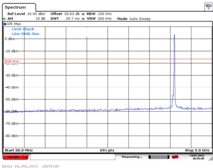
Fig. 32 Conducted Spurious Emission (802.11b, Ch11, 30 MHz-3 GHz)
