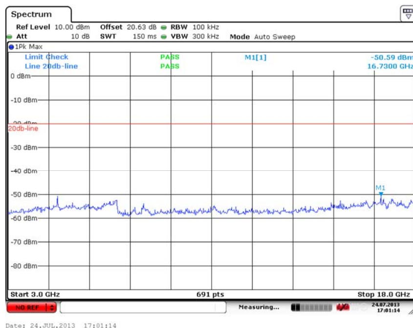
Fig. 36 Conducted Spurious Emission (802.11g, Ch1, 3 GHz-18 GHz)
