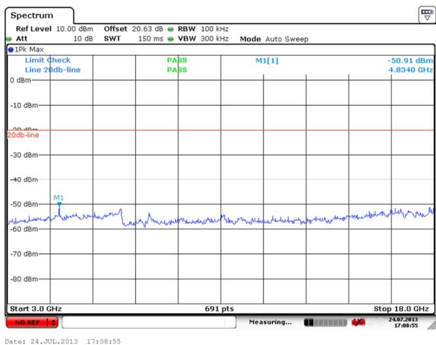
Fig. 45 Conducted Spurious Emission (802.11n-20M, Ch1, 3 GHz-18 GHz)
