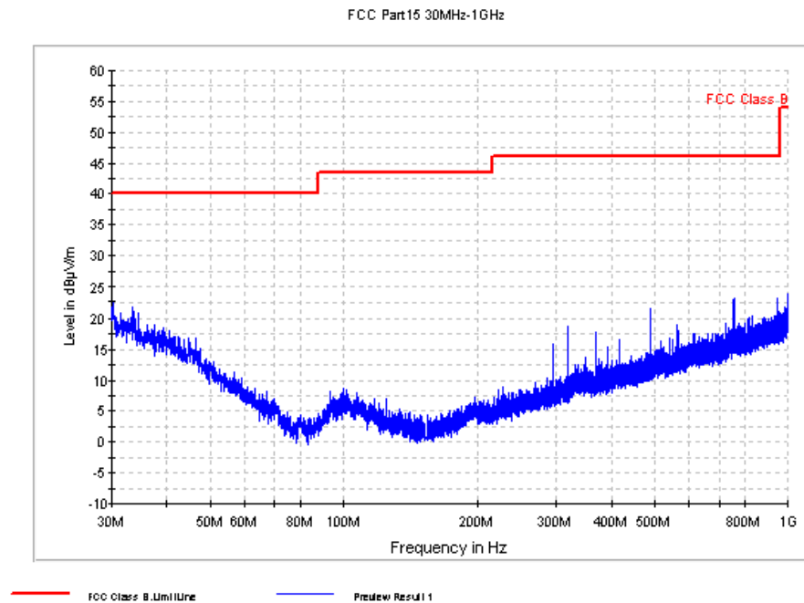
Fig. 59 Radiated Spurious Emission (802.11b, Ch11, 30 MHz-1 GHz)
