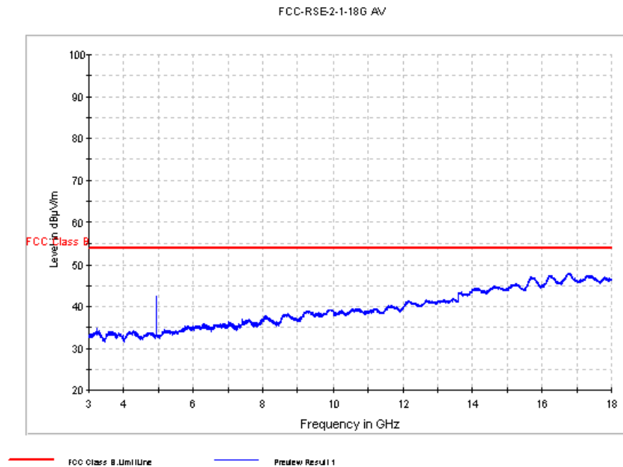
Fig. 61 Radiated Spurious Emission (802.11b, Ch11, 3 GHz-18 GHz)
