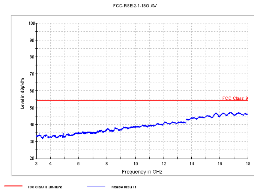
Fig. 76 Radiated Spurious Emission (802.11n-20M, Ch6, 3 GHz-18 GHz)
