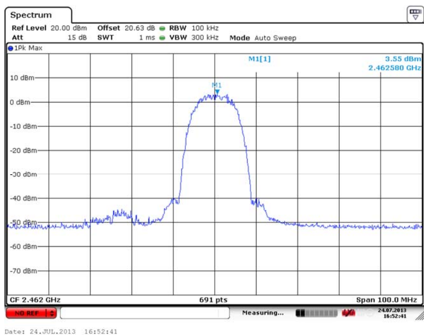
Fig. 31 Conducted Spurious Emission (802.11b, Ch11, Center Frequency)
