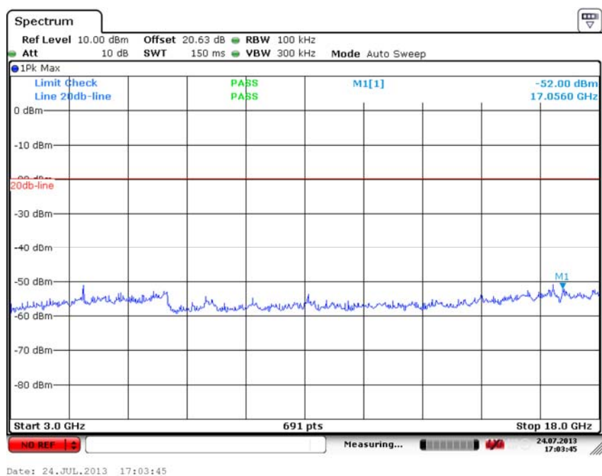
Fig. 39 Conducted Spurious Emission (802.11g, Ch6, 3 GHz-18 GHz)
