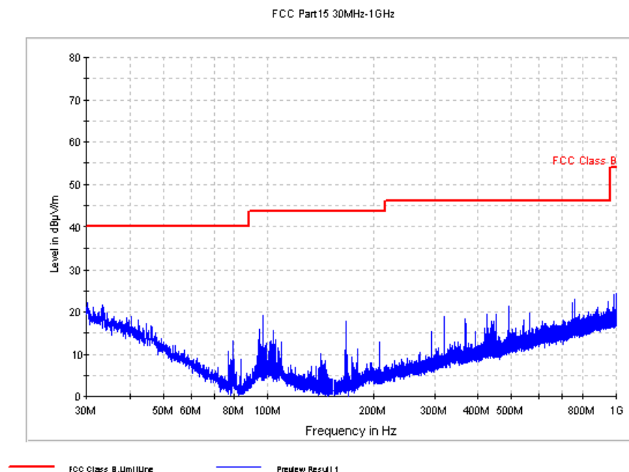
Fig. 68 Radiated Spurious Emission (802.11g, Ch11, 30 MHz-1 GHz)
