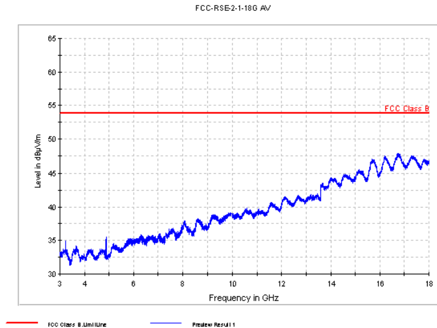
Fig. 67 Radiated Spurious Emission (802.11g, Ch6, 3 GHz-18 GHz)
