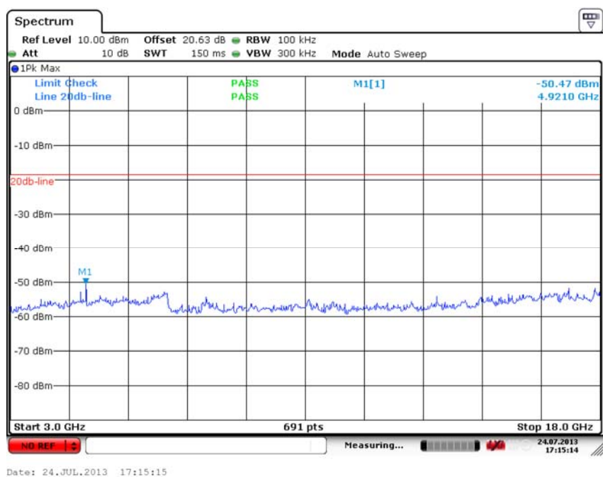
Fig. 51 Conducted Spurious Emission (802.11n-20M, Ch11, 3 GHz-18 GHz)
