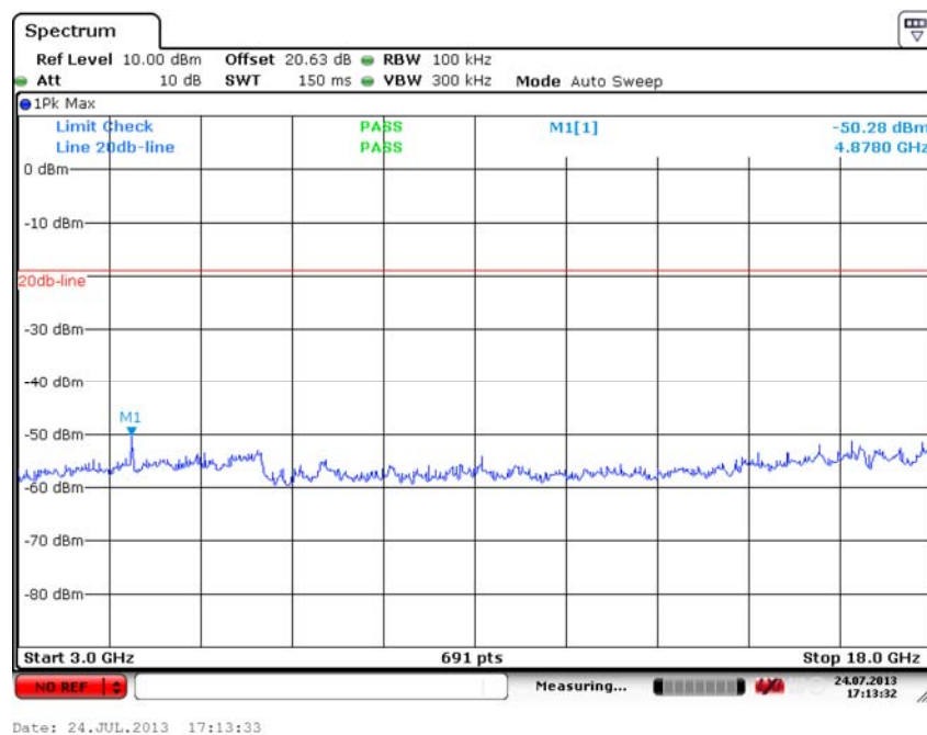
Fig. 48 Conducted Spurious Emission (802.11n-20M, Ch6, 3 GHz-18 GHz)
