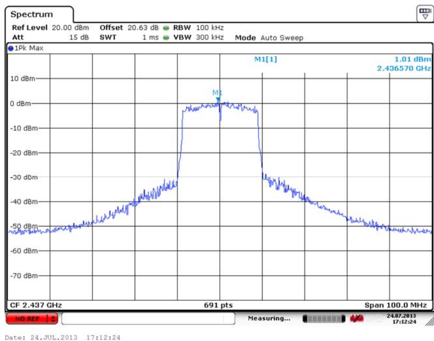
Fig. 46 Conducted Spurious Emission (802.11n-20M, Ch6, Center Frequency)
