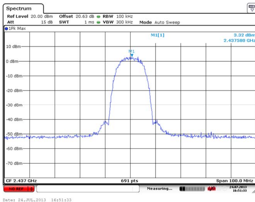
Fig. 28 Conducted Spurious Emission (802.11b, Ch6, Center Frequency)
