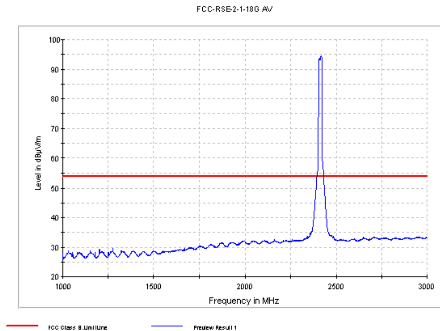
Fig. 63 Radiated Spurious Emission (802.11g, Ch1, 1 GHz-3 GHz)
