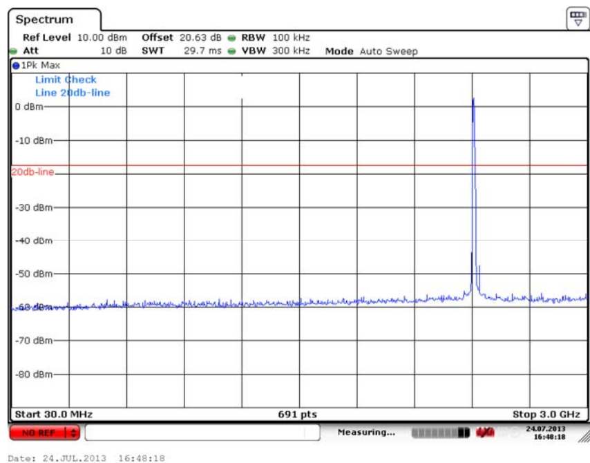
Fig. 26 Conducted Spurious Emission (802.11b, Ch1, 30 MHz-3 GHz)
