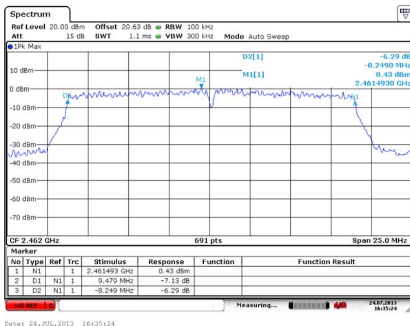
Fig. 18 Occupied 6dB Bandwidth (802.11n-20MHz, Ch 11)
