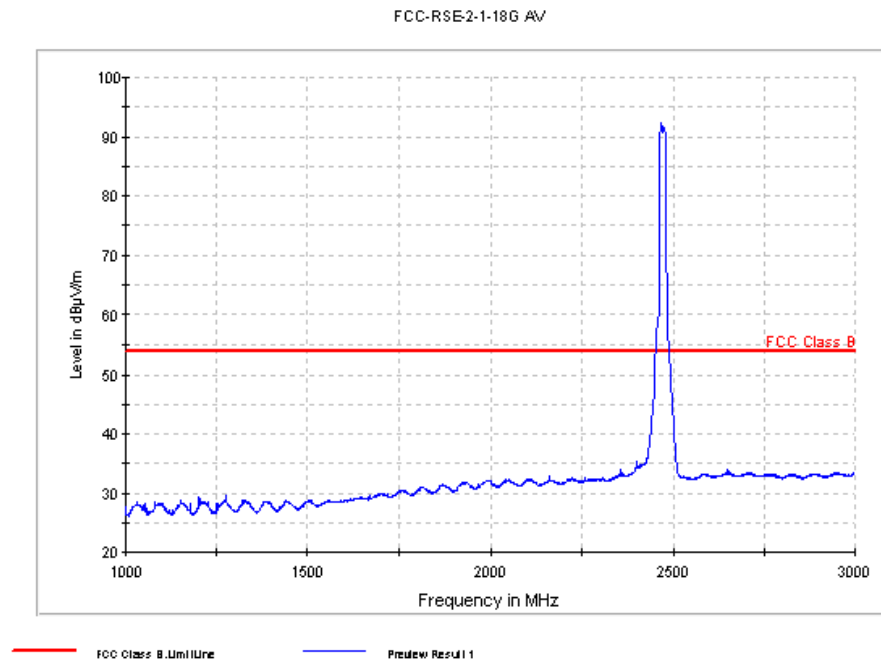
Fig. 69 Radiated Spurious Emission (802.11g, Ch11, 1 GHz-3 GHz)
