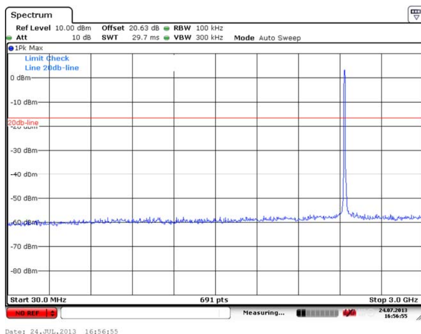
Fig. 29 Conducted Spurious Emission (802.11b, Ch6, 30 MHz-3 GHz)
