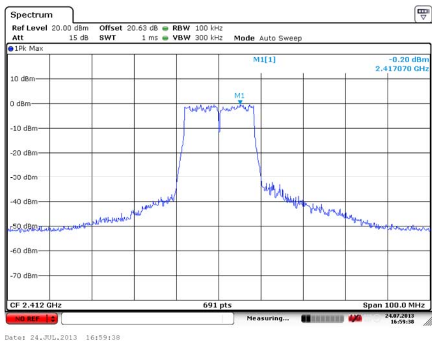
Fig. 34 Conducted Spurious Emission (802.11g, Ch1, Center Frequency)
