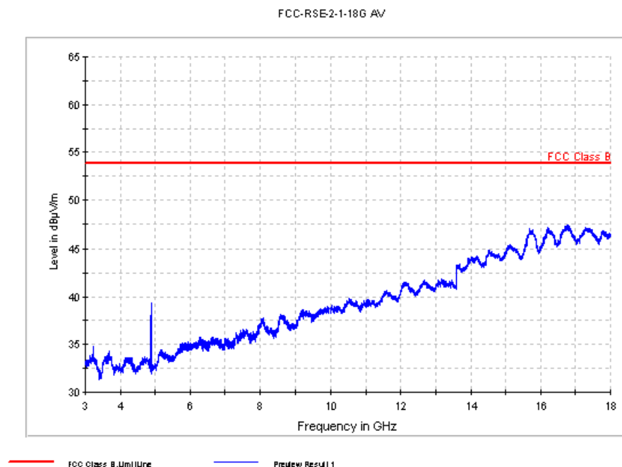
Fig. 58 Radiated Spurious Emission (802.11b, Ch6, 3 GHz-18 GHz)
