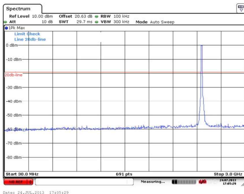
Fig. 41 Conducted Spurious Emission (802.11g, Ch11, 30 MHz-3 GHz)
