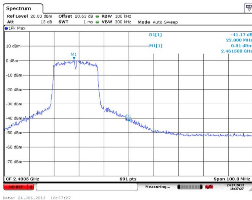
Fig. 24 Band Edges (802.11 n-20MHz, Ch 11)
