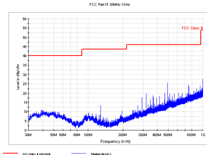
Fig. 62 Radiated Spurious Emission (802.11g, Ch1, 30 MHz-1 GHz)
