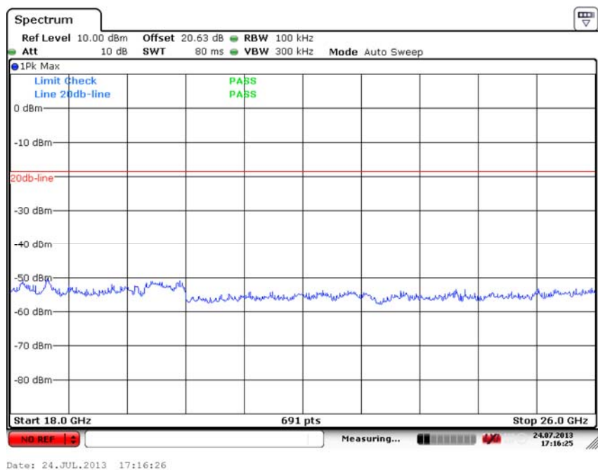
Fig. 52 Conducted Spurious Emission (All channels, 18 GHz-26 GHz)
