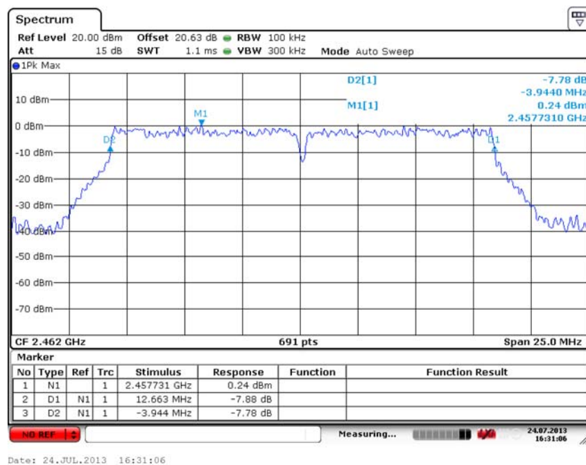
Fig. 15 Occupied 6dB Bandwidth (802.11g, Ch 11)
