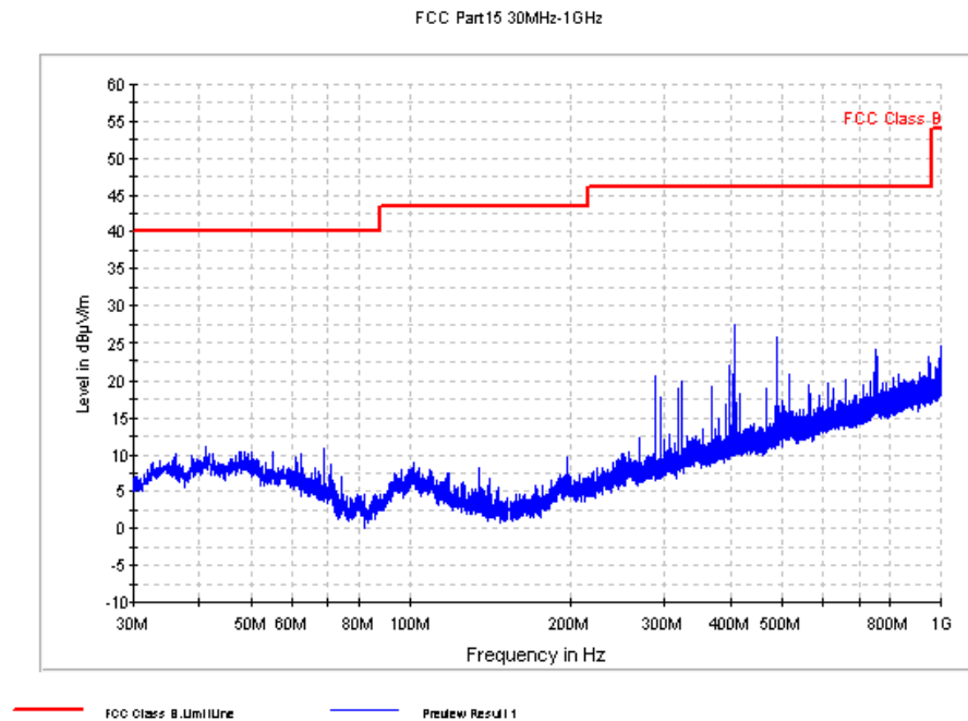
Fig. 53 Radiated Spurious Emission (802.11b, Ch1, 30 MHz-1 GHz)
