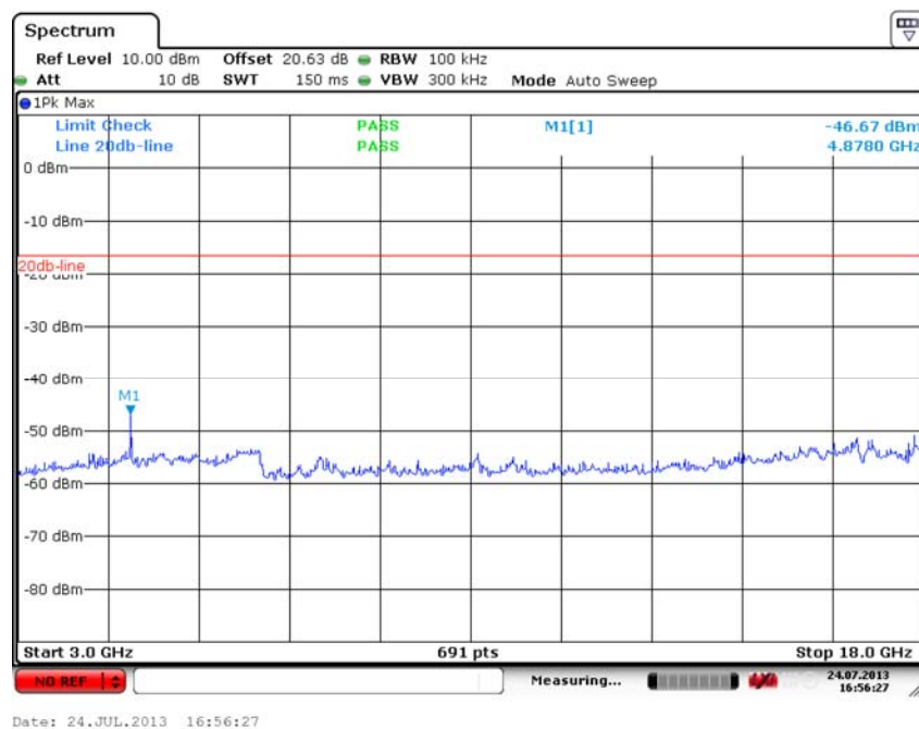
Fig. 30 Conducted Spurious Emission (802.11b, Ch6, 3 GHz-18 GHz)
