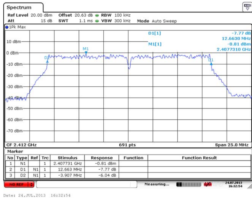
Fig. 13 Occupied 6dB Bandwidth (802.11g, Ch 1)
