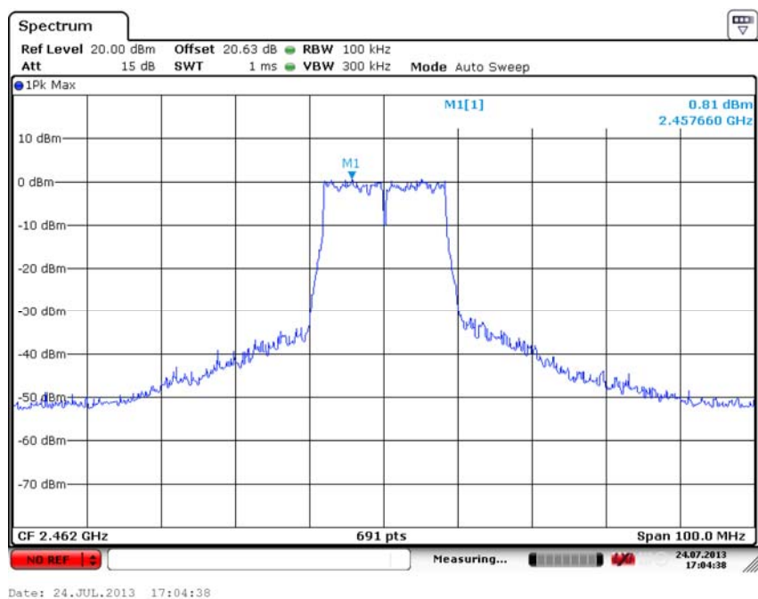
Fig. 40 Conducted Spurious Emission (802.11g, Ch11, Center Frequency)
