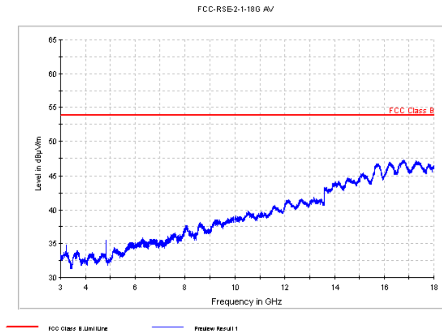
Fig. 55 Radiated Spurious Emission (802.11b, Ch1, 3 GHz-18 GHz)
