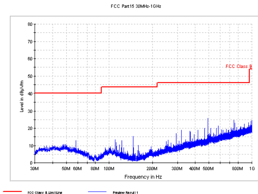
Fig. 62 Radiated Spurious Emission (8DPSK, Ch39, 30 MHz ~1 GHz)
