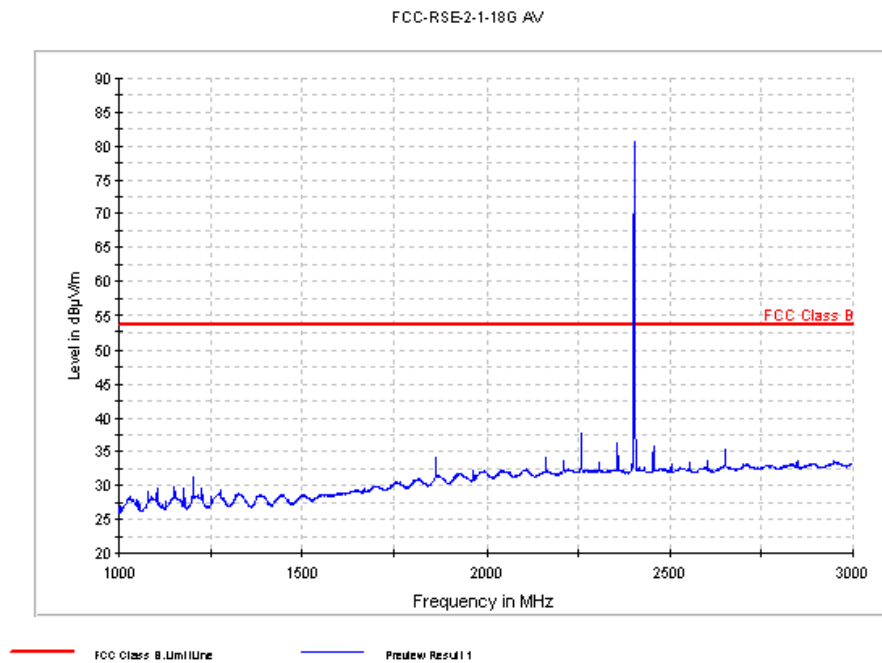
Fig. 42 Radiated Spurious Emission (GFSK, Ch0, 1 GHz ~3 GHz)
