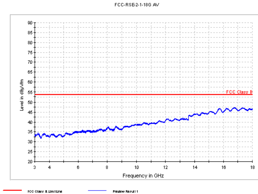
Fig. 43 Radiated Spurious Emission (GFSK, Ch0, 3 GHz ~18 GHz)
