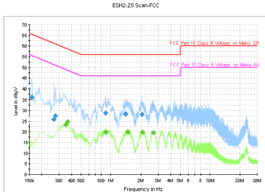
Fig. 87 AC Power line Conducted Emission (GFSK, Ch39)
