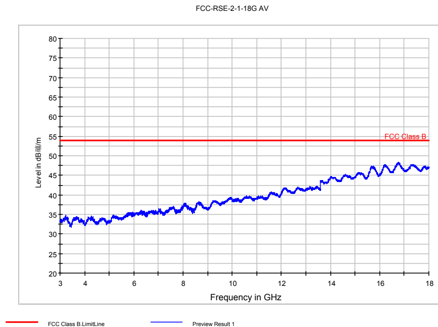
Fig. 55 Radiated Spurious Emission ( \pi/4 DQPSK, Ch39, 3 GHz ~18 GHz)
