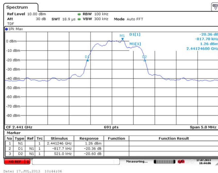
Fig. 71 Occupied 20dB Bandwidth (8DPSK, Ch 39)
