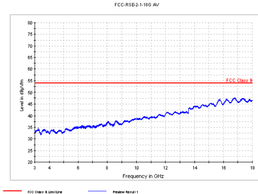
Fig. 61 Radiated Spurious Emission (8DPSK, Ch0, 3 GHz ~18 GHz)
