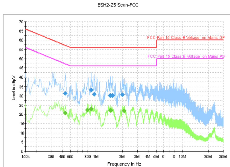
Fig. 89 AC Power line Conducted Emission (8DPSK, Ch39)
