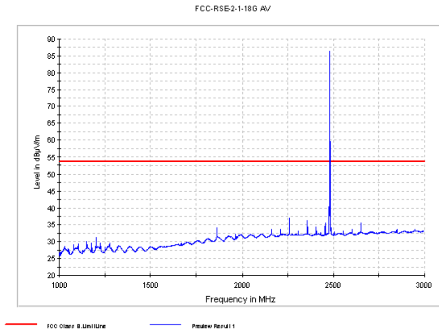
Fig. 48 Radiated Spurious Emission (GFSK, Ch78, 1 GHz ~3 GHz)
