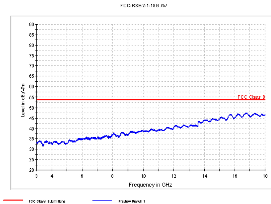
Fig. 49 Radiated Spurious Emission (GFSK, Ch78, 3 GHz ~18 GHz)
