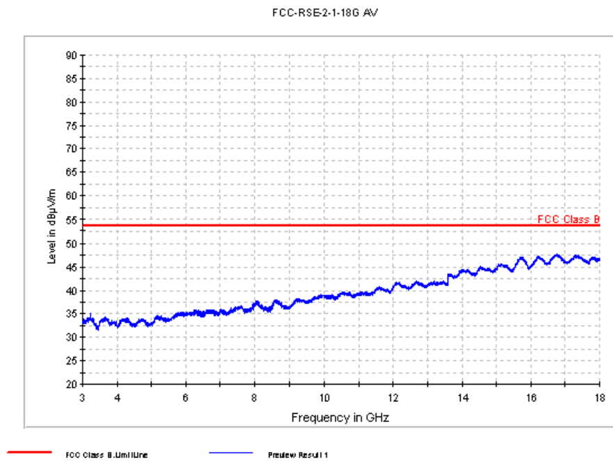
Fig. 67 Radiated Spurious Emission (8DPSK, Ch78, 3 GHz ~18 GHz)
