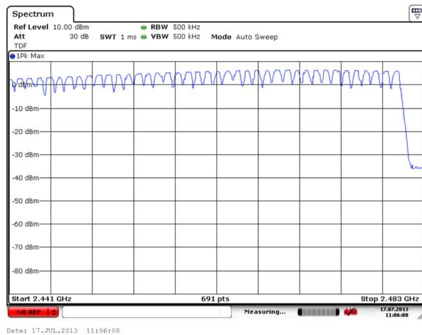
Fig. 79 Hopping channel ch39~78 (GFSK, Ch39)
