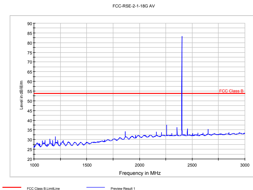
Fig. 51 Radiated Spurious Emission ( \pi/4 DQPSK, Ch0, 1 GHz ~3 GHz)
