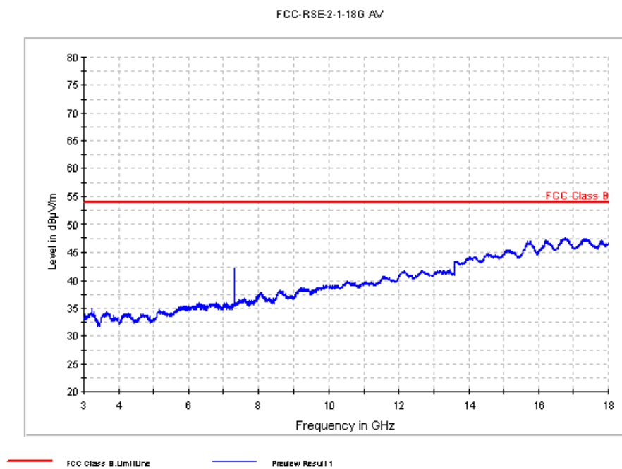
Fig. 46 Radiated Spurious Emission (GFSK, Ch39, 3 GHz ~18 GHz)
