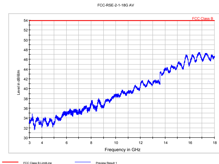
Fig. 52 Radiated Spurious Emission ( \pi/4 DQPSK, Ch0, 3 GHz ~18 GHz)
