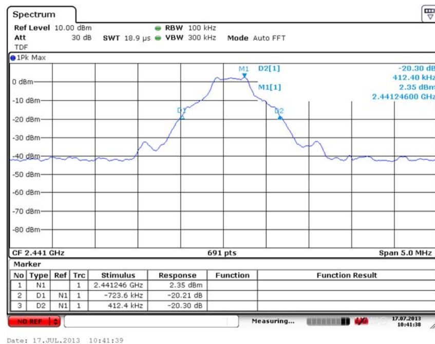
Fig. 69 Occupied 20dB Bandwidth (GFSK, Ch 39)
