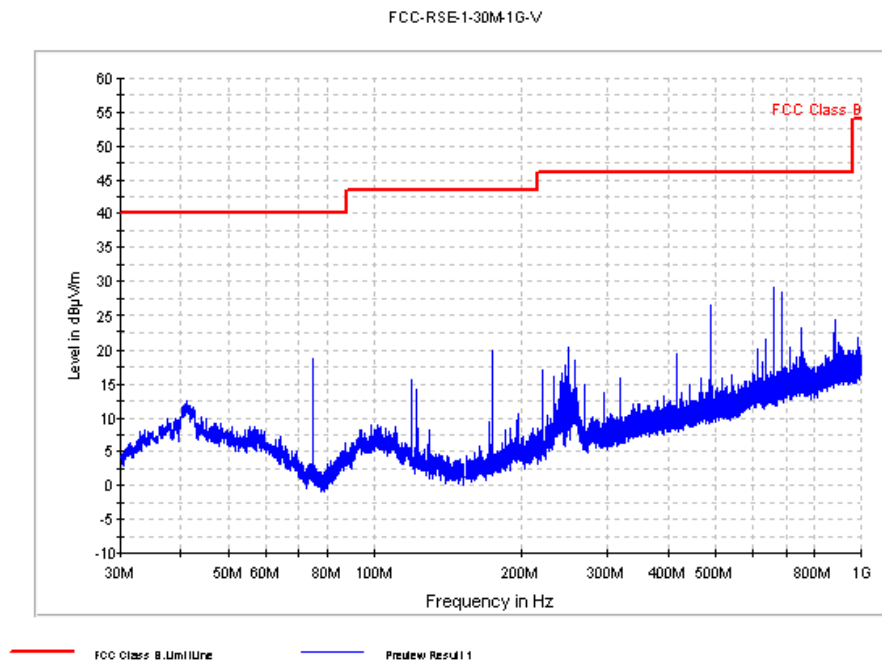
Fig. 44 Radiated Spurious Emission (GFSK, Ch39, 30 MHz ~1 GHz)
