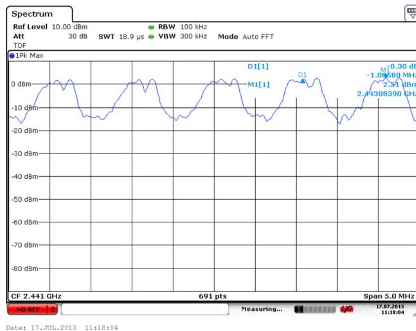
Fig. 84 Carrier Frequency Separation (GFSK, Ch39)
