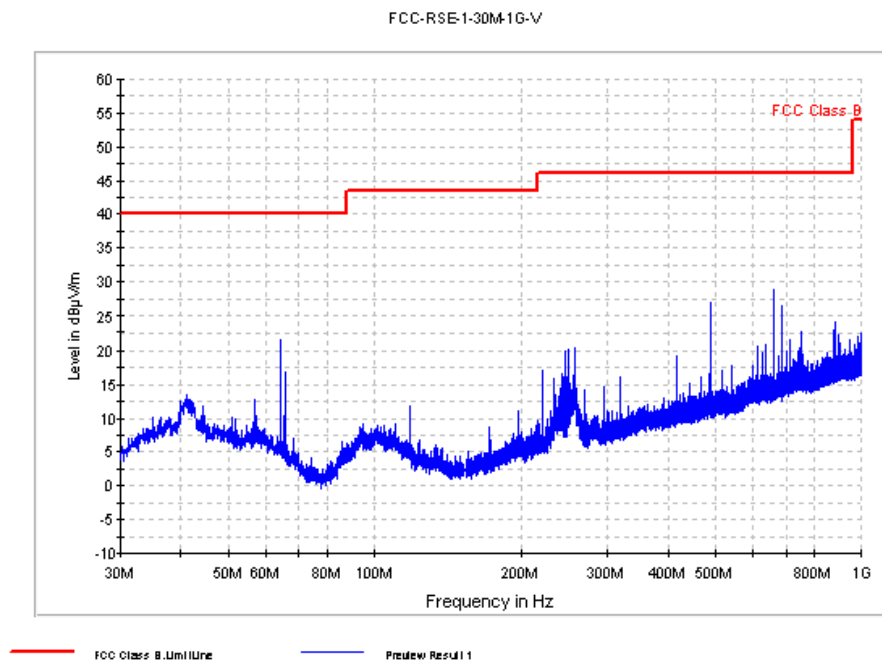
Fig. 41 Radiated Spurious Emission (GFSK, Ch0, 30 MHz ~1 GHz)
