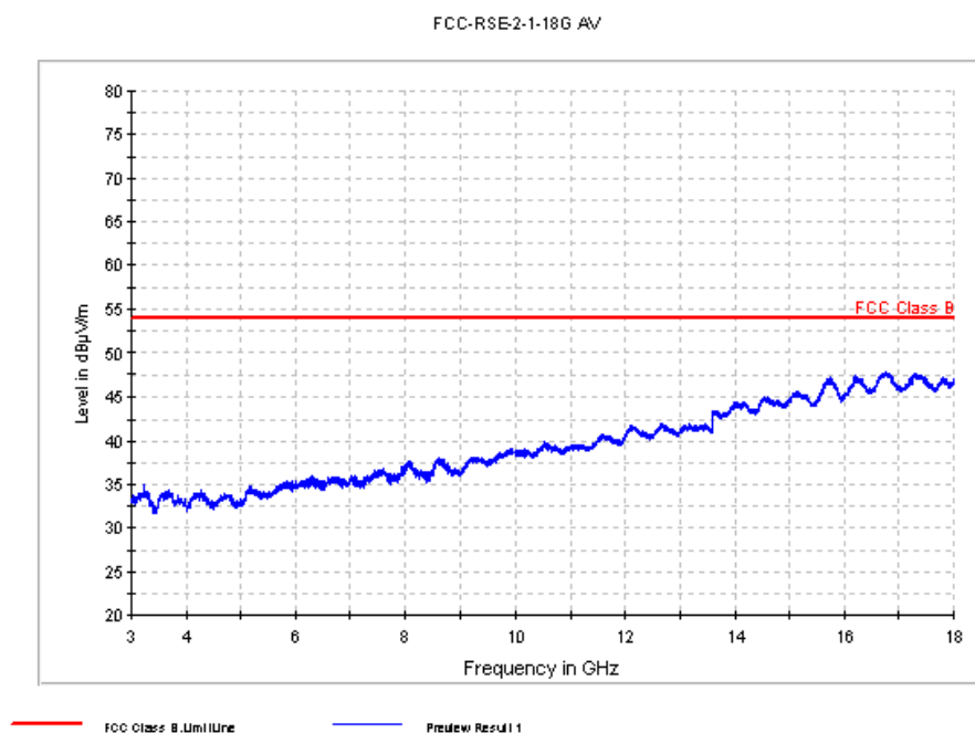
Fig. 58 Radiated Spurious Emission ( \pi/4 DQPSK, Ch78, 3 GHz ~18 GHz)
