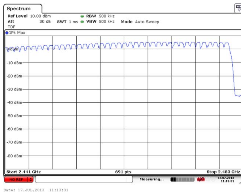
Fig. 83 Hopping channel ch39~78 (8DPSK, Ch39)
