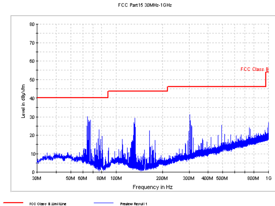
Fig. 59 Radiated Spurious Emission (8DPSK, Ch0, 30 MHz ~1 GHz)
