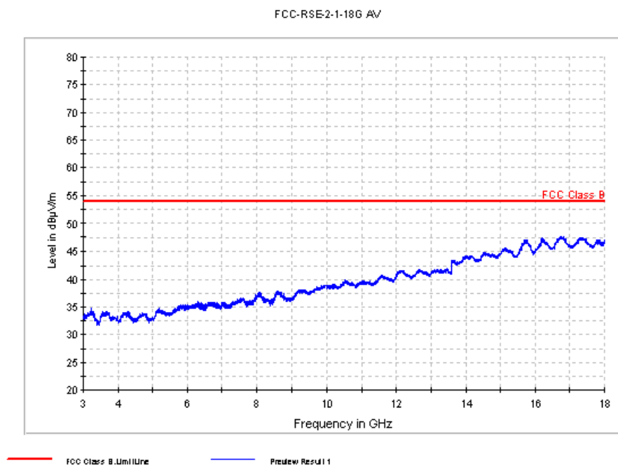
Fig. 64 Radiated Spurious Emission (8DPSK, Ch0, 3 GHz ~18 GHz)
