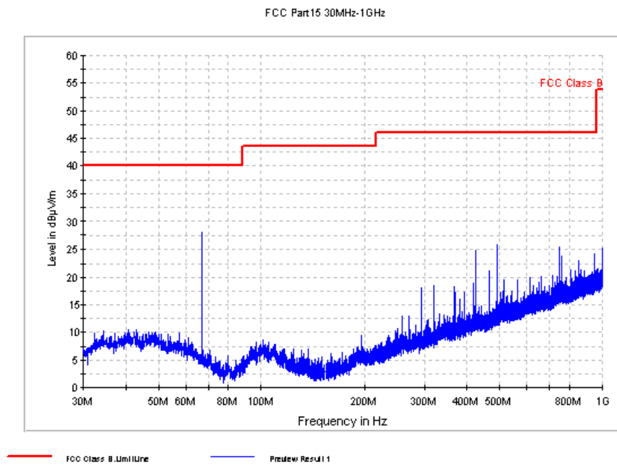
Fig. 65 Radiated Spurious Emission (8DPSK, Ch78, 30 MHz ~1 GHz)
