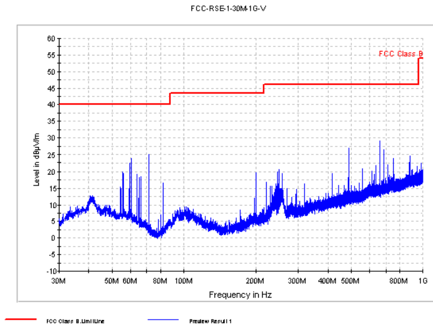
Fig. 50 Radiated Spurious Emission ( \pi/4 DQPSK, Ch0, 30 MHz ~1 GHz)
