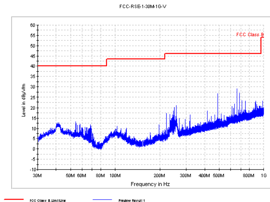
Fig. 56 Radiated Spurious Emission ( \pi/4 DQPSK, Ch78, 30 MHz ~1 GHz)
