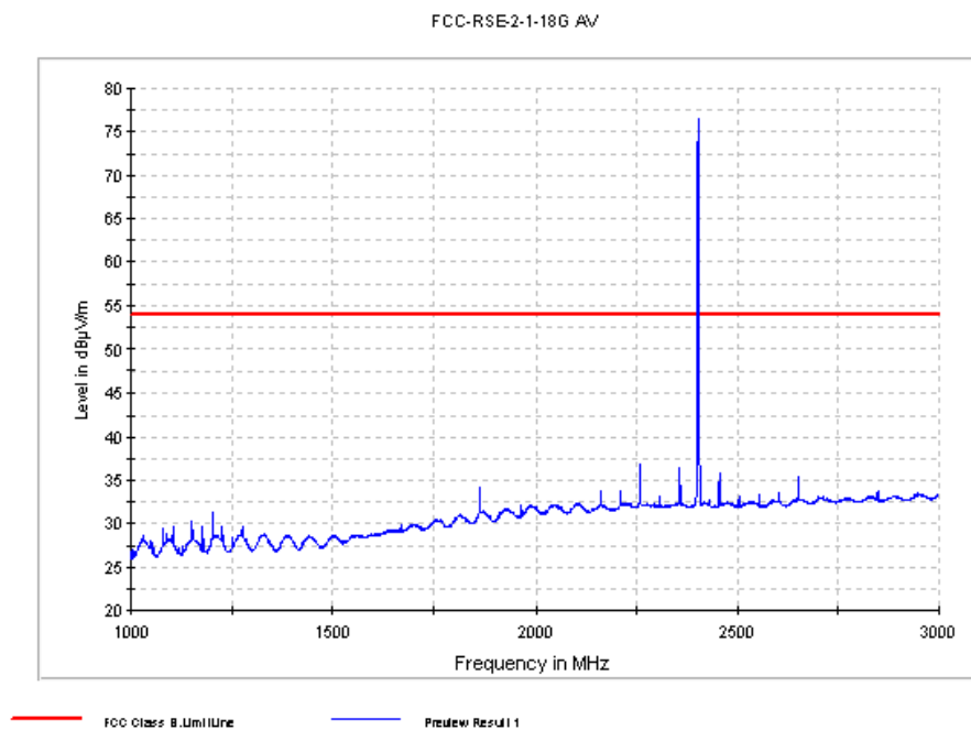
Fig. 60 Radiated Spurious Emission (8DPSK, Ch0, 1 GHz ~3 GHz)
