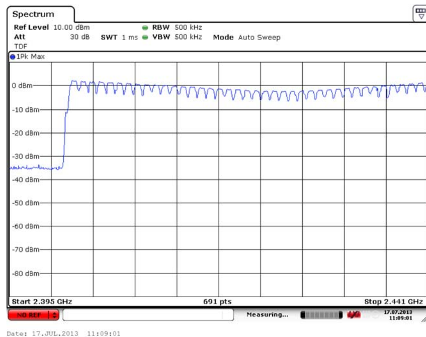
Fig. 80 Hopping channel ch0~39 ( \pi/4 DQPSK, Ch39)
