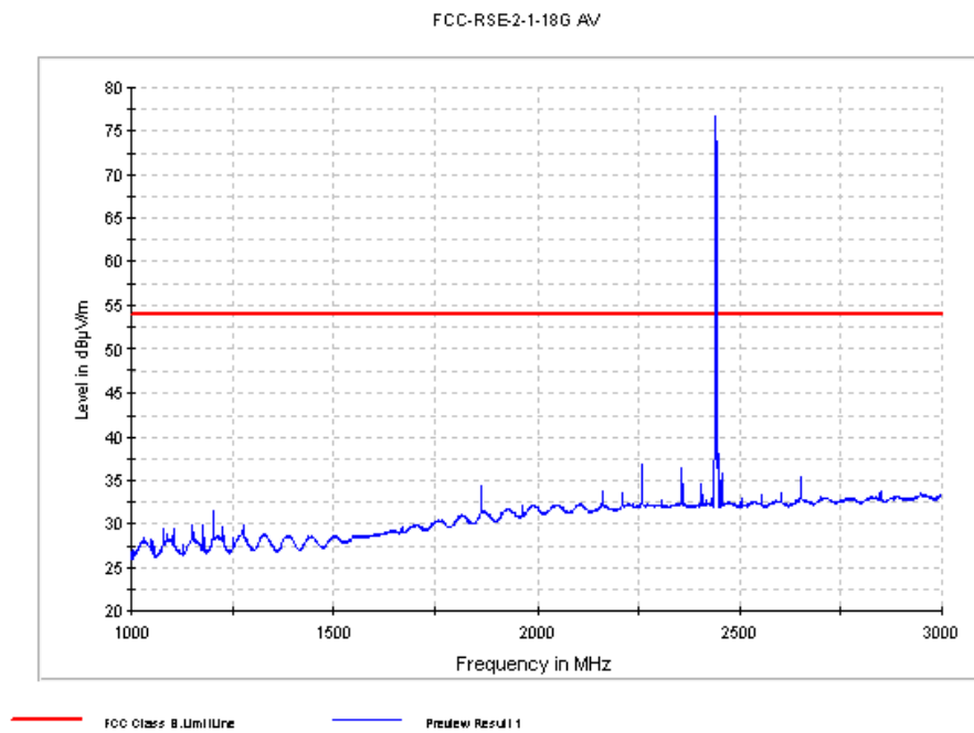
Fig. 63 Radiated Spurious Emission (8DPSK, Ch0, 1 GHz ~3 GHz)
