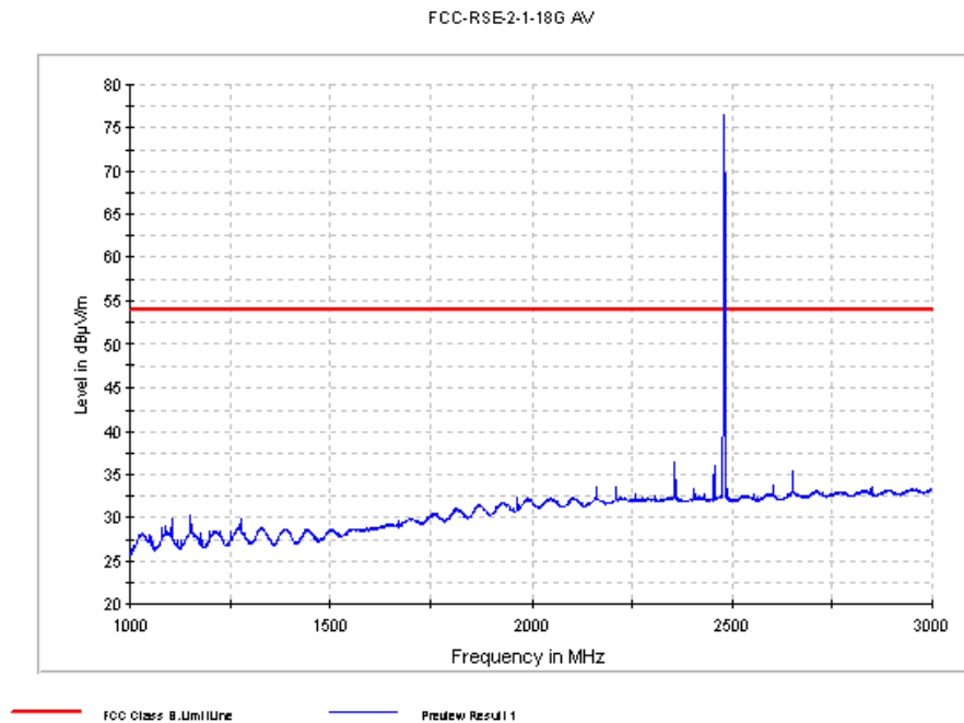
Fig. 57 Radiated Spurious Emission ( \pi/4 DQPSK, Ch78, 1 GHz ~3 GHz)
