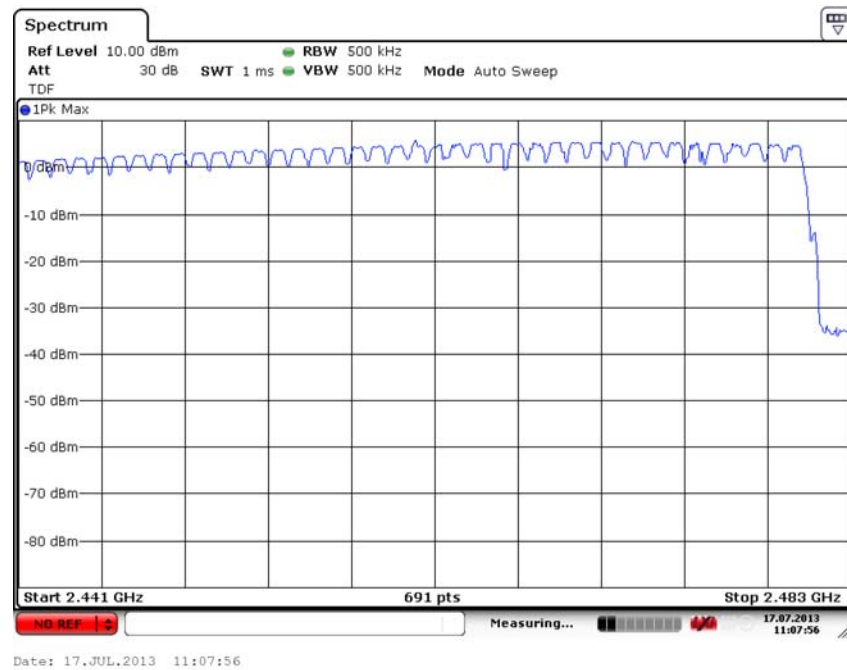
Fig. 81 Hopping channel ch39~78 ( \pi/4 DQPSK, Ch39)
