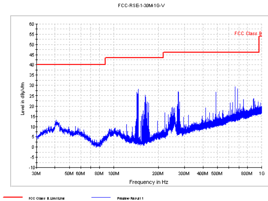
Fig. 47 Radiated Spurious Emission (GFSK, Ch78, 30 MHz ~1 GHz)
