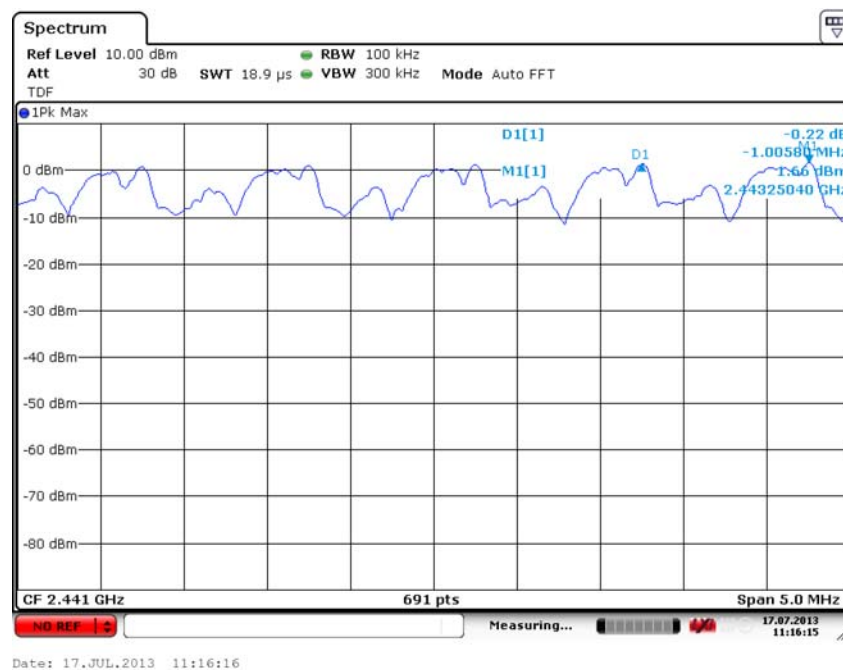
Fig. 86 Carrier Frequency Separation (8DPSK, Ch39)
