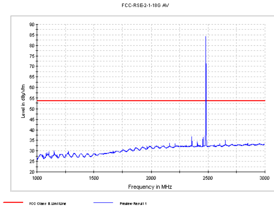
Fig. 66 Radiated Spurious Emission (8DPSK, Ch78, 1 GHz ~3 GHz)
