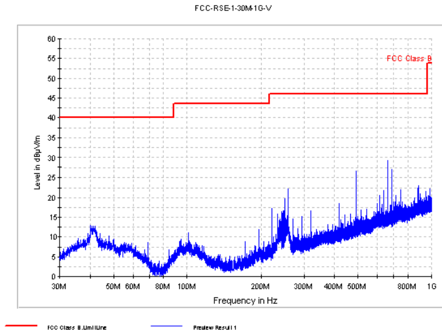
Fig. 53 Radiated Spurious Emission ( \pi/4 DQPSK, Ch39, 30 MHz ~1 GHz)
