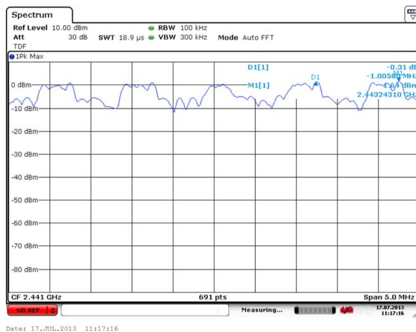
Fig. 85 Carrier Frequency Separation ( \pi/4 DQPSK, Ch39)
