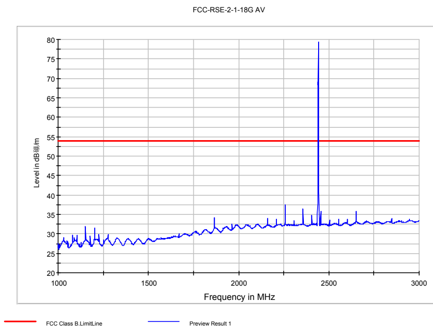
Fig. 54 Radiated Spurious Emission ( \pi/4 DQPSK, Ch39, 1 GHz ~3 GHz)
