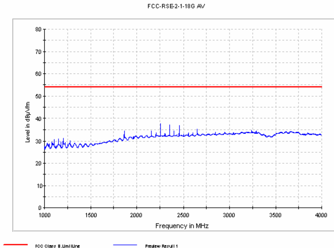
Figure A.2 Radiated Emission from 1GHz to 4GHz (Set.1, Charging mode)
