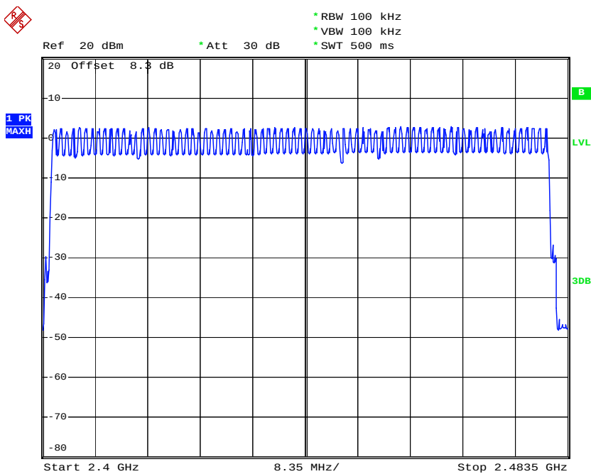
Number of Hopping Channel Plot on Channel 00 - 78
