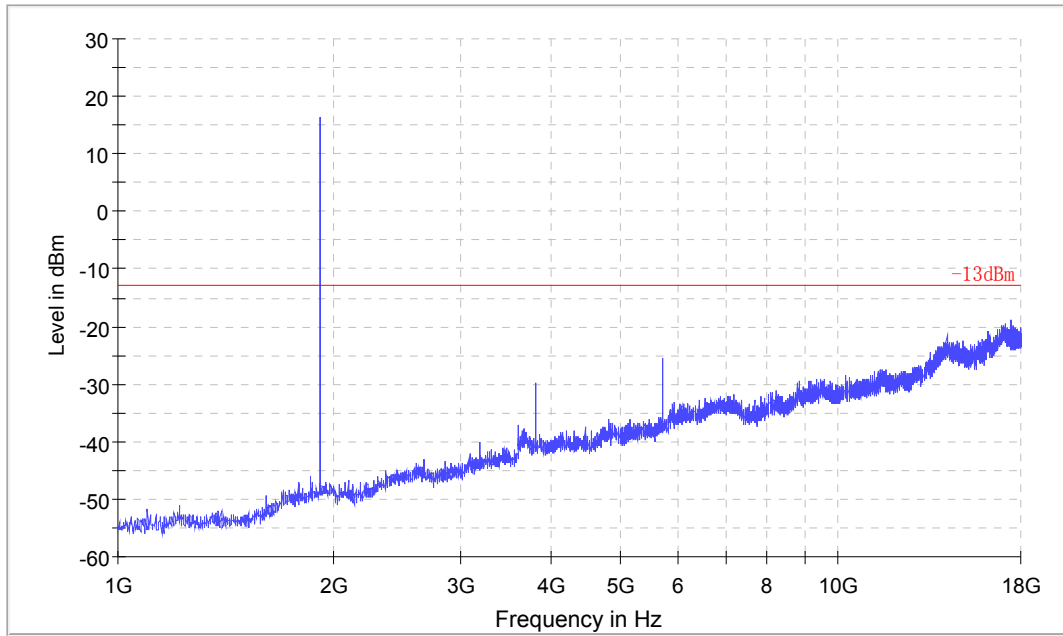
above 1GHz
