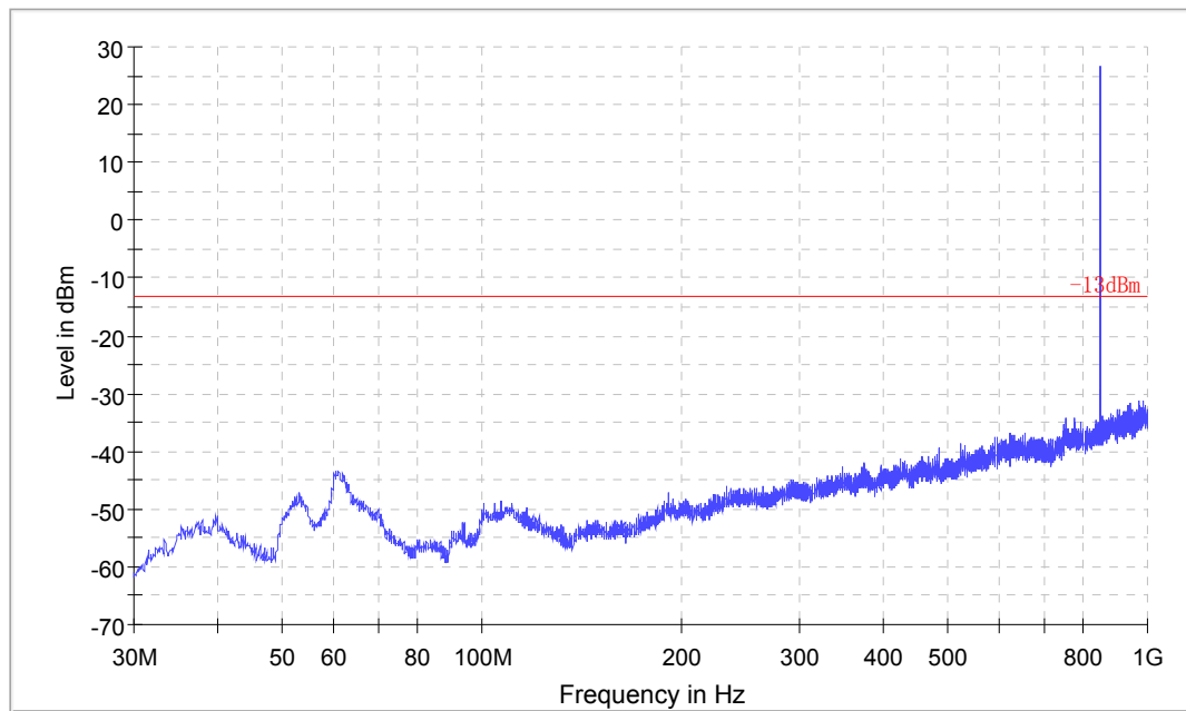
below 1GHz
