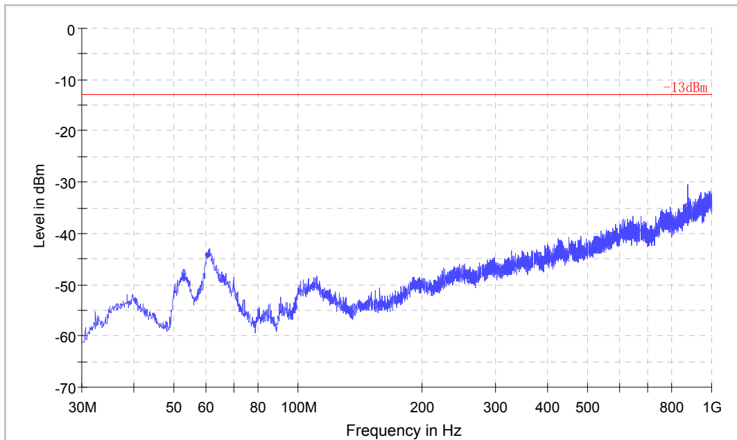
below 1GHz
