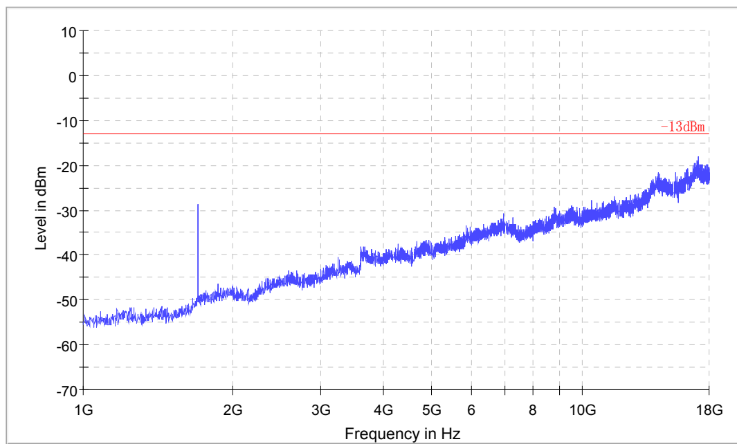
above 1GHz
