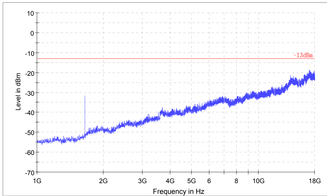
above 1GHz
