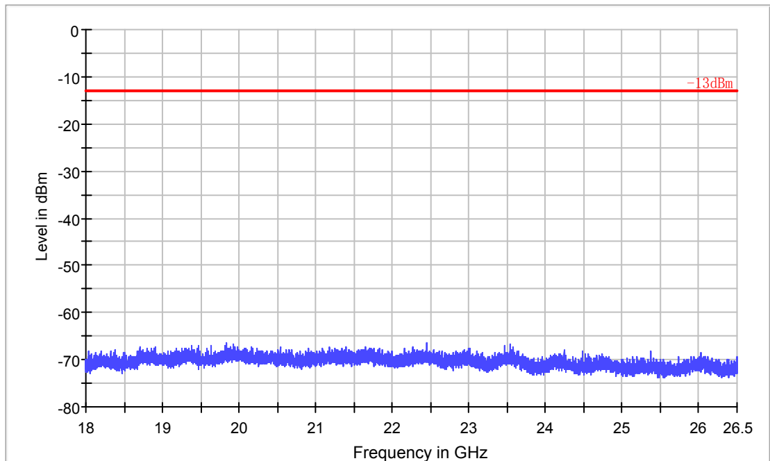
Copy of Spurious emission 18-26.5GHz
