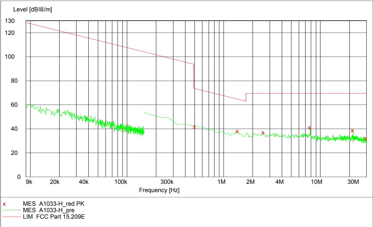
Radiated Emission Plot between 9 kHz ~ 30MHz (Horizontal)
