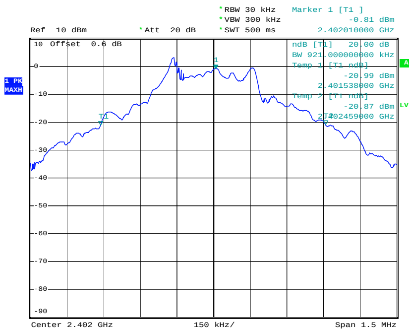
20 dB Bandwidth Plot on Channel 00
