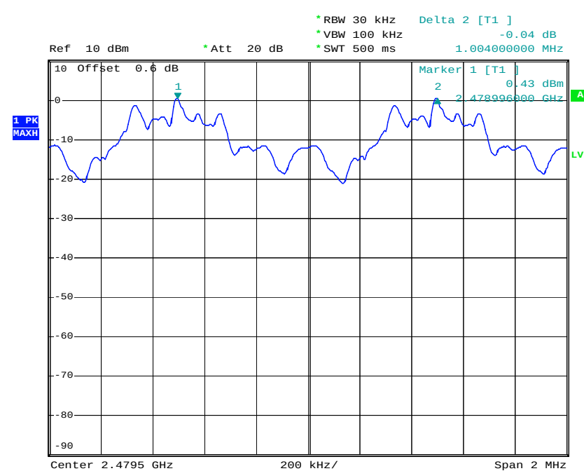
Channel Separation Plot on Channel 77 - 78
