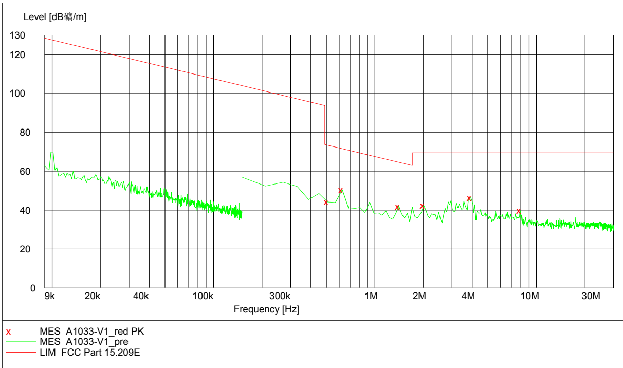
Radiated Emission Plot between 9 kHz ~ 30MHz (Vertical)
