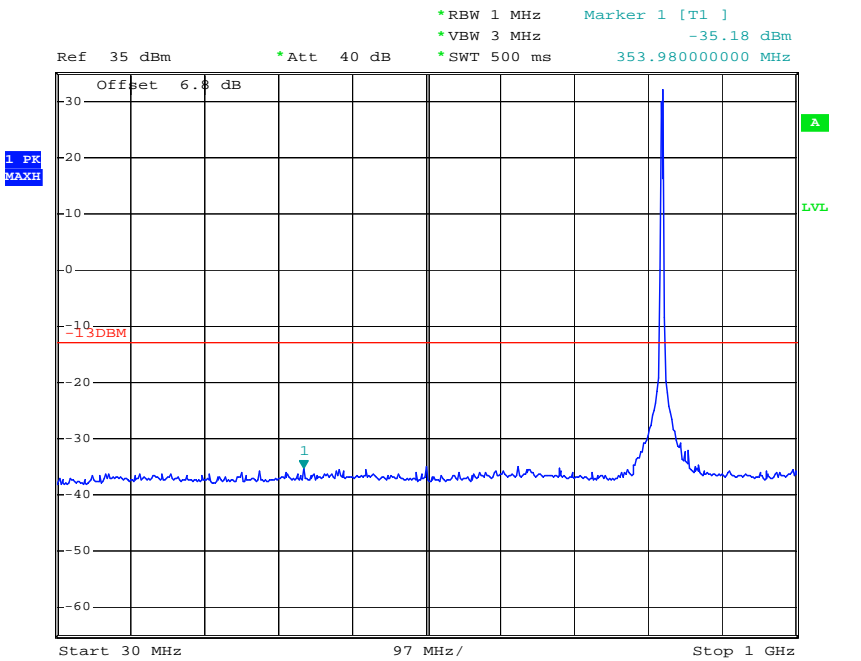
Conducted Emission Plot between 30MHz ~ 1GHz
