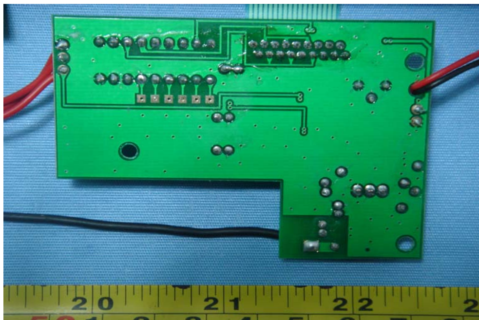
PCB1-Back View
