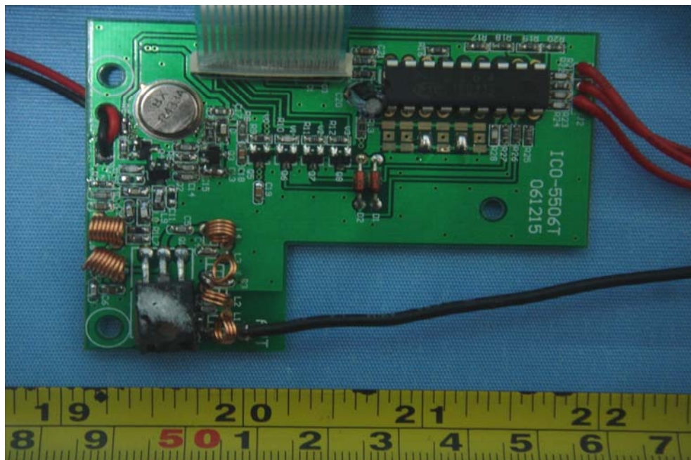
PCB1-Front View
