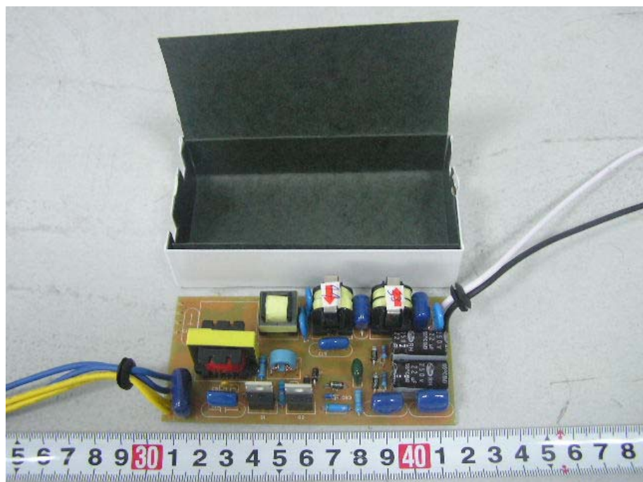
EUT-Inside View
