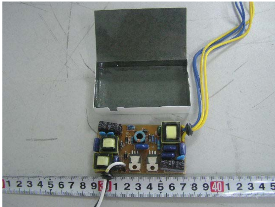
EUT-Inside View
