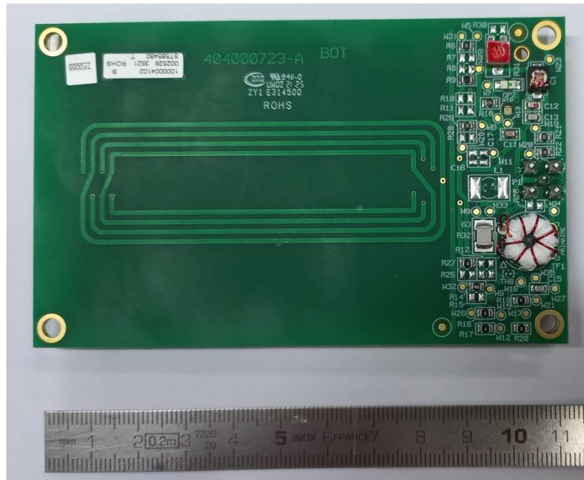
CLess unstacker V2 antenna Top (ELM_1000042017)
