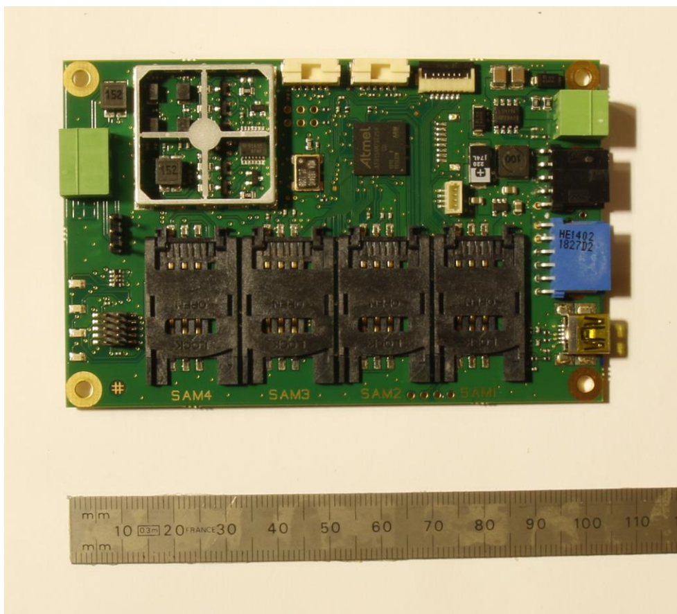
CLESS reader board Top without shielding
