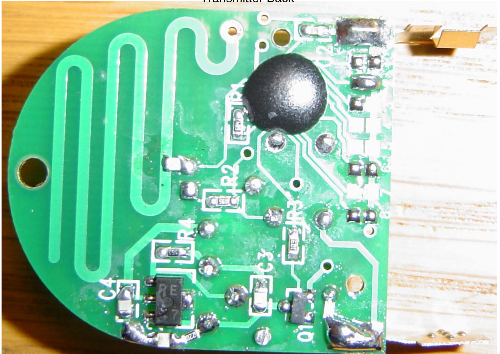
Transmitter Back
