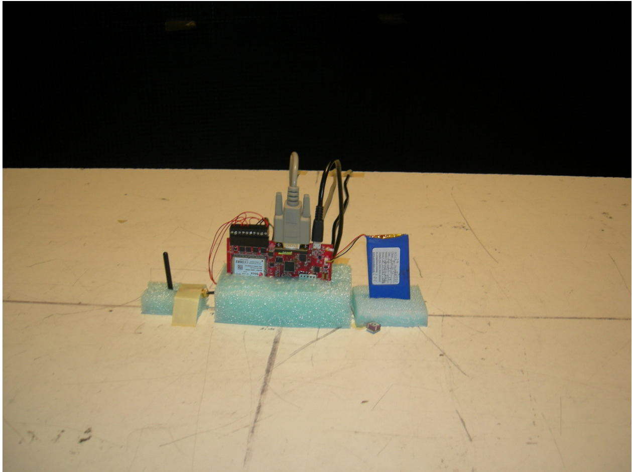
Figure 5: Radiated Emissions – Whip Antenna YPOS
