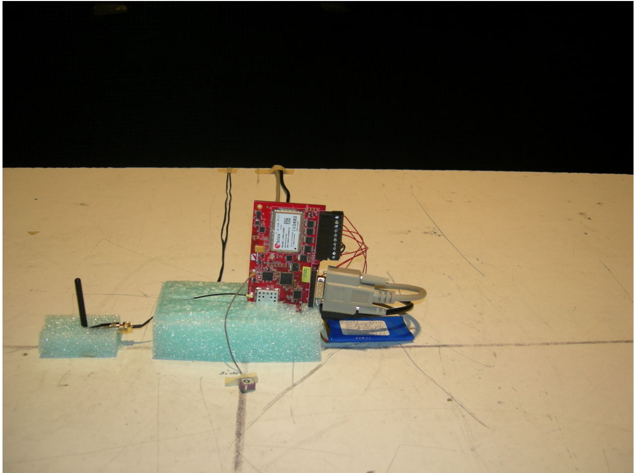
Figure 6: Radiated Emissions – Whip Antenna ZPOS
