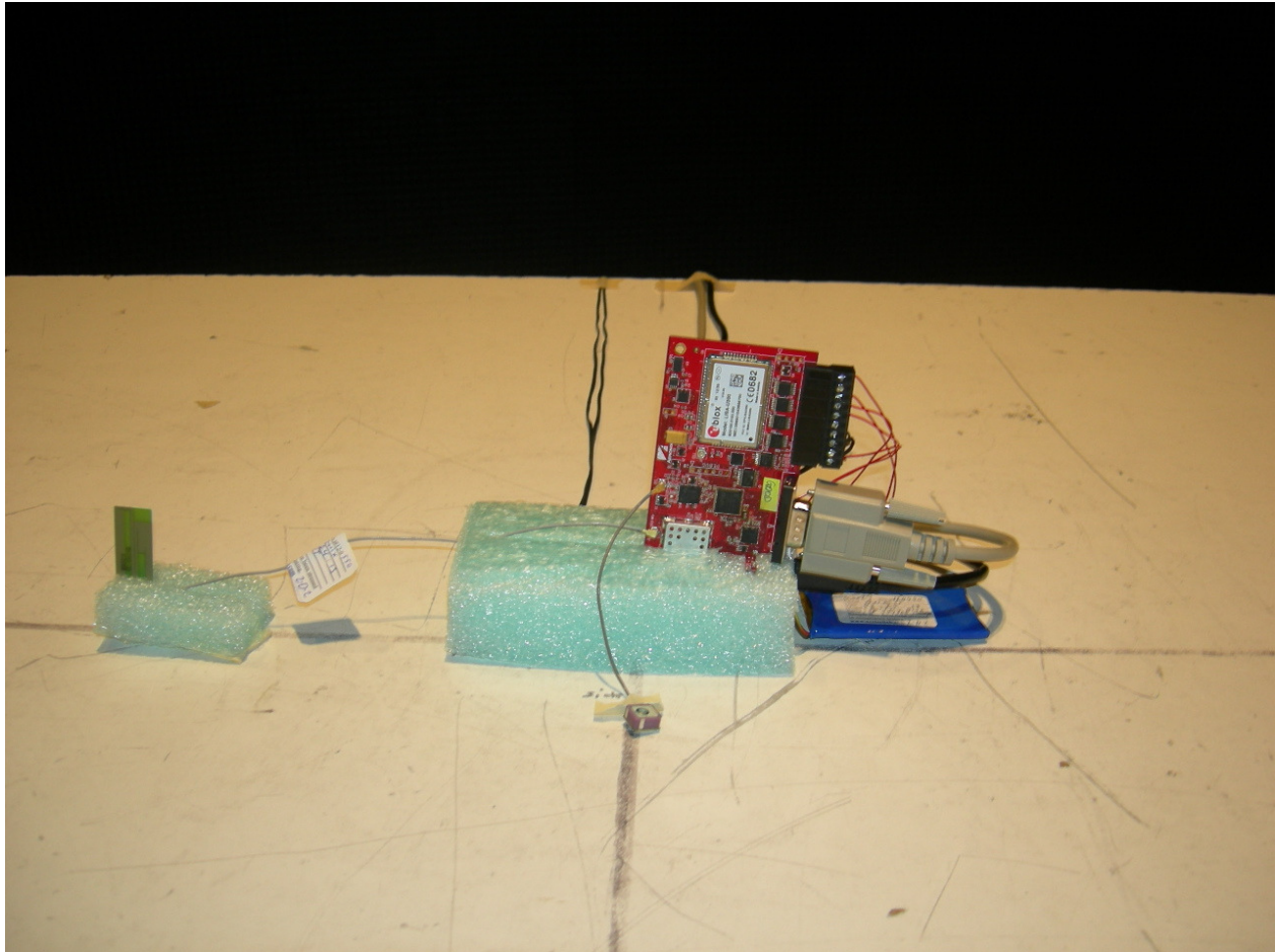
Figure 3: Radiated Emissions – PCB Antenna ZPOS
