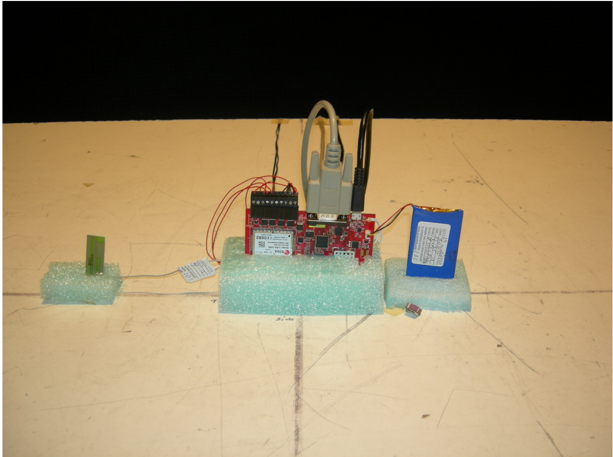
Figure 2: Radiated Emissions – PCB Antenna YPOS
