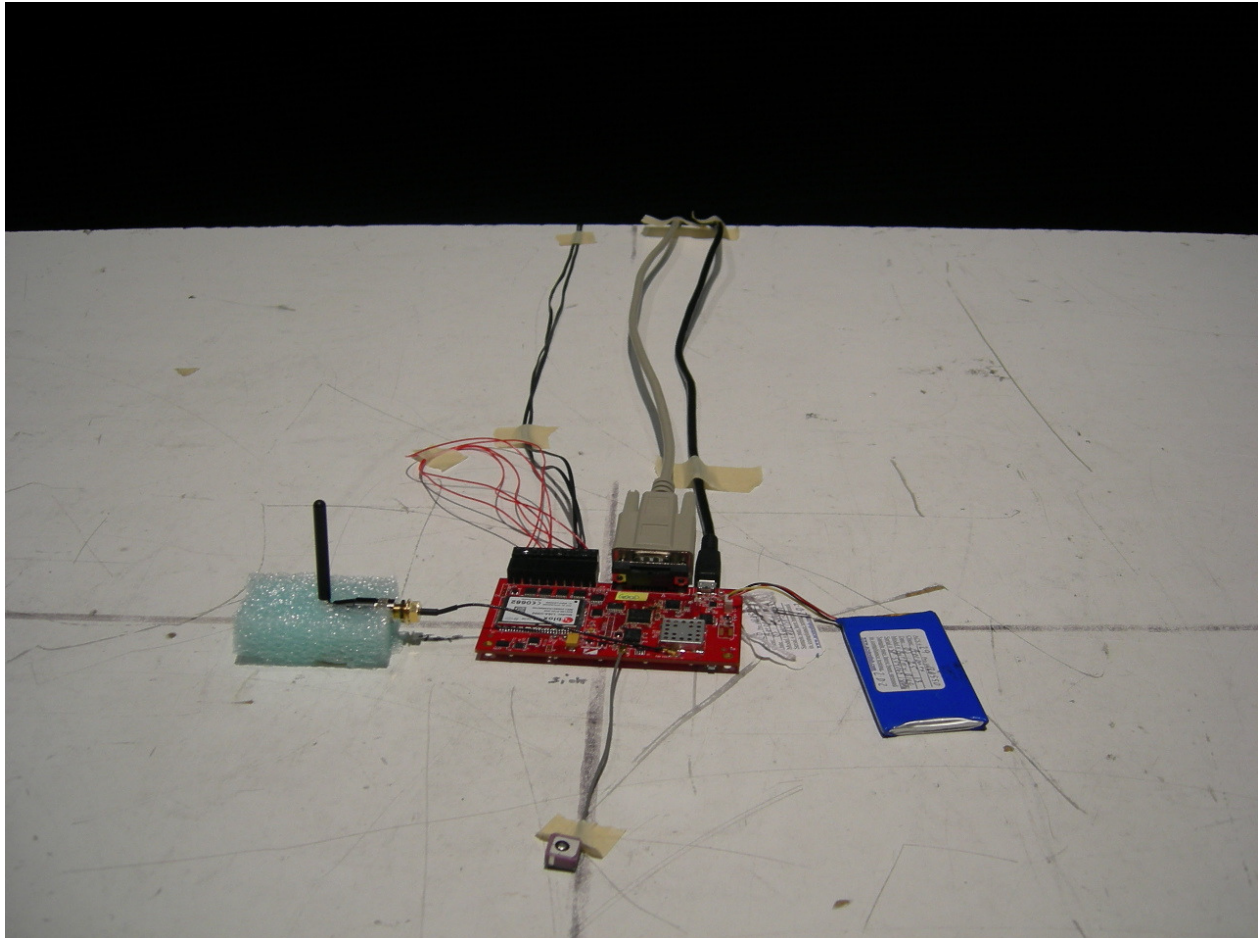
Figure 4: Radiated Emissions – Whip Antenna XPOS
