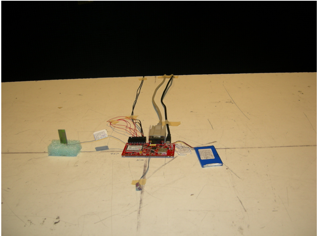
Figure 1: Radiated Emissions – PCB Antenna XPOS
