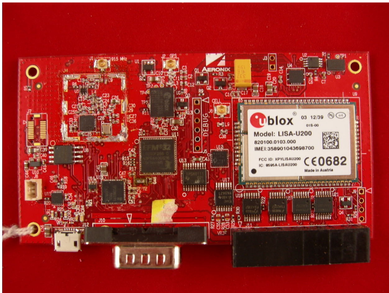
Figure 1: PCB Top (No Shields)
