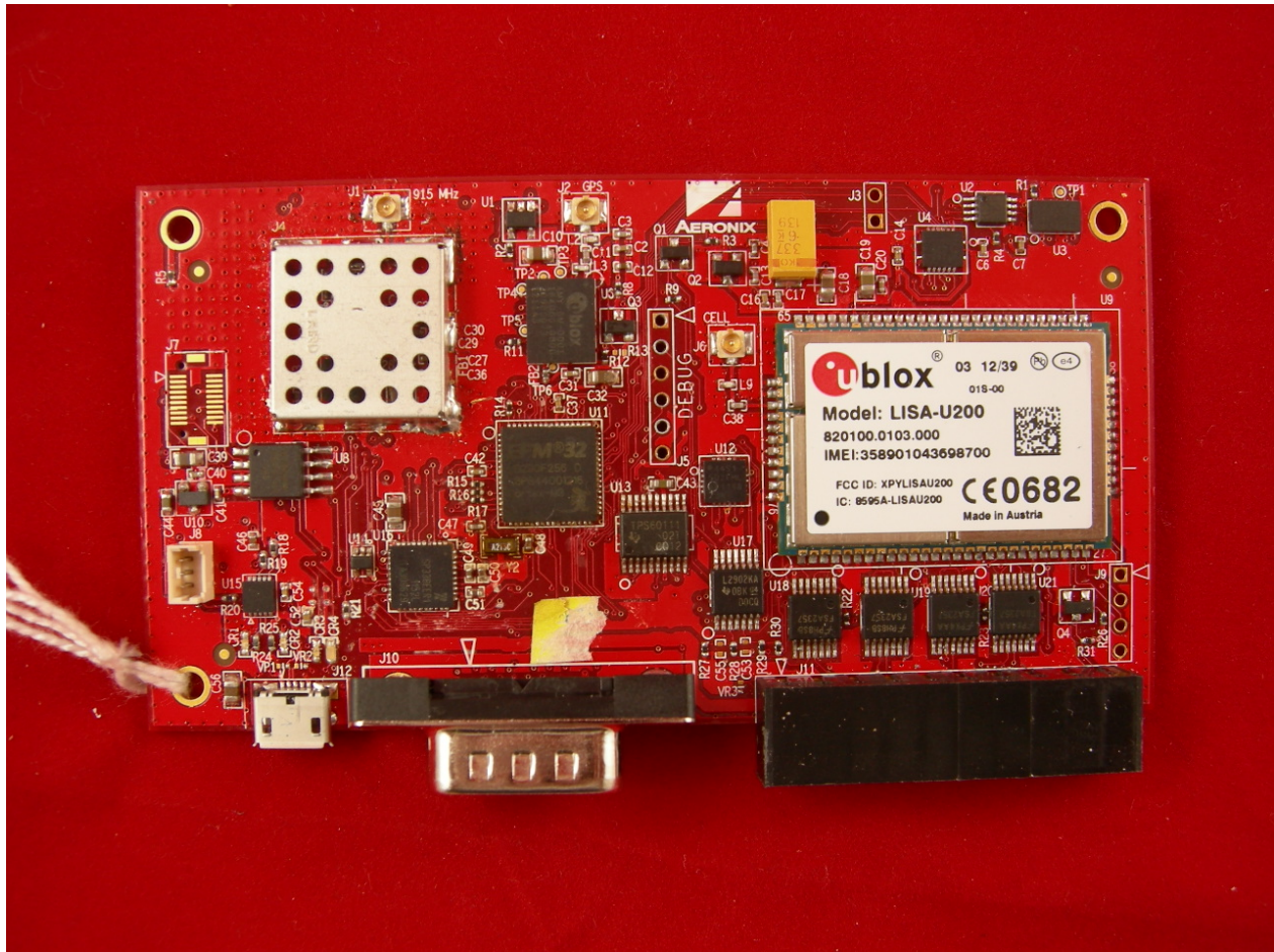
Figure 1: PCB Top
