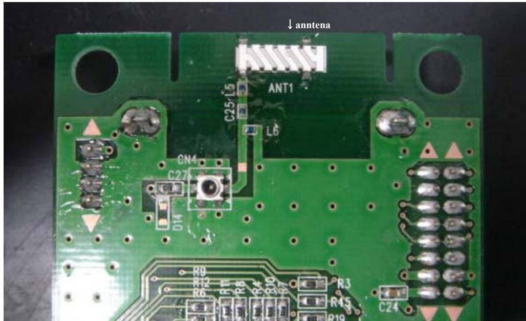
Antenna part
