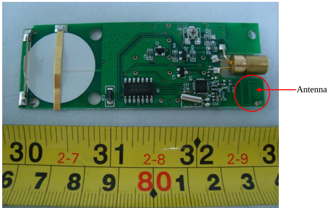
EUT – RF Board Bottom Components View
