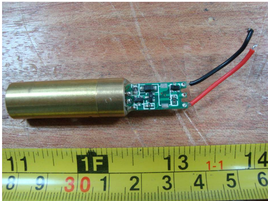
EUT – Laser Transmitter Board Top View
