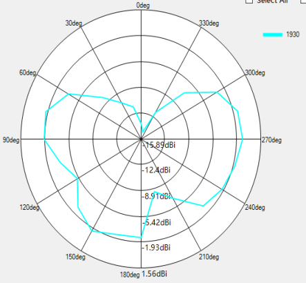
2D Antenna pattern (X->Y;X->Z;Y->Z)
