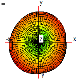
3D Antenna pattern
