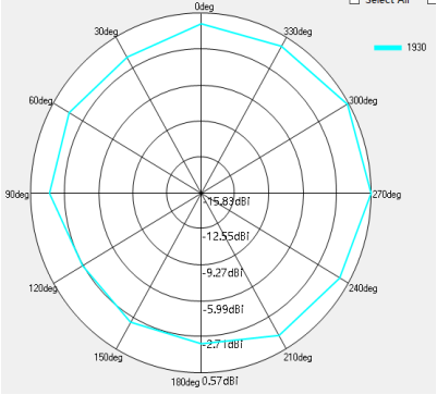
2D Antenna pattern (X->Y;X->Z;Y->Z)
