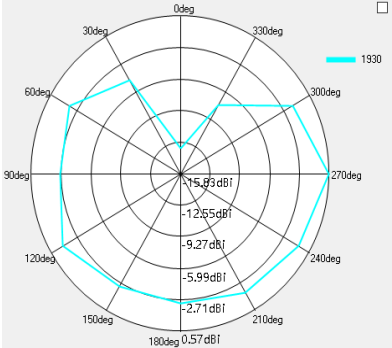
2D Antenna pattern (X->Y;X->Z;Y->Z)
