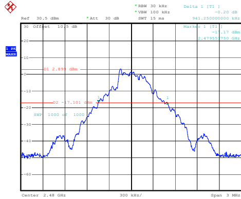
DH1_High 0.941MHz
