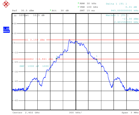
DH1_Low 0.945MHz
