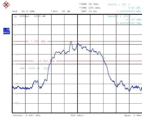
2DH1_Middle 1.230MHz
