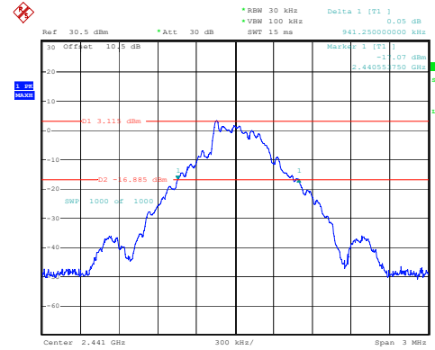
DH1_Middle 0.941MHz
