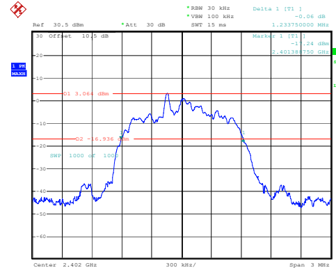
2DH1_Low 1.234MHz
