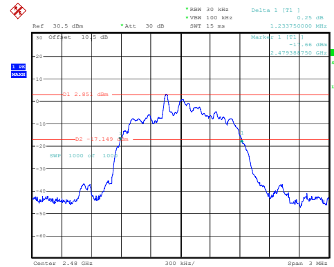
2DH1_High 1.234MHz
