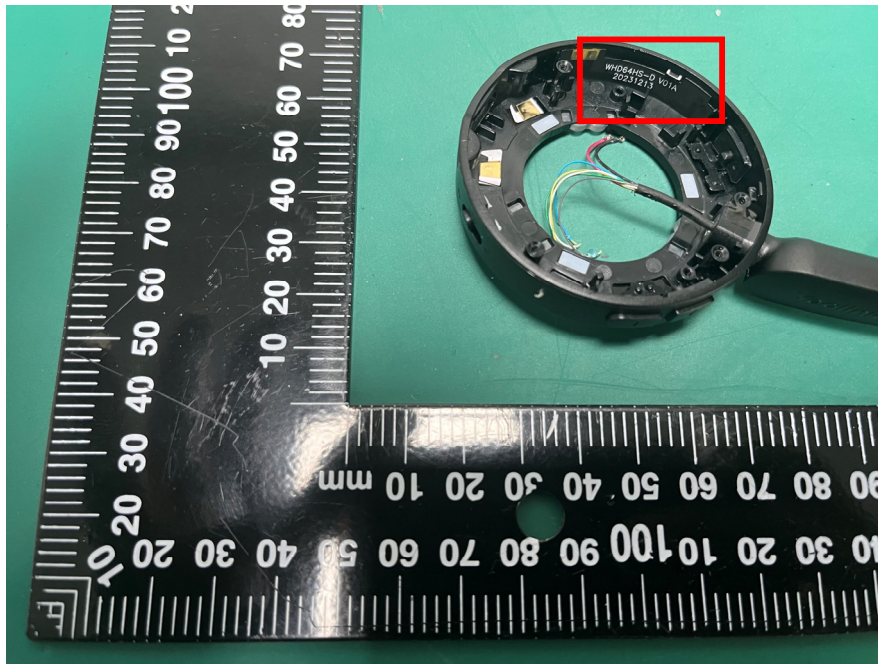
DECT ANT1
