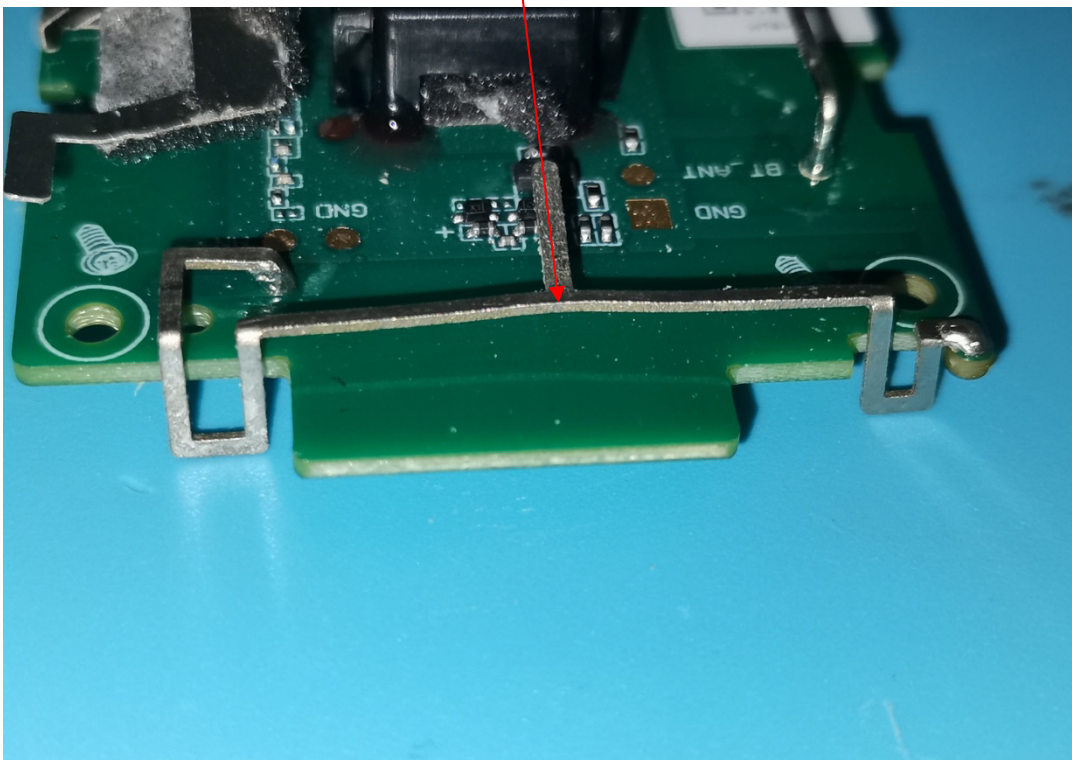
DECT Antenna 2
