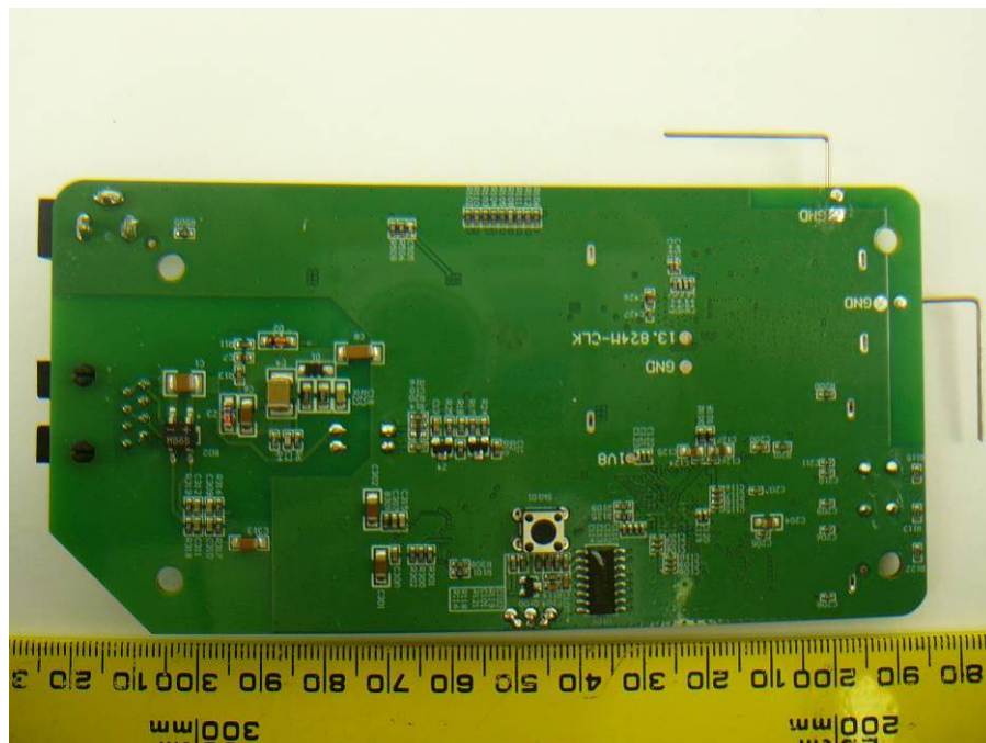
EUT Gateway Main Board without Shielding Bottom View
