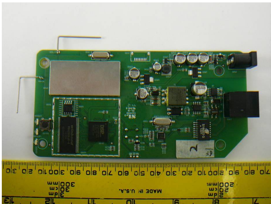
EUT Gateway Main Board with Shielding Top View
