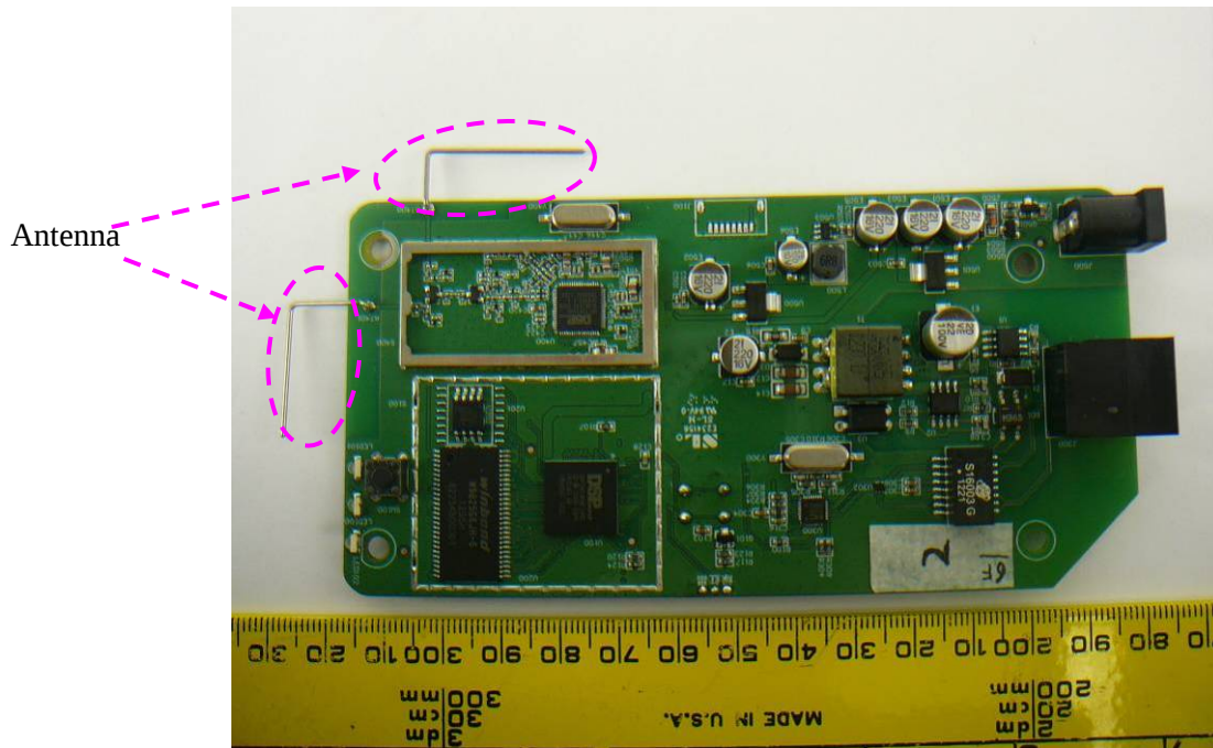
EUT Gateway Main Board without Shielding Top View
