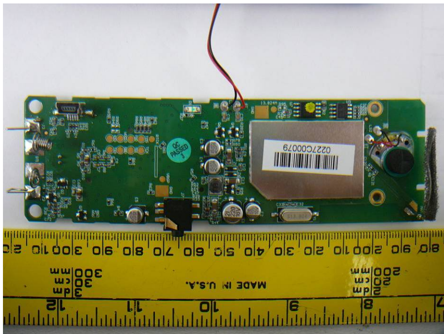
EUT Handset Main Board with Shielding Top View
