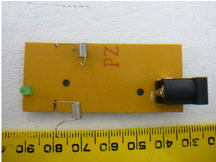
EUT Handset Base/Charger Board Bottom View
