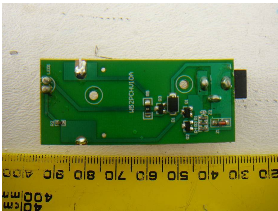
EUT Handset Base/Charger Board Top View
