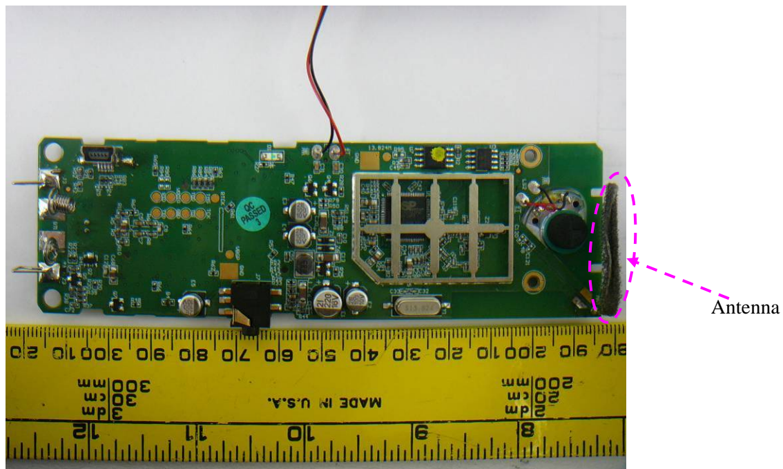
EUT Handset Main Board without Shielding Top View
